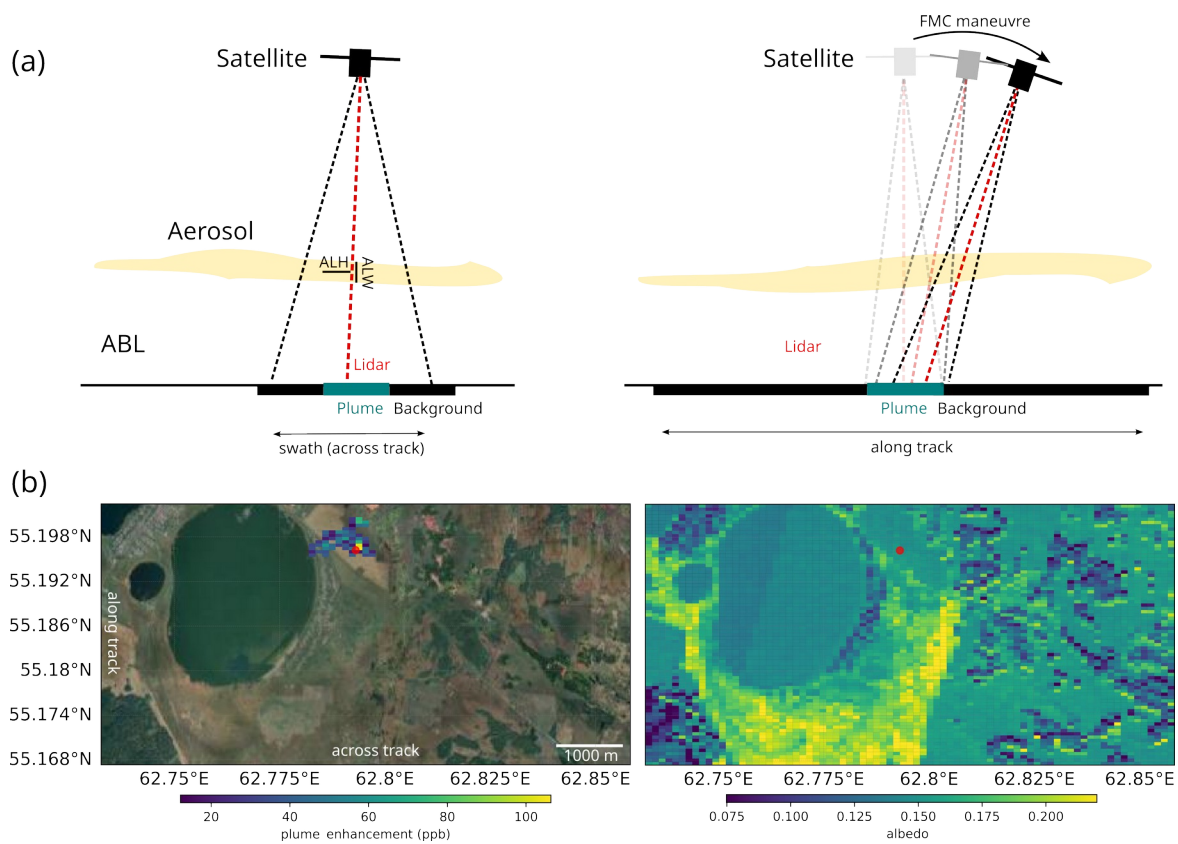
Figure 1. Observation situation. (a) Schematic view of measurement geometry with a staring lidar co-aligned with the push broom spectrometer. In this example the background \text{XCH}_4 is off the center swath, whilst the \text{XCH}_4 enhancement (plume) is at the center of the swath. Left: across track view. ALH and ALW are measured in the swath center. Right: Along track view depicting the forward motion compensation (FMC). ALH and ALW represent average values over the probed track. ABL depicts the atmospheric boundary layer. Figure not to scale. (b)
