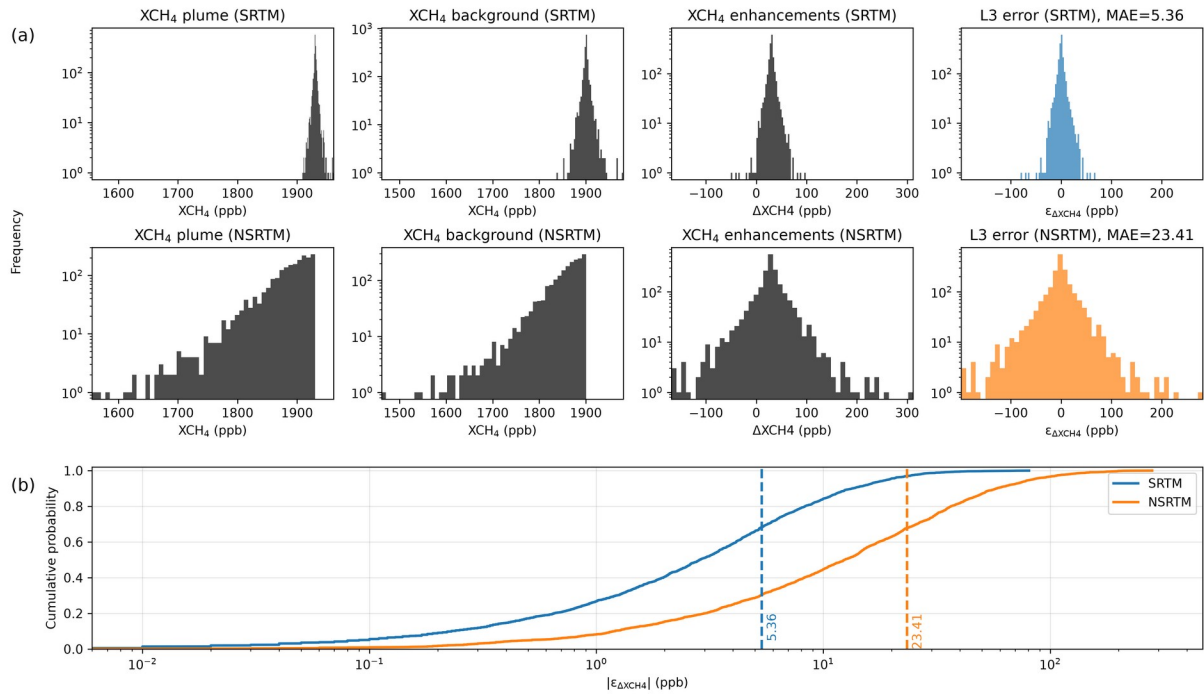
Figure 3. Results for the single central lidar with noise scenario. (a) Histograms of plume and background L2 results, L3 results and L3 bias for the SRTM and NSRTM case. (b) Empirical cumulative distribution of absolute L3 errors for SRTM and NSRTM with MAE depicted.
