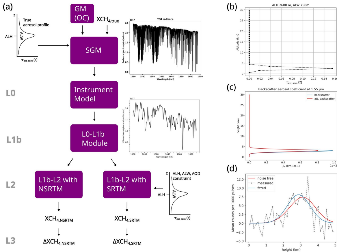
Figure 2. (a) End-to-end simulation scheme (E2E) for a given pixel with geometry module (GM/OC), scene generation module (SGM), instrument module, L0-L1b module, and L1b-L2 module which includes the forward model. Example TOA and L1b spectra are shown. (b) Example discretized AOD profile as used in E2E. (c) Backscatter and attenuated backscatter profile input for lidar simulation. (d)
