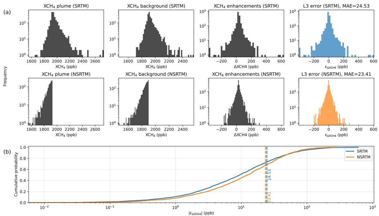
Figure 4. Results for the random guess scenario. (a) Histograms of plume and background L2 results, L3 results and L3 bias for the SRTM and NSRTM case. (b)
