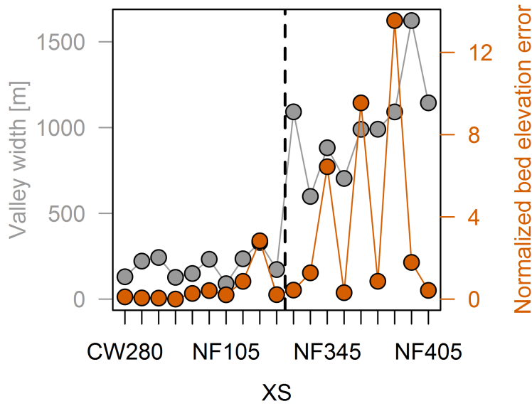
Figure 8: Valley width and error in modeled bed elevation for each cross section in the NFTR (generally shown in order of upstream to downstream). Errors are generally higher where the valley becomes significantly wider.
