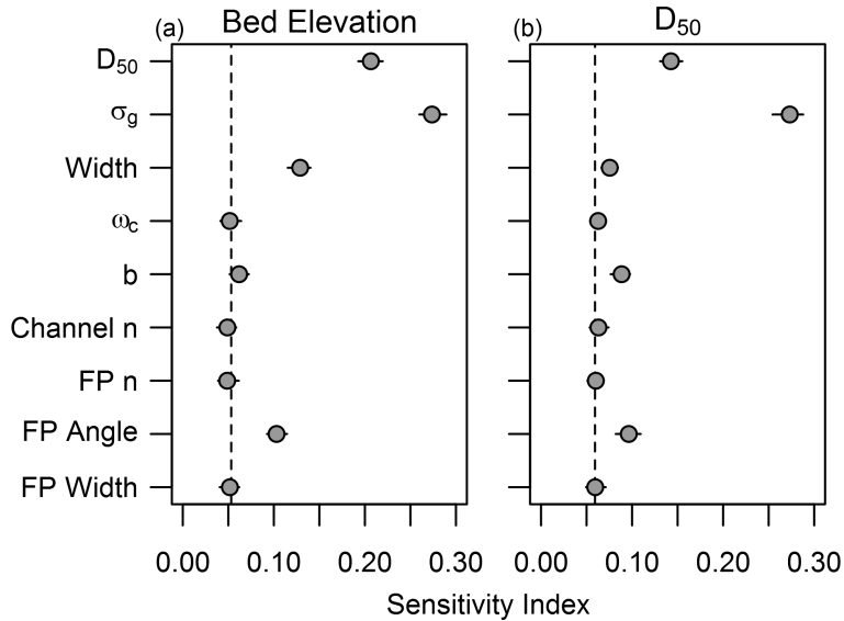
Figure 6: Sensitivity results for the Colorado River for modeled bed elevation (a) and bed D_{50} (b). Points at or below the vertical dashed line had no influence on model output. Points are bias corrected sensitivity indices with ranges estimated from bootstrapping.
