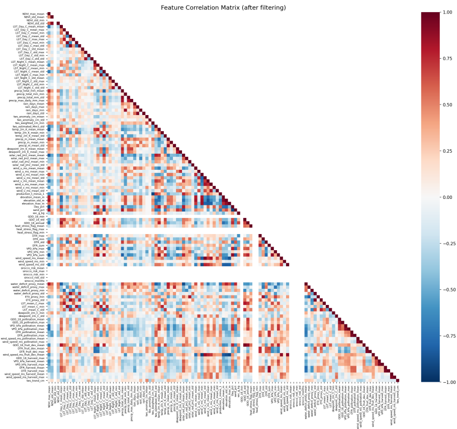
Figure S2: Pairwise Pearson correlation heatmap of the 111-feature predictor set used by the forecasting models. The |r| > 0.95 filter removes the most strongly co-varying pairs.
