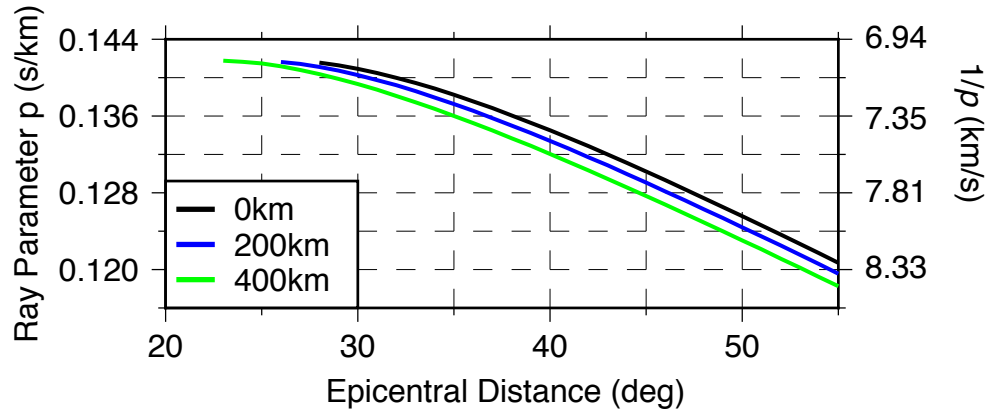
Figure 2. Ray parameters of teleseismic S waves ( S_s ) and corresponding S_sPmp as functions of epicentral distance and focal depth, calculated using the IASP91 model. Note the ray parameter does not exceed 0.143 s/km due to triplication at the bottom of the mantle transition zone.
