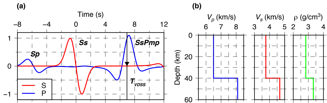
Figure 3. (a): P and S components of the synthetic waveforms computed using the models in (b) and aligned to Ss arrival. Ray parameter of the incident S wave is p = 0.127 s/km ( 1/p=7.87 km/s). The source time function has a dominant frequency of \sim 0.25 Hz. The Ss arrival is picked at the zero-crossing of the source wavelet, the peak of the envelope function. Black inverted triangle: SsPmp arrival time relative to Ss ( T_{VDSS} ) predicted with ray theory. Large amplitude and phase shift of SsPmp are due to post-critical reflection at the Moho. (b): 1D velocity and density model of a homogeneous crust over a half-space mantle that are used to compute waveforms in (a).
