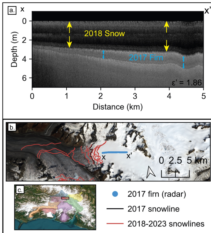
Fig. 9. (a) 2018 airborne radar data on the Logan Glacier prominently shows the 2017 firn layer thinning and disappearing near the (b) 2017 end-of-summer snow line. The radargram is read from x to x' in (b). Radargram is flattened so that the surface is at zero depth. Background is a Landsat 8 image acquired on August 6, 2017. (c) Context map for panel b using the same color shading as in Fig. 1. Subset of (b) is the black box.
