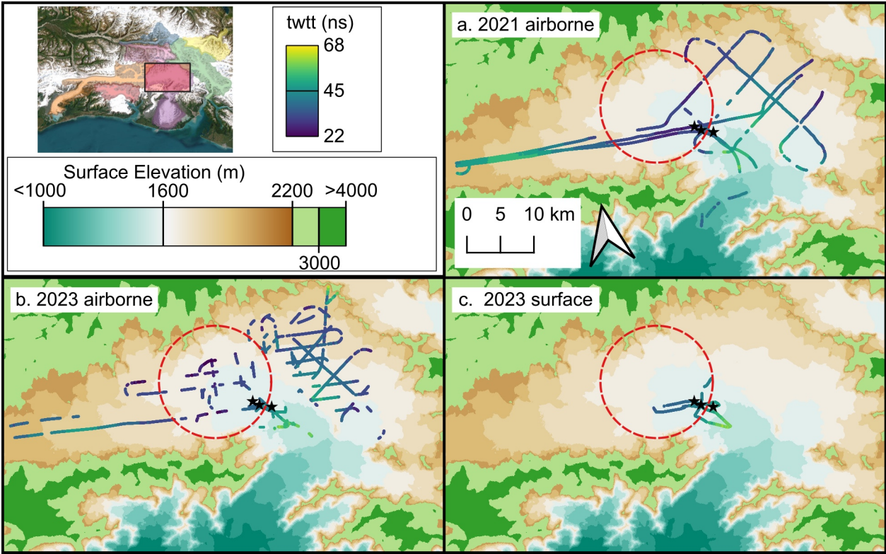
Fig. 12. Two-way travel times to the last summer surface on the Seward Glacier for the (a) 2021 and (b) 2023 airborne radar data, in addition to the (c) surface GPR data. To emphasize the 1000–2200 m elevation range, the Copernicus GLO-30 DEM background uses discrete steps of 100 m between 1000–2200 m, with single colors for 2200–3000 m and >3000 m. The three pit sites from 2023 are marked by black stars.
