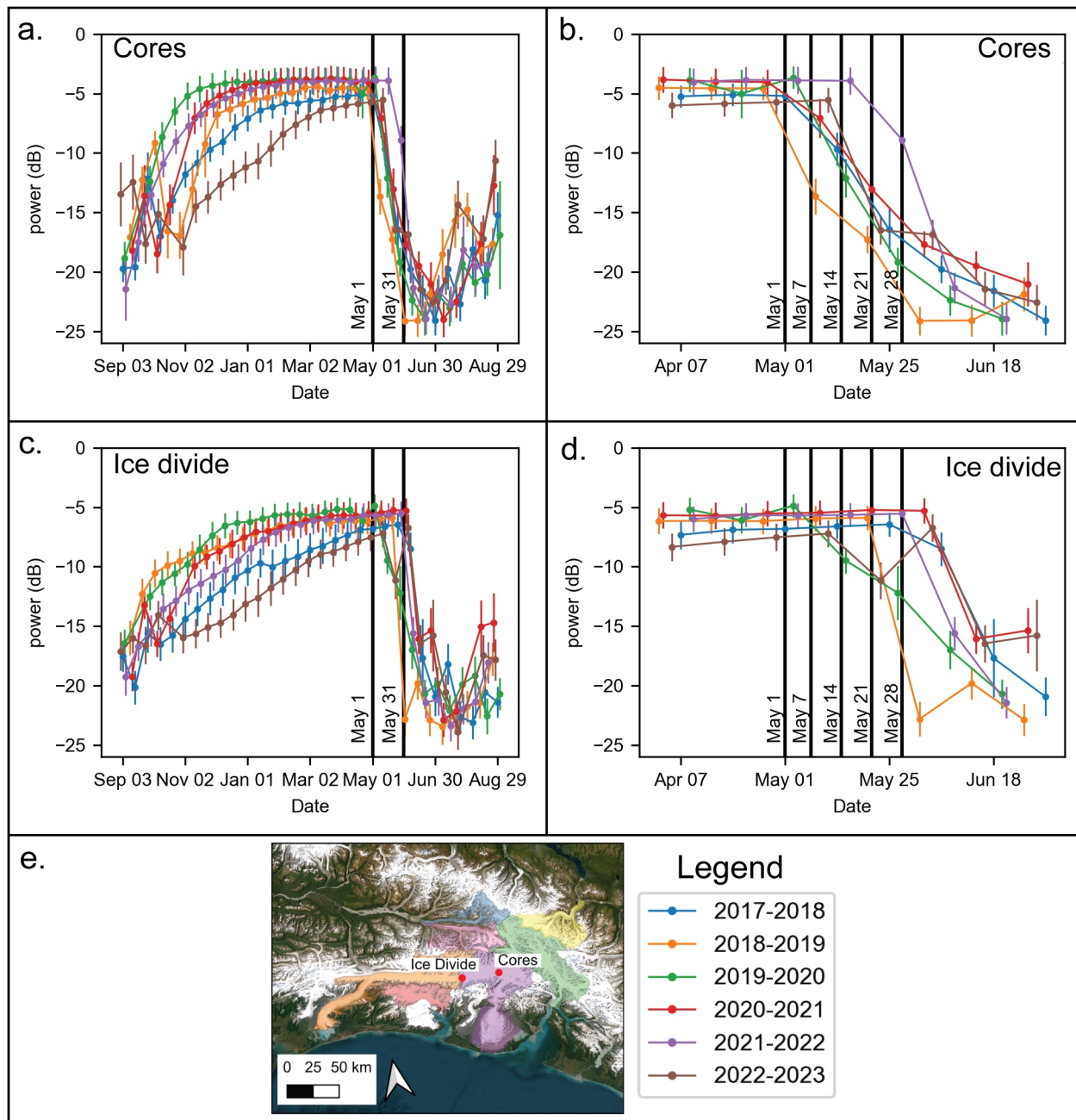
Fig. 10. Sentinel 1 reflectivity over six water years for the (a) 2023 Seward core sites at ~1600 m a.s.l. and (b) subset from April 1 to June 30. Same period for the (c) Seward-Bering ice divide at ~2000 m a.s.l. and (d) subset from April 1 to June 30. Error bars are single standard deviation of the power in the sampling area. Vertical lines are labeled with context dates for improved understanding of the time series around May. (e) Context map of the location of the two Sentinel 1 sample sites and the water year color legend.
