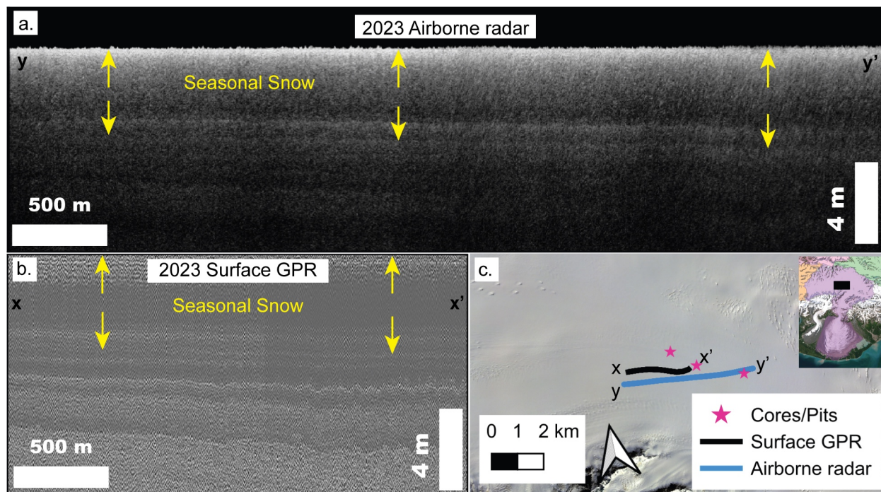
Fig. 3. Sample radargrams for (a) airborne radar and (b) surface GPR from the Seward Glacier near the 2023 core sites. (c) Paths for each of the radargrams with the inset showing the Seward Glacier and the extent of panel (c) marked by the black box. Both radargrams are read left to right from x/y to x'/y' as marked in (c). The yellow arrows mark the seasonal snow layer. A layer is present above what we mark as the last summer surface in both. Based on context from the nearby cores, the reflector marked by the yellow arrows is a better fit for the last summer surface depth than the shallower reflector (Section 3.1.3). The layer above the last summer surface reflector may be related to a surface-wetting event in Fall 2022. Both radargrams are flattened so that the surface is at zero depth.
