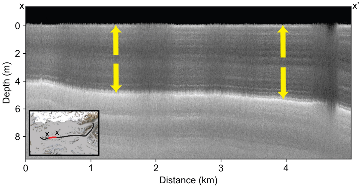
Fig. 11. Sample radargram from 2023 on the center arm of the Kaskawulsh Glacier with the extent of the inset box being the same as the inset in Fig. 4d. Radargram surface elevation was ~2700 m a.s.l. In the inset we include the path of the radargram in Fig. 4 as the black line, while this radargram is the red section. The radargram is flattened so that the surface is at zero depth and is read from x to x'.
