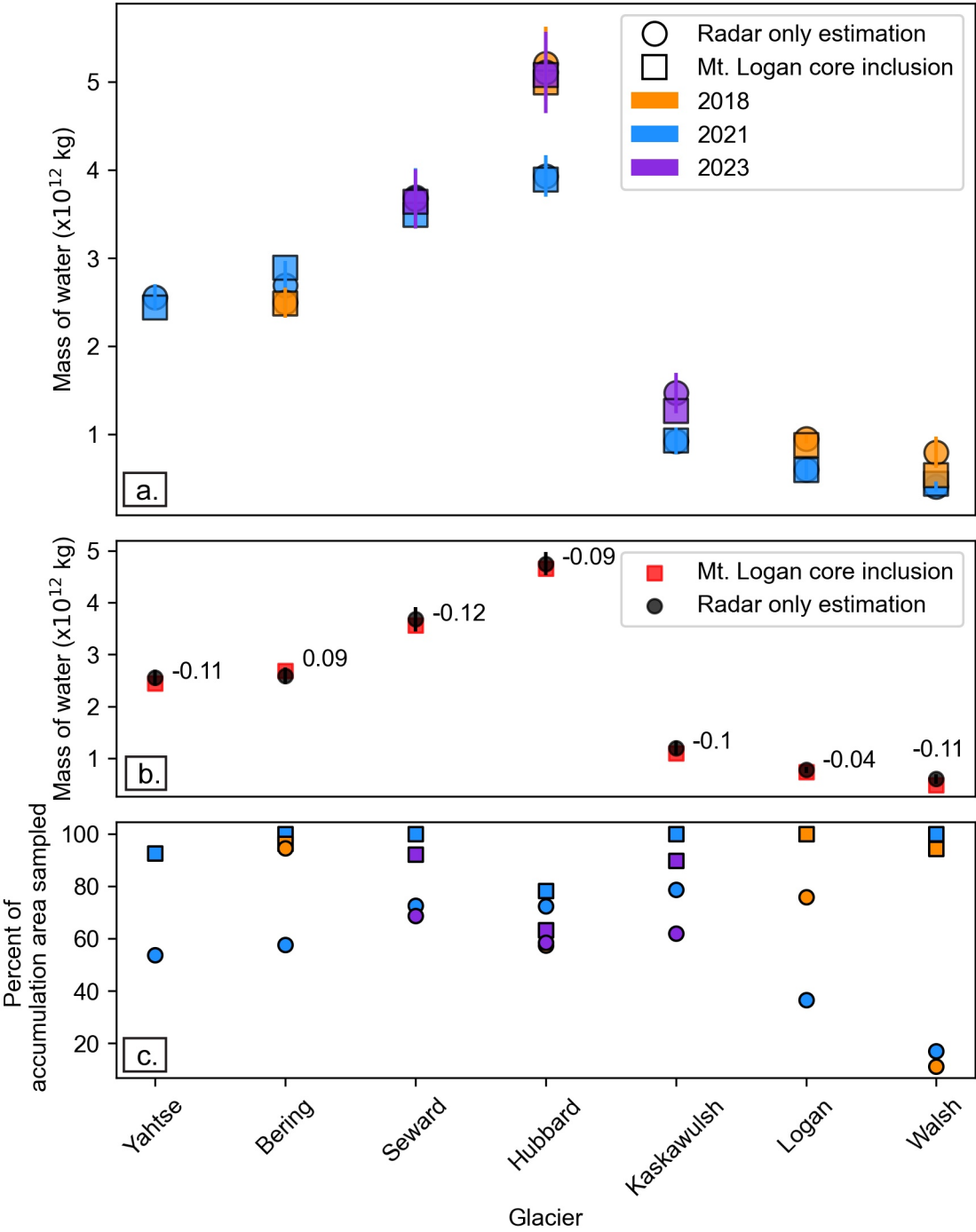
Fig. 8. (a) Winter accumulation area mass input in mass of water for each glacier by survey year. (b) The mean value from (a) per glacier with the difference between the two methods reported by the numbers on the plot in units of 10^{12} kg. The mean estimates that include the interpolation to the Mt. Logan core record lie within the uncertainty of the radar only estimation for all seven glaciers. Values are reported in Table S3. (c) The corresponding percent of the accumulation area sampled. Glaciers are ordered roughly by their distance from the coast, closer (left) to further (right). The percent of the accumulation area sampled is the sum of the areas for each hypsometry elevation range that contains radar-derived SWE values divided by the glacier area above our defined ELAs. For the Mt. Logan core inclusion estimation, the percent of accumulation area sampled includes the glacier area above the highest surface elevation with radar data.
