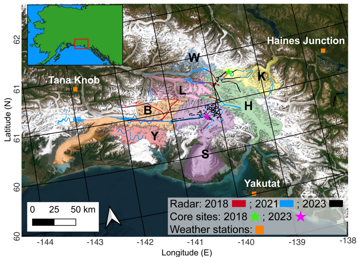
Fig. 1. Airborne radar data coverage, in situ measurement locations, and long-term weather station locations for our study. Glacier outlines are from the Randolph Glacier Inventory v7 (RGI Consortium, 2023). Glaciers are labeled by their first letter; B: Bering, H: Hubbard, K: Kaskawulsh, L: Logan, S: Seward, W: Walsh, and Y: Yahtse. The 2018 core site (green) is from Ochwat and others (2021) and the 2023 core site (magenta) is from our field measurements. This map, and all others in this work, are projected to NAD83/Alaska Albers EPSG:3338.
