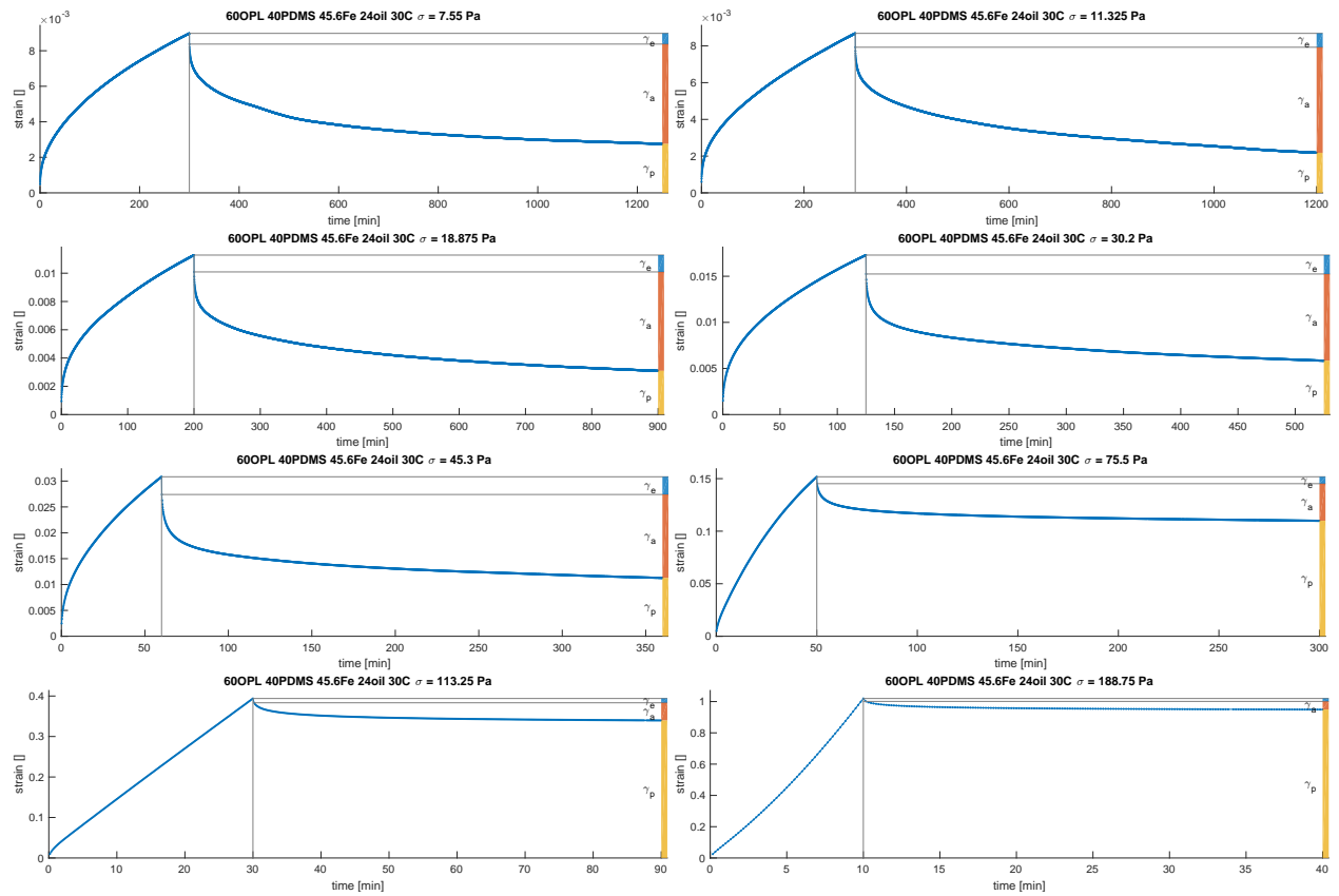
Figure 20: Strain during loading and relaxation for 60 OPL 40 PDMS 24 oil @ T = 30^\circ \text{C} at each stress level, with elastic strain \gamma_e , anelastic strain \gamma_a and permanent strain \gamma_p . Permanent strain is used to compute the mean strain rate and steady-state viscosity \bar{\eta} (equation (20)).
