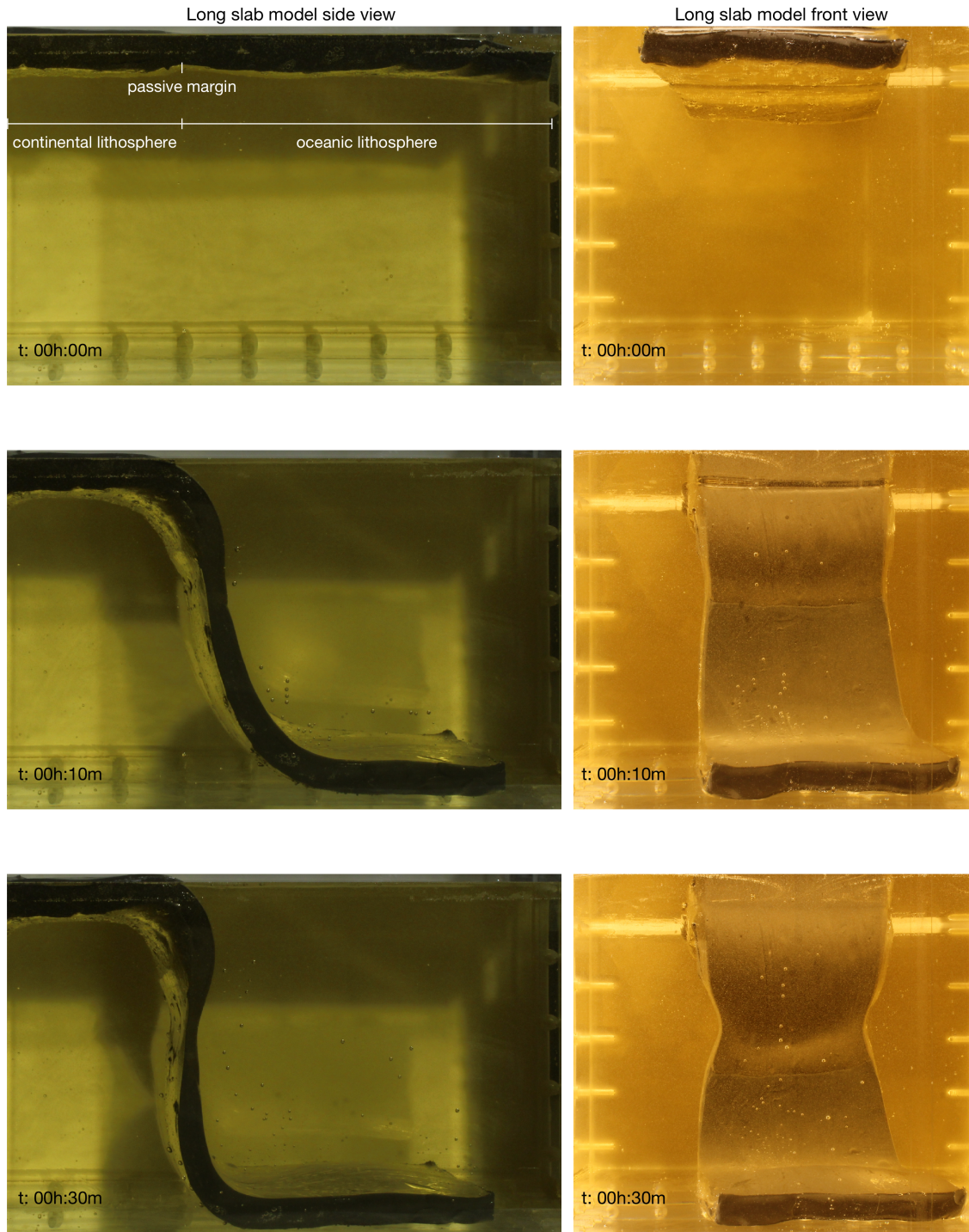
Figure 11: Snapshots of side and frontal views of the long slab model. The location of the continental and oceanic lithospheric units, as well as the passive margin are depicted in the upper panels.
