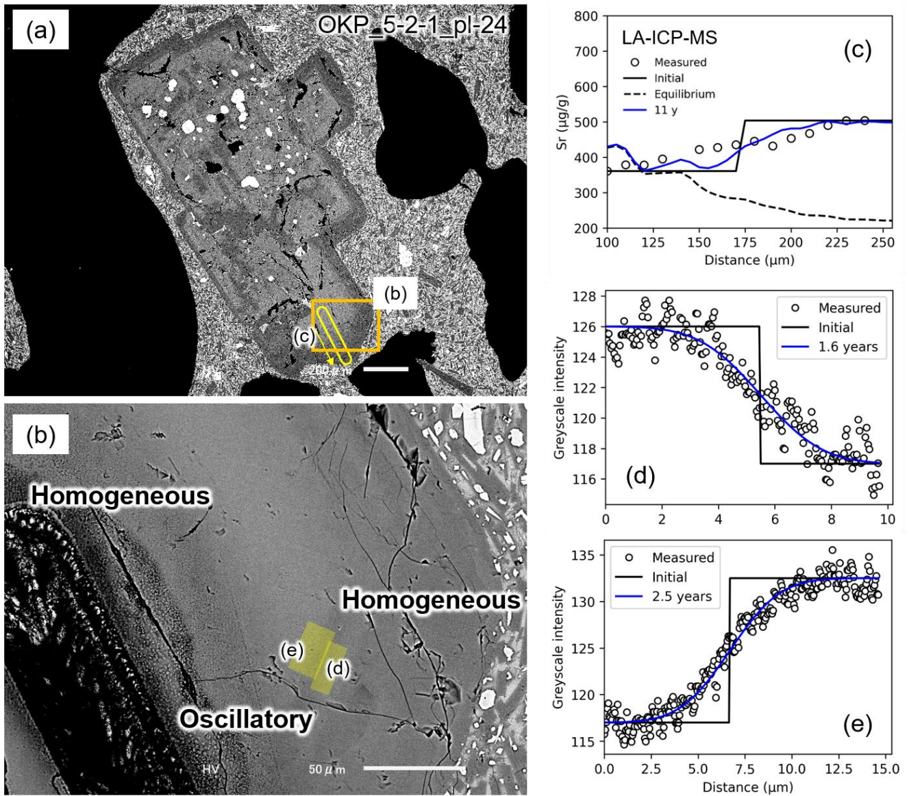
Figure 7: Modelling examples of Sr diffusion and CaAl-NaSi interdiffusion in plagioclase crystals (Type D, honeycomb core + homogeneous mantle + homogeneous rim). (a) Back-scattered electron (BSE) image, (b) magnified image, (c) Sr profile, and (d-e) greyscale intensity (white circles), initial (black lines) and best-fit diffusion (blue lines) profiles.
