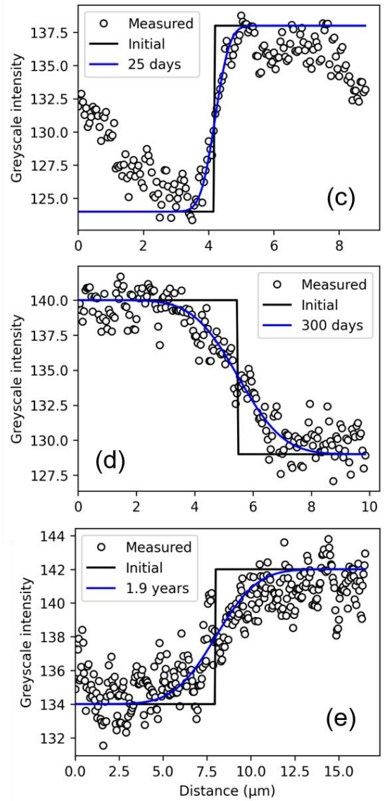
Figure 3: Modelling examples of CaAl-NaSi interdiffusion in plagioclase crystals (Type B, patchy core + oscillatory-zoned mantle + homogeneous rim). (a) Back-scattered electron (BSE) image, (b) magnified image, and (c–e) greyscale intensity (white circles), initial (black lines) and best-fit diffusion (blue lines) profiles.
