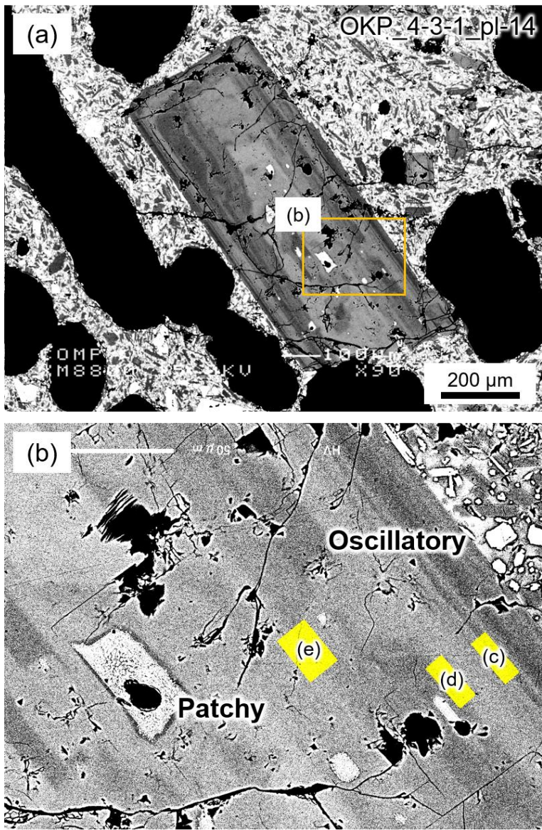
Figure 3: Modelling examples of CaAl-NaSi interdiffusion in plagioclase crystals (Type B, patchy core + oscillatory-zoned mantle + homogeneous rim). (a) Back-scattered electron (BSE) image, (b) magnified image, and (c–e) greyscale intensity (white circles), initial (black lines) and best-fit diffusion (blue lines) profiles.
