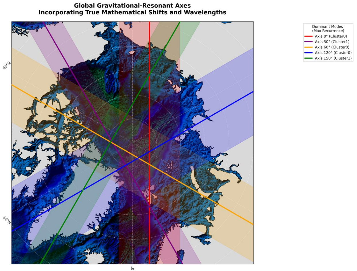
Figure 3: Five main transarctic gravitational-resonant axes of ice compression. Axis N^\circ is the geographic meridian of the wave front (Axis 0^\circ through Fram Strait). The axes are strictly anchored to bottom topography (background: IBCAO bathymetry). (Note: The Python script for this data visualization was generated with the assistance of Cursor AI).
