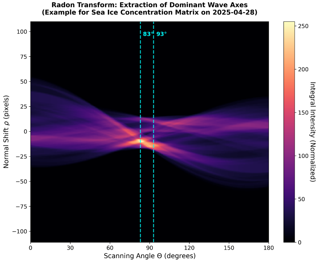
Figure 1: Example of the Radon Transform. Maxima of integral intensity indicate scanning angles \Theta corresponding to the dominant axes of kinematic compression in the sea ice cover. (Note: The Python script for this data visualization was generated with the assistance of Cursor AI).
