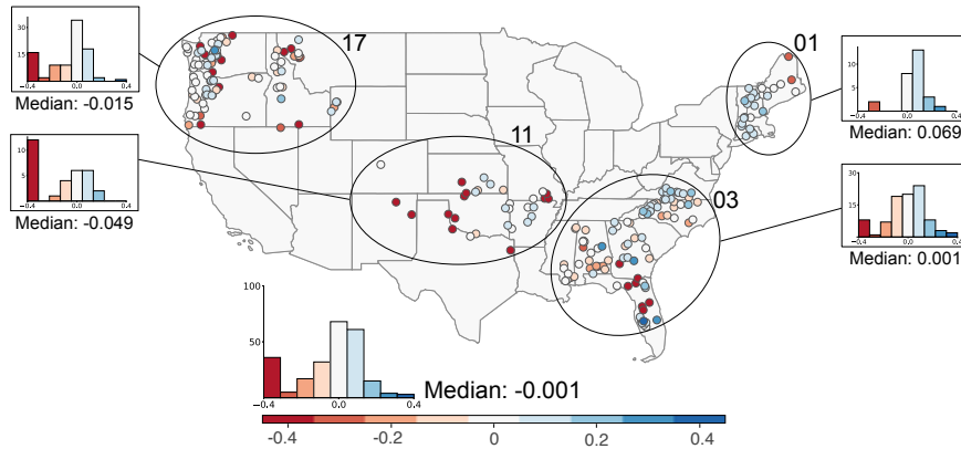
Figure 9. Difference of the regional model compared to the models from Experiment 1 for each basin regarding the NSE of the validation period. Blue colors ( > 0 ) mean the regional model performed better than the models from Experiment 1, red ( < 0 ) the other way around.
