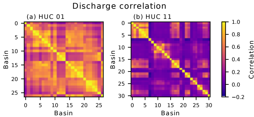
Figure 11. Correlation matrices of the observed discharge of all basins in a) HUC 01 and b) HUC 11.
