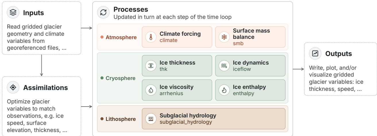
Figure 4. Overview of the IGM modular architecture: Gridded glacier geometry and climate variables are read from georeferenced files in “input” modules and optionally adjusted in “assimilation” modules to match observations (e.g., ice surface speed, surface elevation, thickness). A configurable chain of “process” modules—color-coded by earth-system component—is then evaluated; each box gives the process name and its module identifier (e.g., smb , thk , iceflow ). Results are written, plotted, or visualized as gridded glacier variables in “output” modules.
