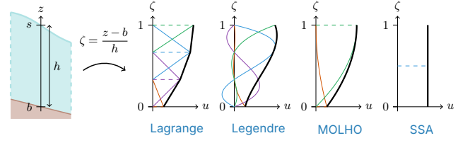
Figure 2. Vertical discretization schematic. The terrain-following coordinate \zeta = (z - b)/h maps the ice column to [0, 1] . Four vertical basis types are shown: Lagrange (piecewise linear polynomial interpolation), Legendre (polynomial expansion; Shapero et al., 2021), MOLHO (SIA profile; Dias dos Santos et al., 2022), and SSA.
