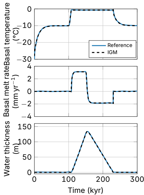
Figure D2. Experiment A of Kleiner et al. (2015). Reference corresponds to the numerical solutions shown in Kleiner et al. (2015).
