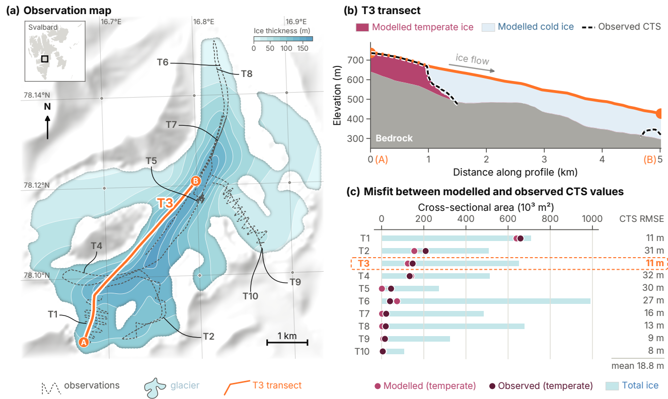
Figure 8. Calibration of the thermal structure of Drønbreen, Svalbard, against the CTS observed along ten GPR transects (Mannerfelt et al., 2025). (a) Ice thickness of the fixed model geometry with the ten radar tracks T1–T10 (dashed) and the featured transect T3 (orange), whose upper and lower ends are marked A and B; inset: location on Svalbard. (b) Modeled temperate (magenta) and cold (light blue) ice along T3 for the best trial, drawn from A to B so that ice flows left to right; the modeled CTS is the boundary between the two fills, and the dashed black line is the observed CTS. Where the observed CTS runs through cold (temperate) ice, the model produces too little (too much) temperate ice. (c) Cross-sectional area of temperate ice observed (dark purple) and modeled (magenta) along each transect, on light-blue bars giving the total ice cross-section; T3 is framed. The column on the right gives the per-transect RMSE of the modeled CTS elevation, whose mean of 18.8 m is the Optuna objective.
