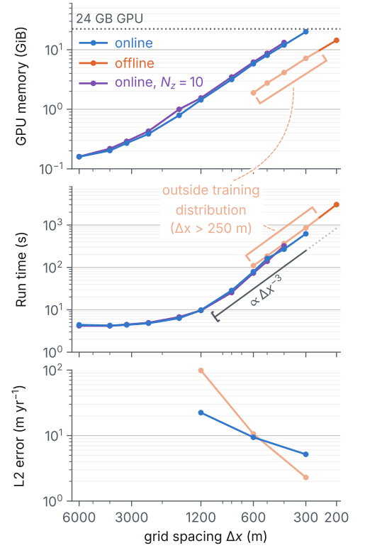
Figure 7. Scalability of IGM on one GPU for a 500-year simulation of a glaciation onset in the Alps. (a) Modelled surface ice speed after 500 years at \Delta x = 200 m over a 192 \times 188 km part of the domain; top-left inset: whole 900 \times 600 km model domain with the extent of the map (red box); circle: close-up magnified \times 4 . (b) Peak GPU memory (top), run time (middle; ice-flow solver time over the whole simulation) and L^2 error of the depth-averaged ice speed after 500 years against a reference solution on a 160 \times 134 km sub-domain (bottom) versus grid spacing \Delta x , online (small network retrained at every time step) and offline (large pretrained network), both with MOLHO ( N_z = 2 ), and online with a Lagrange basis ( N_z = 10 ; cost and memory only). The online runs do not fit in memory at 200 m ( N_z = 2 ) and below 400 m ( N_z = 10 ). Faded: offline outside its 50–250 m training distribution. Grey line: \Delta x^{-3} , from where this regime starts (bracket). Dotted line: memory of the 24 GB GPU.
