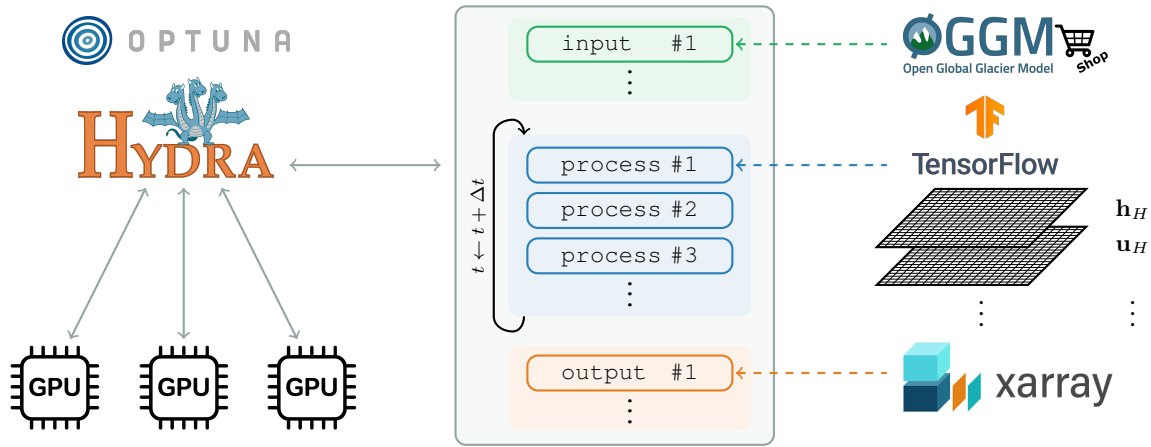
Figure 5. Schematic of the IGM software architecture. Simulations are assembled from input, assimilation, process, and output modules selected in a YAML configuration file. Input components populate the model state from local files or external glacier data sources; process components update state variables on a raster grid during the time loop; and output components write fields, diagnostics, or visualizations. Internally, spatial fields are represented as TensorFlow tensors, while file-based input and output are handled through Xarray.
