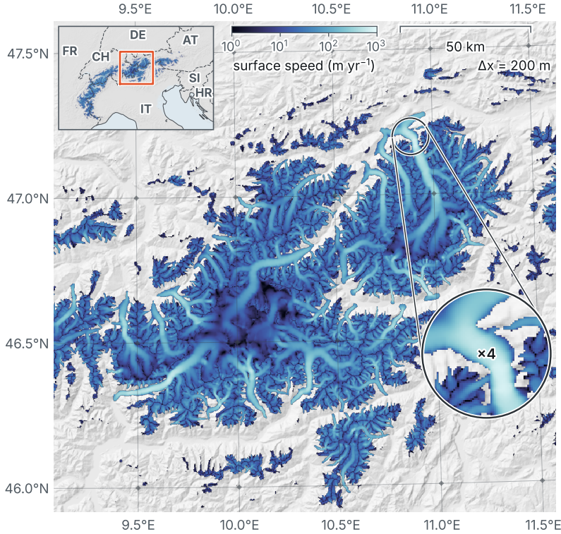
Figure 7. Scalability of IGM on one GPU for a 500-year simulation of a glaciation onset in the Alps. (a) Modelled surface ice speed after 500 years at \Delta x = 200 m over a 192 \times 188 km part of the domain; top-left inset: whole 900 \times 600 km model domain with the extent of the map (red box); circle: close-up magnified \times 4 . (b) Peak GPU memory (top), run time (middle; ice-flow solver time over the whole simulation) and L^2 error of the depth-averaged ice speed after 500 years against a reference solution on a 160 \times 134 km sub-domain (bottom) versus grid spacing \Delta x , online (small network retrained at every time step) and offline (large pretrained network), both with MOLHO ( N_z = 2 ), and online with a Lagrange basis ( N_z = 10 ; cost and memory only). The online runs do not fit in memory at 200 m ( N_z = 2 ) and below 400 m ( N_z = 10 ). Faded: offline outside its 50–250 m training distribution. Grey line: \Delta x^{-3} , from where this regime starts (bracket). Dotted line: memory of the 24 GB GPU.
