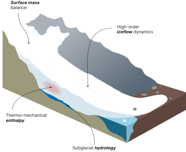
Figure 1. Overview of IGM, with a schematic of a glacier showing the coupled physical processes (left) and the framework’s design principles (right) that together enable efficient glacier evolution simulations.
