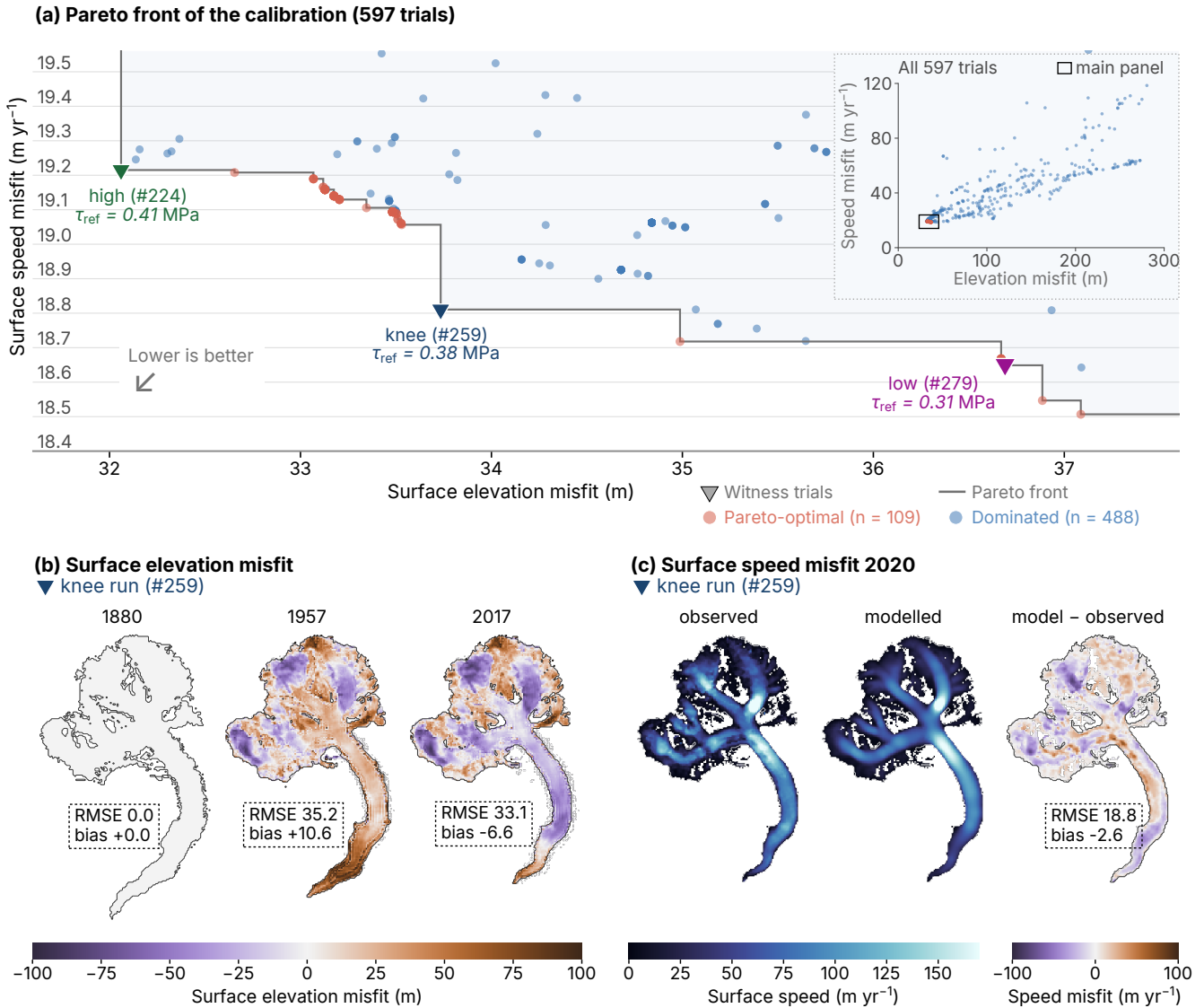
Figure 6. Calibration of Aletsch Glacier from 1880 to 2020 with a \sim 600 -trial NSGA-II sweep. (a) Pareto front, zoomed on its extent: dominated trials (blue) and Pareto-optimal trials (red) are semi-transparent, so that repeated parameter sets appear darker; the gray staircase is the Pareto front and the shading marks the region it dominates. The triangles mark three witness trials: the knee, and the Pareto-optimal trials with the lowest and highest basal shear stress \tau_{\text{ref}} . The inset shows all trials over their full range, with the extent of the main panel outlined. (b) Modeled – observed surface elevation of the knee run at three DEM dates (1880 being the initial state), over the union of the modeled and observed ice extents; the black line is the modeled ice margin. (c) Observed and modeled surface speed in 2020, and their difference, over all observed pixels. The dashed boxes give the RMSE and mean bias of each misfit map.
