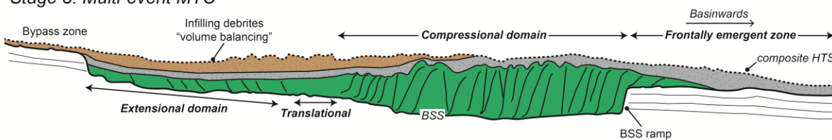
42 Figure 8: MTC emplacement models, Model 1: Shear coupling mechanism, stage 1 initiation through 43 overriding debris flow producing localisation of shear stress on a mechanically weak likely shallow 44 gas filled zone, stage 2 in situ failure of underlying sediments through shear coupling, stage 3 failure 45 of underlying sediments has produced significant extensional and compressional domains in the final 46 deposit, Model 2: Loading mechanism, stage 1 initiation through loading and progressive downslope 47 failure, stage 2 infilling of remnant topography by later debris flow(s), stage 3 failure from a loading 48 mechanism has produced similar extensional and compressional domains to Model 1.
