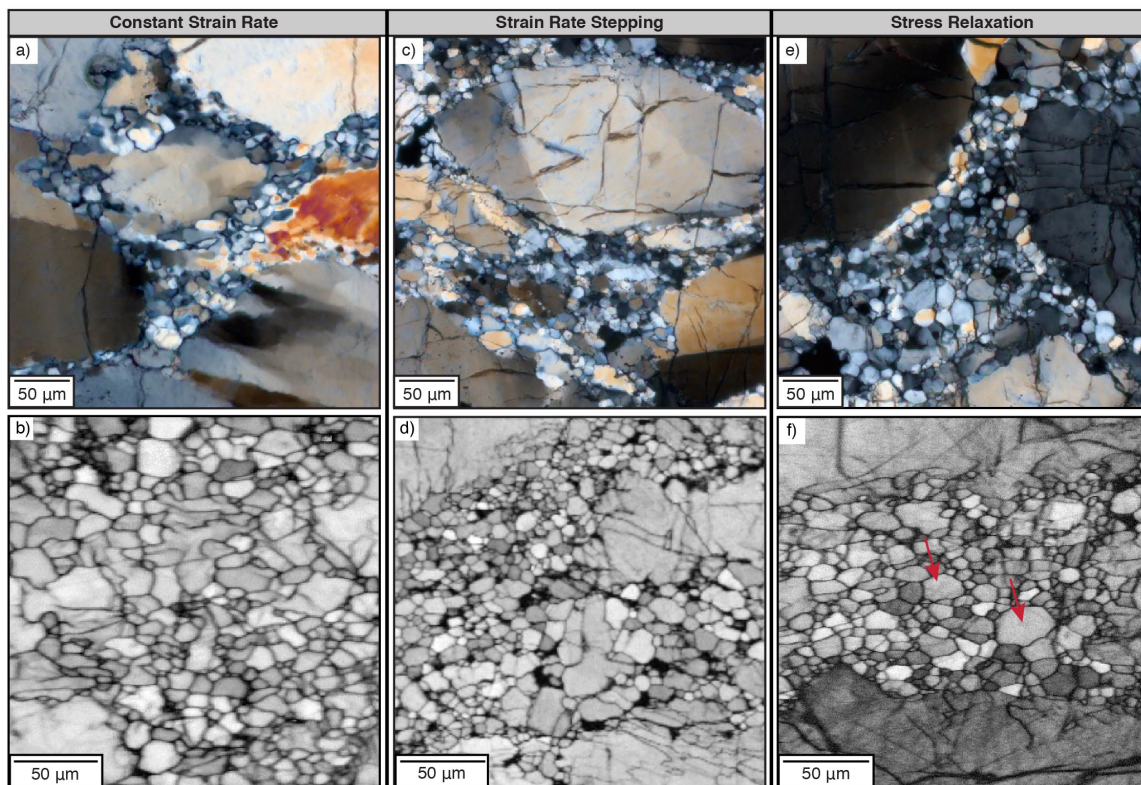
Figure 6. Representative cross-polarized micrographs for each type of experiment, and EBSD band contrast maps of different regions within the same samples. a and b) Constant strain rate (w1990, peak stress = 323 MPa), c and d) rate-stepping (w2002, 558 MPa), e and f) stress relaxation (w1964, 399 MPa); larger grains are convex inward adjacent to smaller grains (red arrows in f). Dark regions are plucked grains. Shortening direction is vertical.
