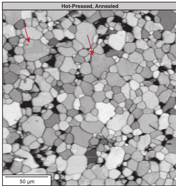
Figure 7. EBSD band contrast map of hot-pressed annealed Balsam Gap dunitite (w2084BG). Larger grains tend to have more than six sides and are convex inward on at least one boundary, adjacent to convex-out grains with fewer grain boundaries (red arrows). Dark regions are plucked grains.
