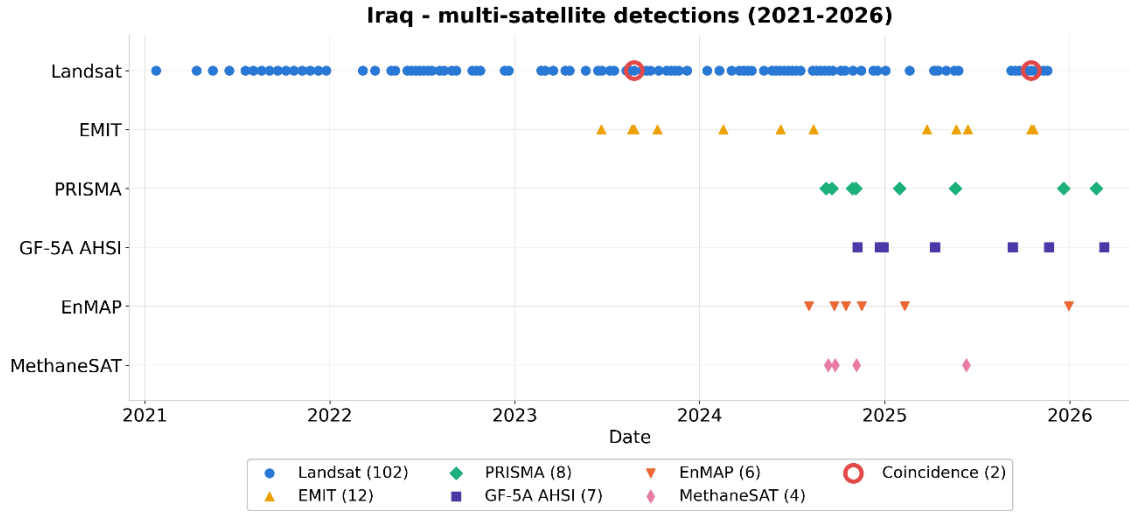
Figure S8. Temporal comparison between Landsat \text{NH}_3 plume detections and hyperspectral observations at the Iraq fertilizer plant (Khor Al-Zubair; 30.185, 47.838) reported by Roger et al. (2026). Landsat detection days over 2021–2025 are shown together with the acquisition dates of the hyperspectral imaging spectrometers (EMIT, EnMAP, PRISMA, Gaofen-5A, and MethaneSAT). Among all the hyperspectral acquisitions, only EMIT (25 August 2023 and 17 October 2025) coincides with a Landsat overpass on the same day.
