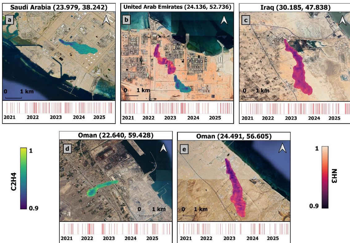
Figure 2. Landsat \text{NH}_3 and \text{C}_2\text{H}_4 plumes at the five focus facilities, with their detection time series represented by each red vertical line. Each panel shows a Landsat band-ratio plume overlaid on a Google Satellite basemap, with the 2021-2025 detection time series (red marks indicating days with a detected plume) below: (a) the Saudi Arabia petrochemical plant (23.979, 38.242), 2023-09-28; (b) the UAE fertilizer-petrochemical complex (24.136, 52.736), 2023-03-22; (c) the Iraq fertilizer plant (30.185, 47.838), 2023-09-10; (d) the Oman fertilizer plant (22.640, 59.428), 2024-08-26; (e) the Oman petrochemical plant (24.491, 56.605), 2025-04-25. \text{C}_2\text{H}_4 plumes follow the green color scale, and \text{NH}_3 plumes the red scale.
