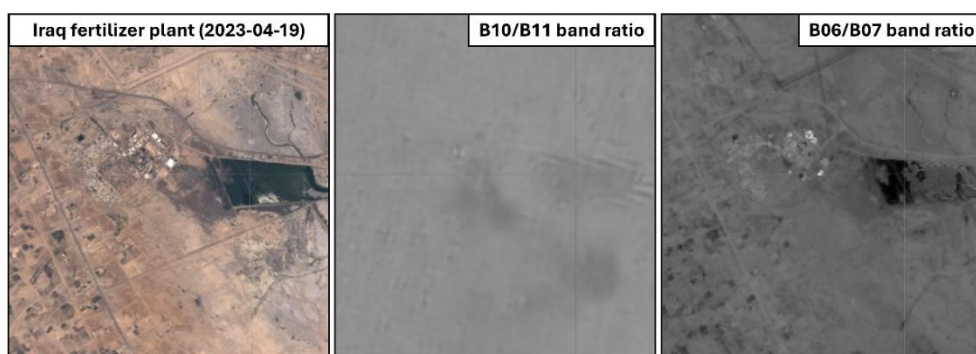
Figure S27. Comparison of thermal- and shortwave-infrared detection at the Iraq fertilizer plant (2023-04-19). Left: Landsat true-color (RGB) reference image of the facility. Center: the B10/B11 thermal-infrared band ratio, in which the \text{NH}_3 plume appears as a diffuse dark enhancement extending from the source. Right: the B06/B07 shortwave-infrared band ratio, which shows only surface features and no detectable plume.
