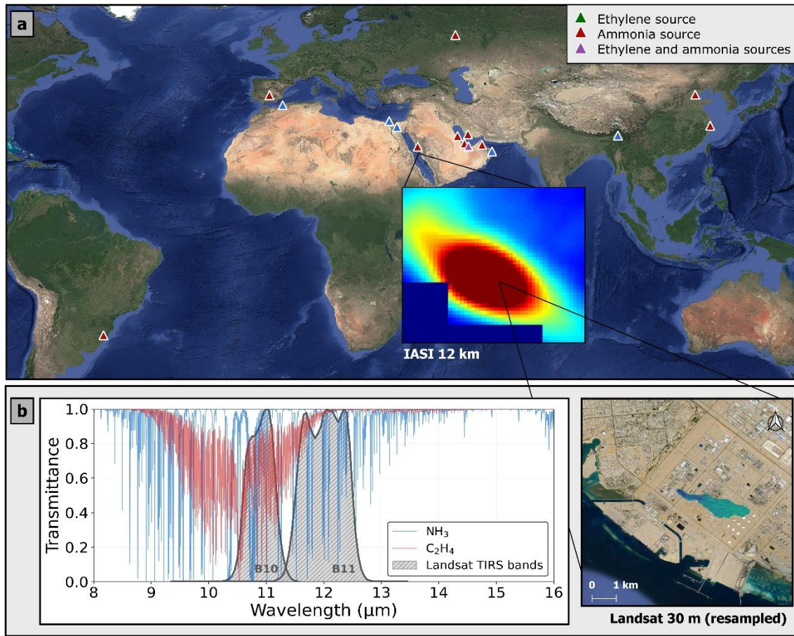
Figure 1. Industrial \text{NH}_3 and \text{C}_2\text{H}_4 point sources and the spectral basis for their detection with Landsat. (a) Global distribution of the facilities where Landsat detected at least one plume over 2021–2025, coloured
