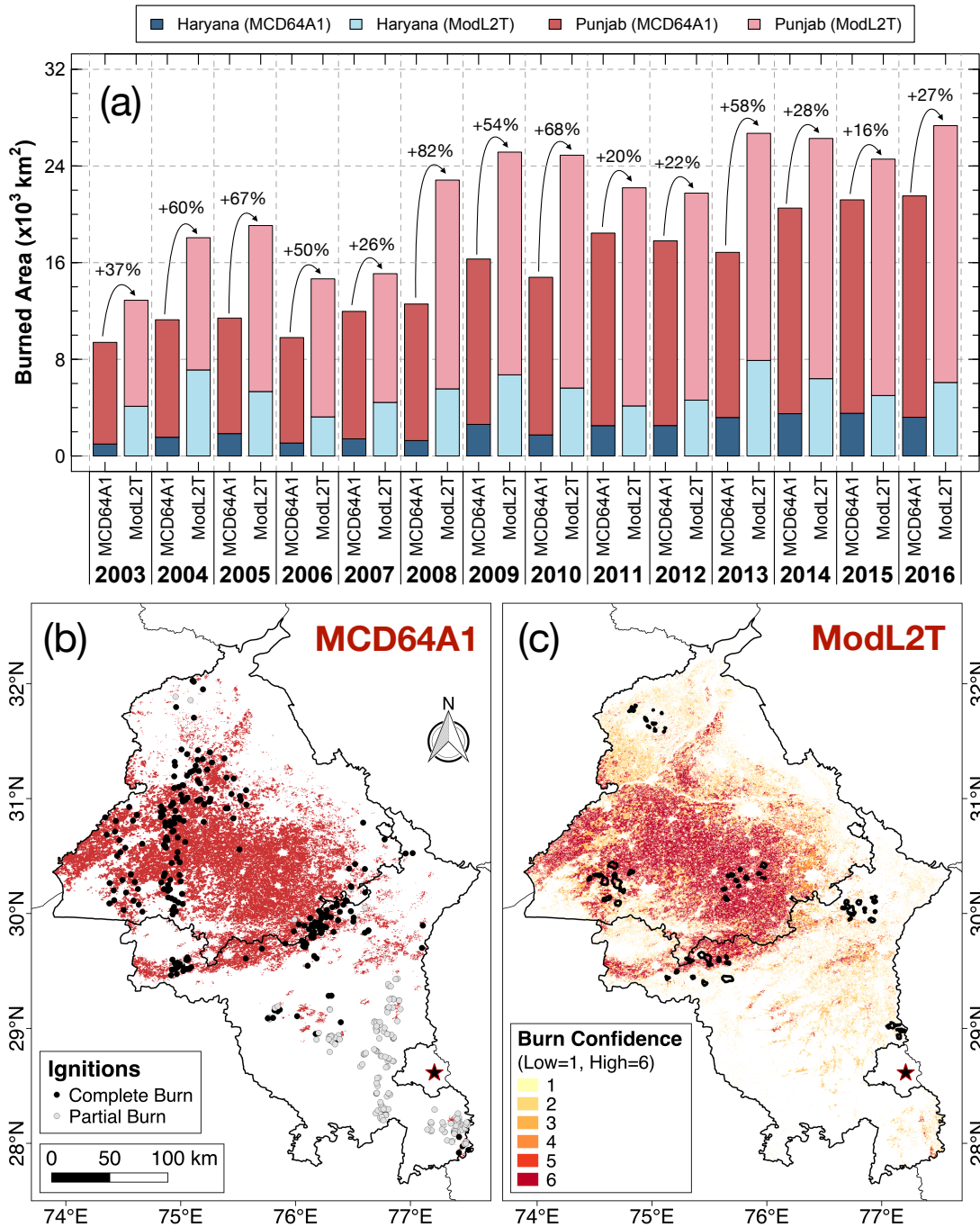
Figure 3. MCD64A1 and ModL2T burned area: (a) BA_{MCD64A1} and BA_{ModL2T} in Punjab (red shades) and Haryana (blue shades) during post-monsoon (Oct-Nov), 2003-2016. The ModL2T algorithm estimates 44 \pm 21\% higher post-monsoon burned area in Punjab and Haryana than MCD64A1. The curved arrows denote the relative boost in burned area mapped by ModL2T compared to MCD64A1. (b) BA_{MCD64A1} and (c) classification confidence (Low = 1, High = 6) for BA_{ModL2T} in Haryana and Punjab, post-monsoon (October-November) in 2016. Ignitions identified from fine-resolution imagery, from 2010-2016 are denoted as black (complete burns) and gray (partial burns) circles in (b). The locations of the villages surveyed in Punjab and Haryana in 2016 are shown as black polygons in (c). The star denotes the location of New Delhi.
