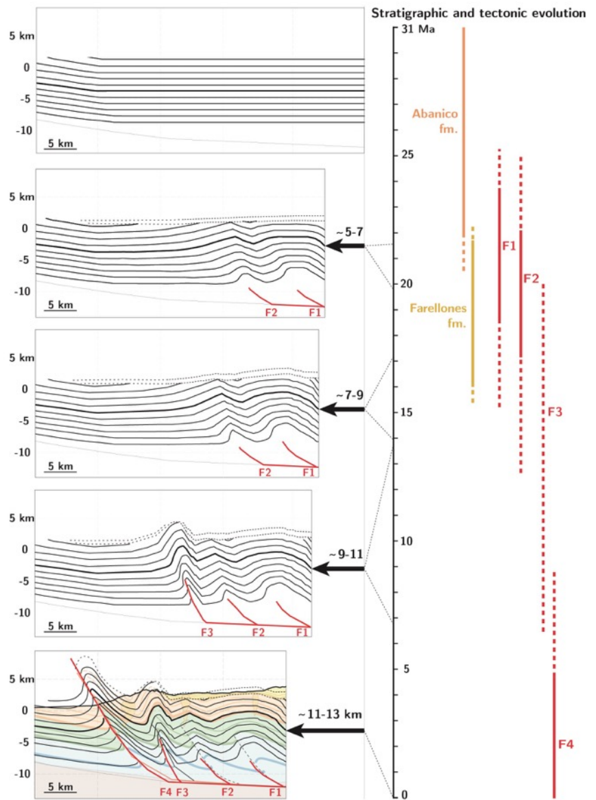
Figure 7. (left) Kinematic evolution of the West Andean fold-and-thrust belt from trishear modeling performed with FaultFold Forward v.6 (freely available from http://www.geo.cornell.edu/geology/faculty/RWA/programs/faultfoldforward.html [Allmendinger, 1998]). The folded structure is modeled by four propagating on-sequence faults ramping up from a décollement. The faults are labeled F1 to F4, with reference to the section of Figure 6. Only the most frontal fault, F4, corresponding to the active San Ramón fault propagates to the surface. Dashed lines indicate layers added at the surface during modeling to simulate deposition of the syntectonic Farellones formation. (right) Synthesis of chronological constraints, as deduced from growth strata within the Farellones formation (see text for further discussion).
