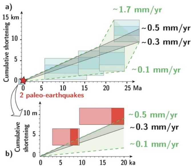
Figure 8. Evolution of tectonic shortening across the Western Andean fold-and-thrust belt (WAFTB) since \sim 25 Ma. (a) Cumulative shortening (relative to present-day) across the WAFTB as a function of time, as deduced from our geological observations (Figures 3 to 6) and kinematic model (Figure 7). The four blue boxes represent shortening accumulated during the four time intervals separating the five temporal steps shown on Figure 7. The dimensions of the boxes represent the range of possible values for shortening (as deduced from our modeling) and timing. An additional 2-3 km uncertainty is represented in light blue and corresponds to the uncertainty estimated from our hand-drawn cross-section. These data are consistent with a long-term average shortening rate of 0.3 – 0.5 mm/yr over the last 25 Myr. The data may however suggest more complex kinematics with an initial higher shortening rate of \sim 1.7 mm/yr prior to \sim 18 -22 Ma, followed by a lower rate of 0.1 to 0.5 mm/yr from \sim 20 Ma to present-day (see discussion in text). (b) Comparison between long-term shortening rates deduced from Figure 8a and occurrences of the two paleo-earthquakes documented by trenching across the San Ramón fault (red boxes, Vargas et al. , 2014). Larger, light red boxes represent the additional uncertainties in time based on the available age constraints [ Vargas et al. , 2014].
