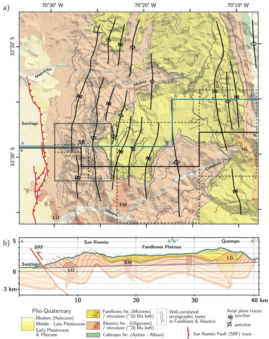
Figure 3. (a) Structural map of the West Andean fold-and-thrust belt (WAFWB), based on earlier map by Armijo et al. [2010] (see location on Figure 1), including well-correlated 3D stratigraphic horizons (grey lines) mapped on DEM-based topography from observations on satellite imagery and aerial photographs, checked carefully with systematic field observations. Here, the traces of the 3D layers are significantly refined by using high-resolution satellite images from the Google Earth database (Landsat 7, DigitalGlobe), digital elevation models (Aster DEM ~30m resolution) and new helicopter views (Figures 4 and 5). For simplicity, we only represent here horizons that correlate well over several kilometers in Abanico and Farellones formations. Additional details are provided as supplementary material, in particular finer stratigraphic horizons required for the projection on the cross-section (see Figure S1 and S2). Major anticline and syncline axes are represented by black arrowed lines. SRF: San Ramón fault ; Q: Cerro Quempo; LO: La Obra pluton, EM: El Manzano pluton; LG: La Gloria pluton. Dashed-line rectangles correspond to the swaths used for the projection of horizons along the a-b section (in black, see text and figures 4 and S1 for further explanations). AA'-A''-A''' section (in blue) represents here the topographic profile, with the minimum altitude required for projecting all structures observed within the swath boxes. Box in black locates figure 4a. Strike and dip measurements are extracted from 3D-mapped continuous horizons, not from discrete field measurements of small-scale features (see text for further explanations). Georeferenced horizons can be retrieved from supplementary data. (b) Synthetic sub-surface cross-section representing form lines deduced by projecting stratigraphic horizon geometries with the swath boxes along section a-b, with the maximum elevation along the combined sections A-A' and A''-A''' (Figure 3a, see Figure S2 of the supplementary materials for detailed stratigraphic horizons projection). Figure 4 further illustrates our projection technique. Direct surface observations are possible from mountain tops down to valley bottoms. Interpretation at depth is deduced from this sub-surface projection, and represented with transparency. Thin blue line reports Maipo and Colorado river bed profiles, that define the limit between directly observed structures and extrapolations at depth.
