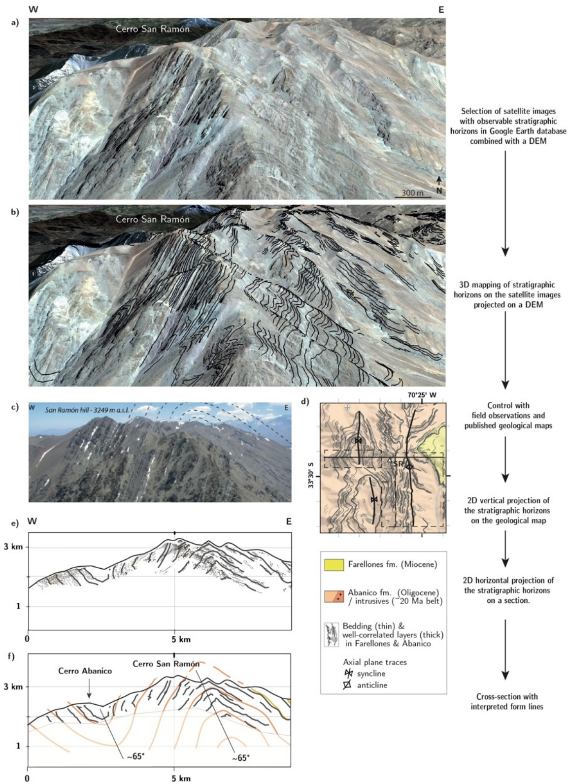
Figure 4: Construction of our 3D-map, illustrated from the specific example of the Cerro San Ramón. (a) High-resolution satellite image of the Cerro San Ramón from the Google Earth database (Landsat 7, DigitalGlobe) projected on a digital elevation model. (b) Same satellite image with the visible stratigraphic horizons mapped in 3D. (c) Field picture of the Cerro San Ramón. (d) Structural map of Cerro San Ramón (SR - black box on Figure 3a). 3D stratigraphic horizons within the swaths marked by dashed boxes are projected onto the section. No strike and dips are represented on the map as we mapped continuous horizons in 3D (see text sections 3.1 and 3.2 for further explanations). Discontinuous stratigraphic horizons are in grey and well-correlated ones are in black. (e) E-W section showing bedding altitudes, obtained by projecting the structural elements (stratigraphic horizons) mapped on the DEM within the dashed boxes (Figure 4a). Discontinuous stratigraphic horizons are in grey and well-correlated ones are in black. (f) Synthetic cross-section deduced from b, showing geometry of the Cerro San Ramón folded structure. The San Ramón anticline and associated Cerro Abanico syncline appears reversed with a clear west-vergence. See Figure 5a and 5b for aerial views of these folds. Well-correlated stratigraphic horizons are in black and interpreted form lines are in orange (Abanico formation) and in yellow (Farelloles formation). Gray lines represent elevation envelope within the swath profiles.
