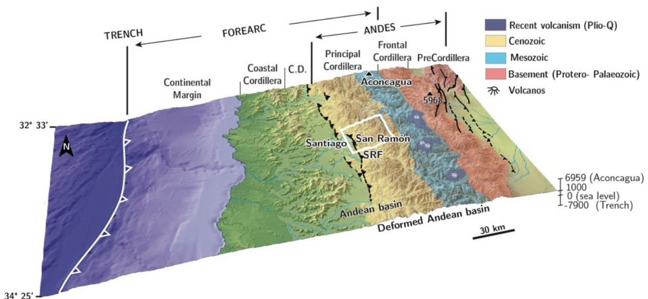
Figure 1. Physiographic view and first-order geology of the subduction margin of the Andes at ~33°S (central Chile and westernmost central Argentina). To the west, the trench marks Nazca-South America plate boundary (in white with open triangles). The Andes mountain belt, ~100km wide at this latitude, is basically made of the Frontal Cordillera basement culmination to the east, and of the folded and thrustured Mesozoic-Cenozoic rocks of the Principal Cordillera to the west. The San Ramón fault (SRF, black segmented line with triangles) marks the western andean front facing the Central Depression (CD) and Santiago city. Main thrusts at the eastern andean front are also indicated in black. See text for further description of geology and tectonic units. White rectangle locates our study area covered by the map of Figure 3.
