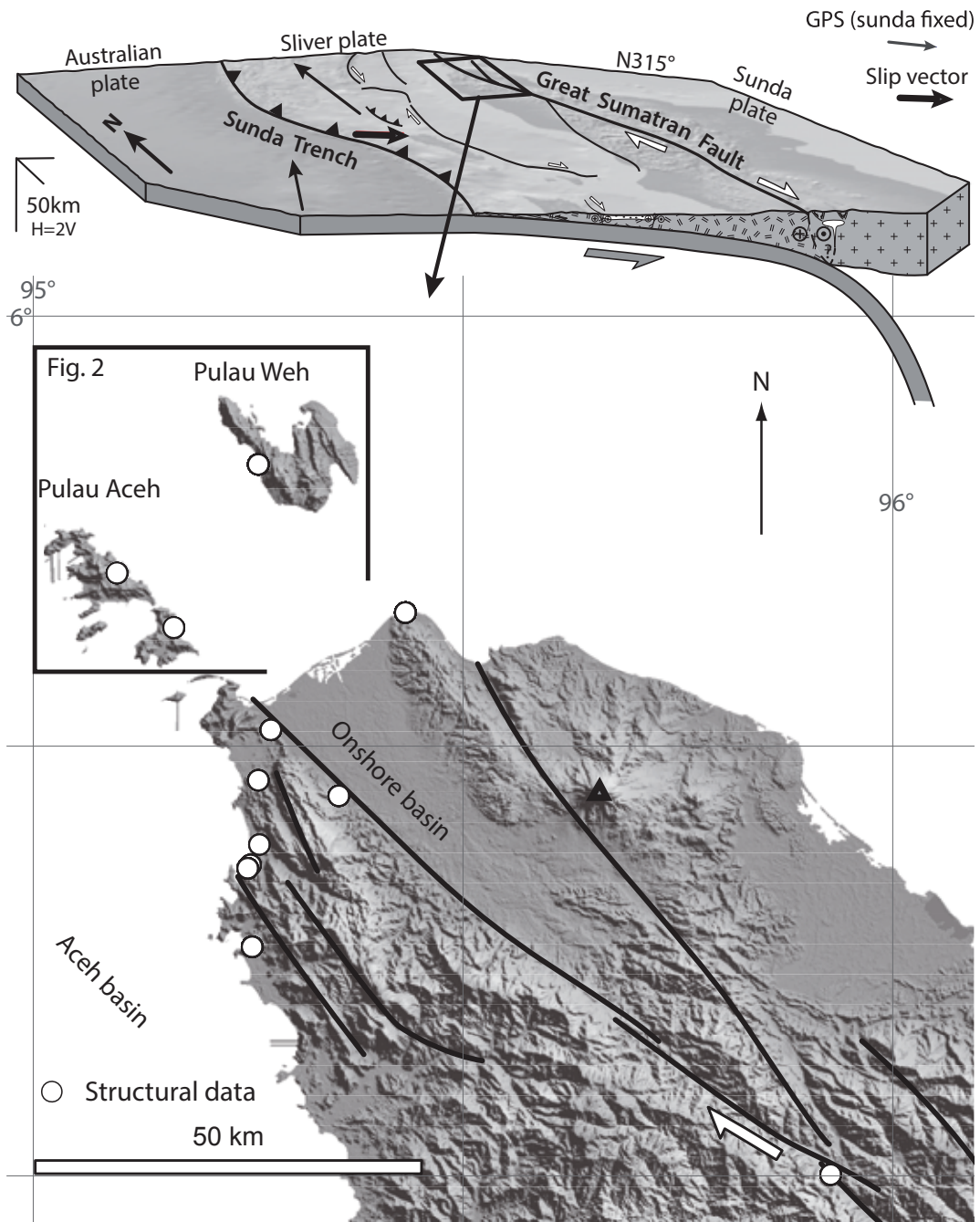
Fig. 1. 3D regional tectonic configuration in the Sumatran section of the Sunda arc-trench system (upper panel), and map-view of the GSF. White dots represent location of the data used in this contribution.
