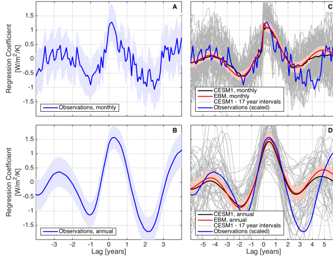
Figure 1. Lagged regressions between de-seasonalized anomalies in global TOA radiation and surface temperature A Observational data sets from 03/2000 to 10/2017. Monthly TOA radiation from CERES [Wielicki et al. , 1996], and monthly global mean surface temperature from GISTEMP [Hansen et al. , 2010]. Greenhouse gas and aerosol forcing is removed and data is processed as in Donohoe et al. [2014]. Shading illustrates 95% regression uncertainty estimates. B Same as A , but for annually averaged anomalies. C Monthly anomalies from a 1,000 year long pre-industrial control run of CESM1 (black), and the EBM (red) prediction. Pink shading illustrates a 95% uncertainty estimates on EBM regression coefficient based on 1,000 Monte Carlo draws. Grey lines indicate lagged-regression structures from 50 non-overlapping segments of the CESM1 simulation, each of equal length to the observational dataset. Blue line indicates the observational lagged-regression structure, scaled as r_{\text{obs}}^{\text{scaled}}(\text{lag}) = r_{\text{obs}}(\text{lag} \cdot 5/3) , with the ratio of 5/3 mimicking the ratio of ENSO periodicity in CESM1 and observations. D same as C but for annually averaged anomalies.
