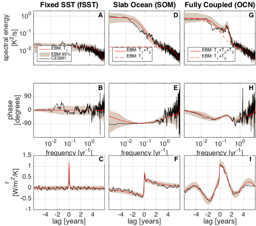
Figure 3. Analytical spectrum, phase difference, and lagged regression coefficient, r , of net TOA anomalies, Q , versus global mean near-surface air temperature, T in a CESM1 control run hierarchy. The hierarchy consists of a fixed SST run (A-C), a slab ocean run (D-F), as well as the fully coupled control run (G-I). The statistics are depicted for CESM1 integrations (black), along with EBM (red) fit. A 95% range of EBM realizations is depicted, based on 1,000 Monte Carlo draws. Spectra are computed using a Multi-Taper algorithm with 8 windows.
