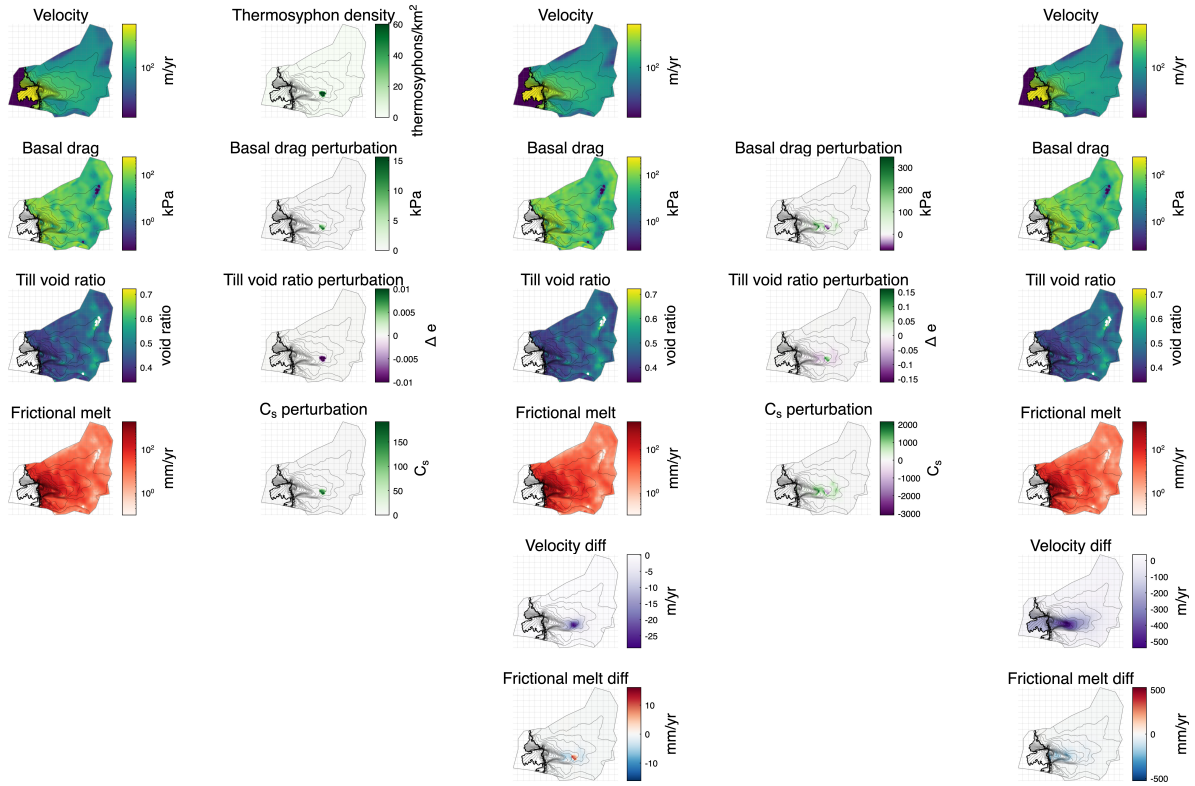
Figure S6: Extended version of ?? which includes the initial state of Thwaites glacier (first column), the calculated perturbation to basal drag due to thermosyphons (second column), the resulting new state of Thwaites glacier (third column), a further meltwater feedback perturbation (fourth column), and the resulting new state of Thwaites glacier (fifth column).
