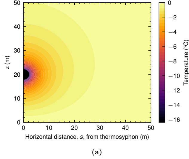
Fig. 7. Temperature around evaporator area of thermosyphon calculated evaporator d = 20 m from the bed, with r_{\text{evap,eff}} = 2 m, after 20 years.
