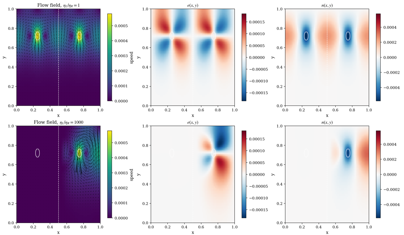
FIGURE 6 – Flow in the two-region Cartesian benchmark. The upper row is isoviscous, with \eta_L/\eta_R = 1 . The lower row has \eta_L/\eta_R = 1000 . From left to right, the columns show the velocity magnitude and vectors, the horizontal component e(x, y) , and the vertical component n(x, y) . White contours mark the two negatively buoyant bodies. The dashed line marks the centre of the viscosity transition. Increasing the viscosity on the left suppresses both the descent of the left body and the circulation that it drives.
