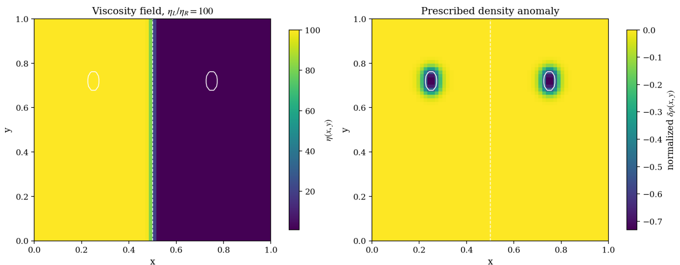
FIGURE 5 – Geometry of the two-region Cartesian benchmark on a 64 \times 64 grid. The left panel shows the prescribed viscosity for \eta_L/\eta_R = 100 . The more viscous material occupies the left half of the box. The right panel shows the two identical normalized density anomalies. The dashed line marks the centre of the viscosity transition and the white contours outline the buoyant bodies. The transition in viscosity and the edges of the density anomalies are smoothed over finite widths.
