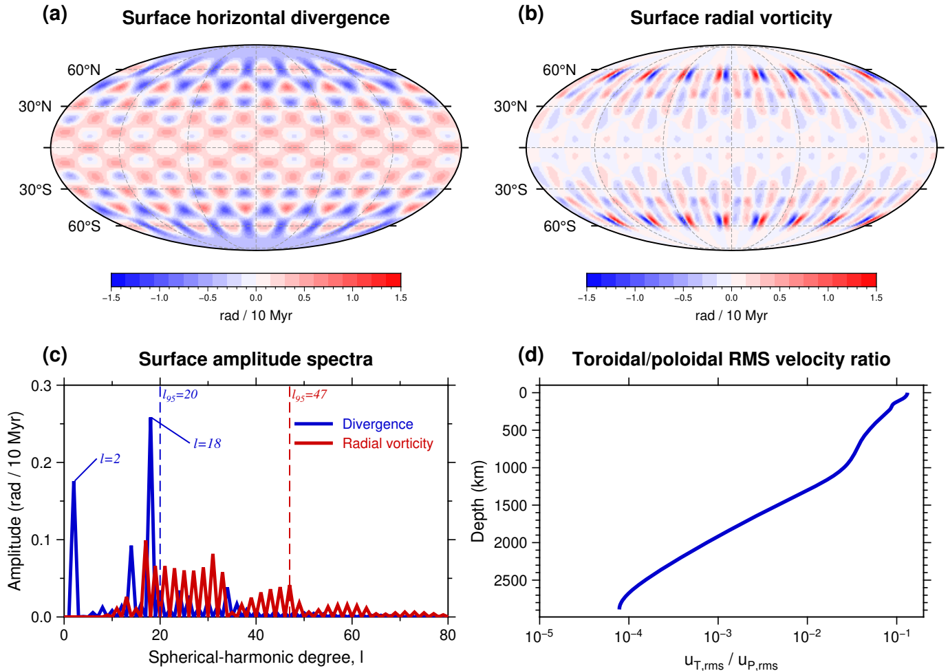
FIGURE 10 – Physical diagnostics for the spherical calculation with a viscosity contrast of 10^4 . (a) Surface horizontal divergence. (b) Surface radial vorticity. The two maps use the same Forte–Peltier normalization and the same symmetric range of [-1.5, +1.5] rad/10 Myr. (c) Degree amplitudes of surface divergence in blue and radial vorticity in red. The dashed markers give \ell_{95} , defined as the smallest degree containing at least 95% of the cumulative squared degree amplitude. The values are \ell_{95} = 20 for divergence and \ell_{95} = 47 for radial vorticity. The labelled degree-two and degree-18 divergence peaks distinguish the directly forced response from the strongest member of the first poloidal band opened by viscosity coupling. (d) RMS toroidal-to-poloidal velocity amplitude ratio as a function of depth, u_{T,rms}/u_{P,rms} = \sqrt{E_T/E_P} . The map grids are interpolated at one-degree spacing for display only; all quoted spectra and RMS quantities are evaluated directly from the spectral solution.
