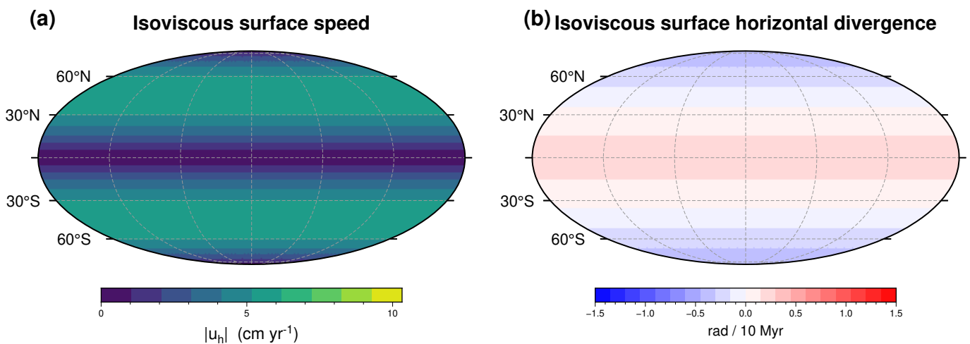
FIGURE 9 – Resolution-matched isoviscous control for the spherical calculation. (a) Magnitude of the physical surface horizontal velocity. (b) Physical surface horizontal divergence in the Forte–Peltier normalization. Every parameter apart from the amplitude of the lateral viscosity field is the same as in Fig. 8. Panel (a) uses the same 0\text{--}10.3256 \text{ cm yr}^{-1} colour scale as Fig. 8(d), and panel (b) uses the same [-1.5, +1.5] \text{ rad}/10 \text{ Myr} scale as Fig. 10(a).
