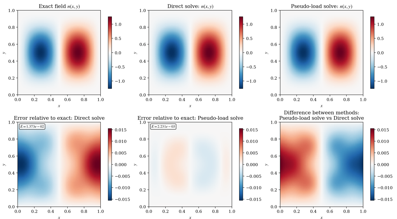
FIGURE 3 – As in Fig. 2, but for the velocity component n(x, y) . The exact field and the two numerical solutions are shown above. Their errors and mutual difference are shown below. The close agreement of the transformed solution with the prescribed field is obtained while the viscosity varies by four orders of magnitude.
