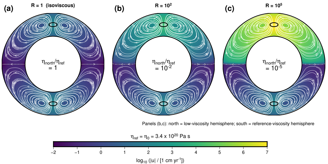
FIGURE 11 – Meridional sections of the physical velocity for the hemispheric viscosity test. The nominal viscosity contrasts are (a) R = 1 , (b) R = 10^2 , and (c) R = 10^5 . The southern hemisphere has the reference viscosity \eta_{\text{ref}} = 3.4 \times 10^{20} \text{ Pa s} , while the northern viscosity is \eta_{\text{north}}/\eta_{\text{ref}} . The colour scale is common to all three panels and shows \log_{10}(|\mathbf{u}|/[1 \text{ cm yr}^{-1}]) . White curves are streamlines of the physical velocity and the arrowheads show their direction. The black outlines mark the location and shape of the two identical, antipodal density anomalies.
