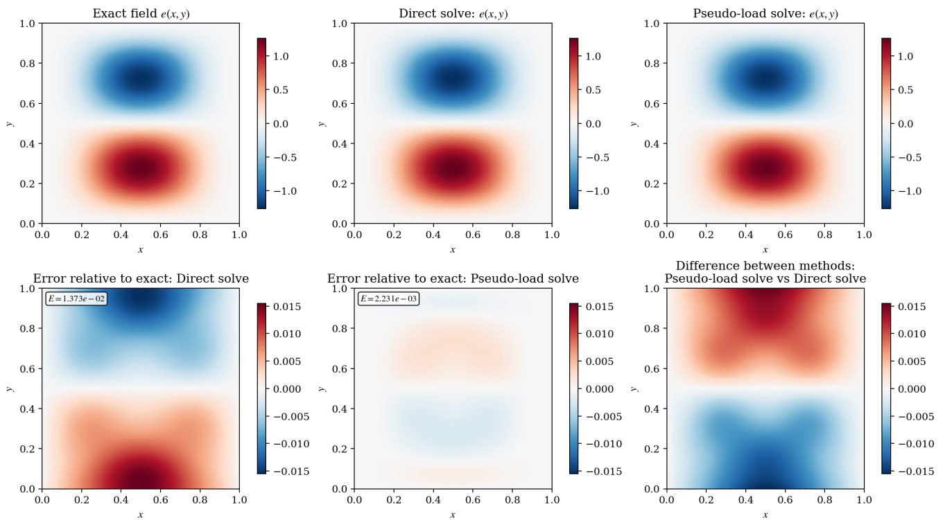
FIGURE 2 – Manufactured solution benchmark for the velocity component e(x, y) on a 128 \times 128 grid. The upper row shows the exact field, the solution from the direct variable viscosity discretization, and the solution from the transformed formulation. The lower row shows the corresponding errors relative to the exact field and, at right, the difference between the two numerical solutions. The quantity E denotes the relative L_2 error.
