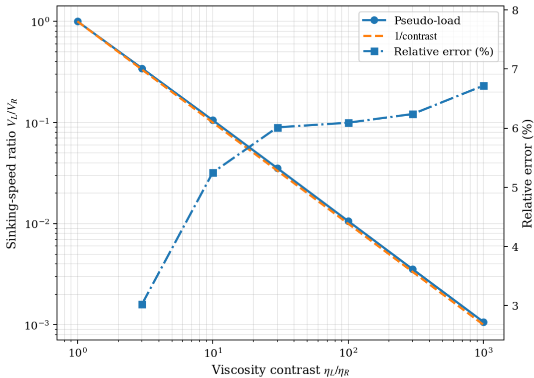
FIGURE 7 – Sinking speed ratio in the two-region Cartesian benchmark. The blue curve is the computed ratio V_L/V_R . The orange dashed curve is the inverse-viscosity scaling 1/(\eta_L/\eta_R) . The right axis gives the relative difference between the two. The agreement persists through \eta_L/\eta_R = 1000 , where the finite transition width, finite body size, and bounded domain account for a remaining difference of about 6–7%.
