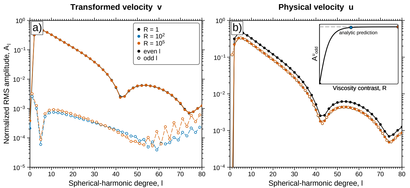
FIGURE 13 – Normalized velocity spectra for the hemispheric viscosity test. The degree amplitude is defined by Eq. (144). Filled symbols show even degrees and open symbols show odd degrees. (a) Transformed velocity \mathbf{v} . The spectrum remains dominated by the same even degrees as R increases, while only a small odd component develops. (b) Physical velocity \mathbf{u} = e^{-\Lambda} \mathbf{v} . At large R , the even and odd amplitudes become comparable although the streamline geometry remains close to the isoviscous case. The large odd contribution in \mathbf{u} arises chiefly from the hemispheric variation of the scalar factor e^{-\Lambda} , while the small odd contribution in \mathbf{v} records the change in the transformed flow itself. The inset in panel (b) shows the analytic prediction from Eq. (147) for the integrated odd-degree RMS amplitude A_{\text{odd}}^{(u)} = (R - 1) / \sqrt{2(R^2 + 1)} , as a function of viscosity contrast R . The coloured symbols show the corresponding numerical values at R = 10^2 and 10^5 , while the horizontal dashed line marks the large- R limit A_{\text{odd}}^{(u)} = 1/\sqrt{2} . The associated odd-to-even amplitude ratio is given by Eq. (148).
