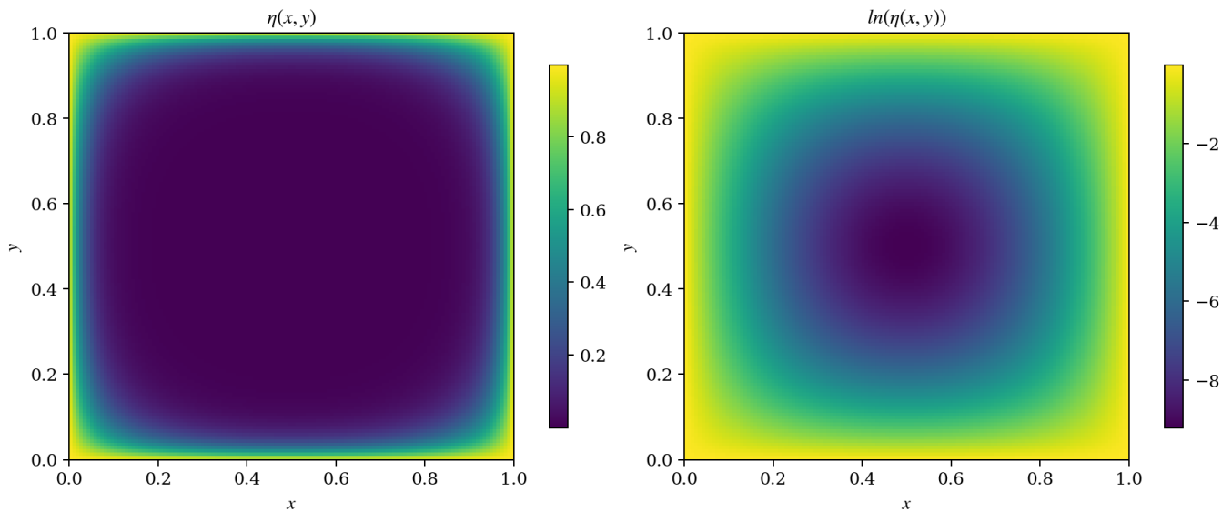
FIGURE 1 – Prescribed viscosity in the manufactured solution benchmark. The left panel shows \eta(x, y) . The right panel shows \ln \eta(x, y) , the field whose gradient enters the transformed equations. The viscosity varies smoothly across four orders of magnitude. The two panels therefore also illustrate the compression of a large multiplicative viscosity range when it is represented in logarithmic form.
