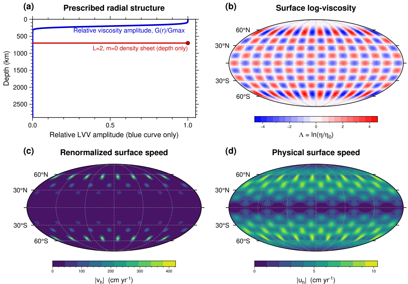
FIGURE 8 – Prescribed structure and surface response of the spherical calculation with \eta_{\max}/\eta_{\min} = 10^4 . (a) Radial envelope of the imposed (L_\eta, m_\eta) = (16, 8) logarithmic viscosity field. The red line marks the depth of the exact (s, m) = (2, 0) buoyancy sheet at 700 km. It is a depth marker, not a representation of a finite source thickness. (b) Surface \Lambda = \ln(\eta/\eta_0) . (c) Magnitude of the renormalized surface horizontal velocity |\mathbf{v}_h| , the variable on which the reference Stokes operator acts. (d) Magnitude of the reconstructed physical surface horizontal velocity |\mathbf{u}_h| . Coastlines are omitted because the lateral structure is an ideal harmonic pattern rather than a geographic model.
