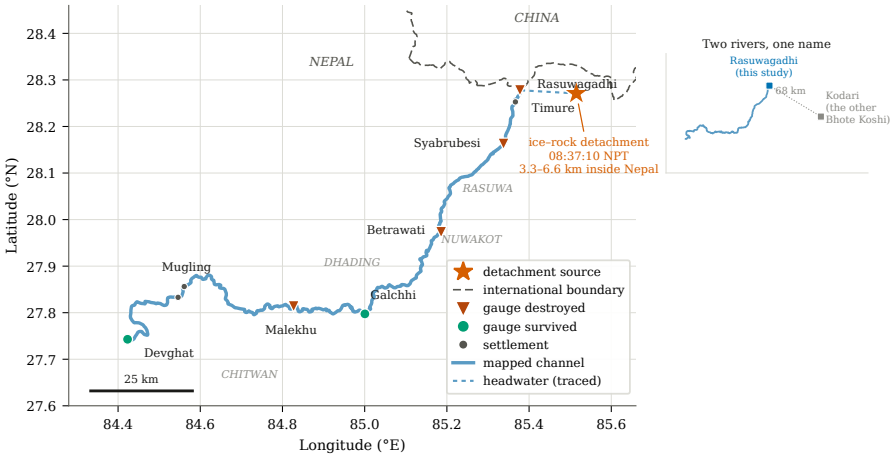
Figure 1. Study area, from OpenStreetMap channel and boundary data. The star marks the detachment source, 3.3 to 6.6 km inside Nepal, and the dashed segment the headwater reach, drawn schematically, its length traced on terrain at 20.1 to 24.0 km. Triangles are gauging stations destroyed on 26 August, circles those that survived. The inset distinguishes the two Nepali rivers named Bhote Koshi.
