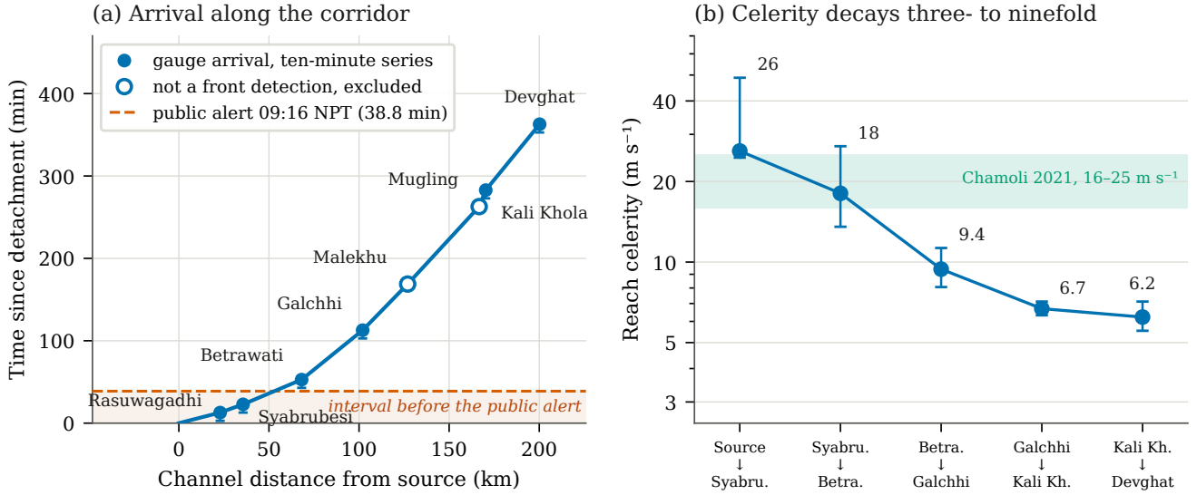
Figure 2. Propagation of the flood wave. (a) Arrival time against measured channel distance from the source. Filled markers are gauge arrivals read from the ten-minute stage series, open markers the two nodes timed by a threshold crossing and by a confirmed-past bound, neither of which detects the front, so both are excluded from the celerity estimates. Horizontal bars give the headwater distance range and vertical bars the arrival brackets set by station reporting cycles. The dashed line marks the mass public alert. (b) Reach-integrated celerity, decaying by a factor of three to nine. Bars carry arrival-time as well as distance uncertainty. The band shows Chamoli 2021 velocities at comparable range (Shugar et al., 2021).
