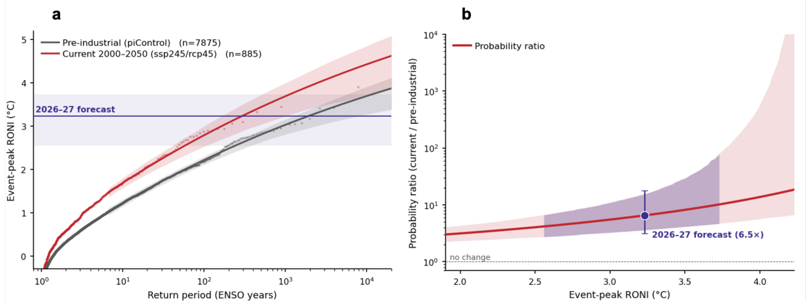
Figure 2. Attribution of extreme El Niño likelihood to anthropogenic warming. a , Return levels of annual peak RONI in the pre-industrial climate (piControl, grey) and the current climate (2000–2050 of historical + RCP4.5/SSP2-4.5, red), pooled across 18 evaluated CMIP models. Dots show empirical annual maxima, solid lines show the common-shape generalised Pareto fits, and shading highlights the 5th–95th percentile range from a bootstrap resampling across models. The horizontal purple line and shading show the forecast 2026/27 magnitude and its 5th–95th percentile range across forecast members. b , Probability ratio between the current and pre-industrial climates as a function of event magnitude. The red line shows the central estimate and red shading highlights the bootstrap 5th–95th percentile range; the purple shaded region highlights the same range over the magnitudes spanned by the forecast uncertainty. The purple marker shows the central estimate of the forecast magnitude, and vertical bars show the bootstrap range on the probability ratio for the central estimate. The dashed line marks a probability ratio of one, indicating no change in likelihood.
