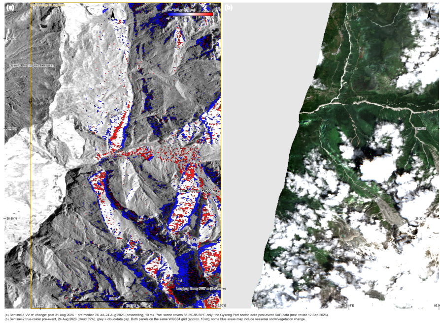
Fig. 3 Sentinel-1 backscatter change ( \Delta dB , VV) in the source sector (left; blue-white-red) and pre-event Sentinel-2 baseline of 24 August 2026 (right). Post-event SAR coverage is a single descending scene of 31 August; the change analysis is limited to the source sector east of \sim 85.4^\circ E .
