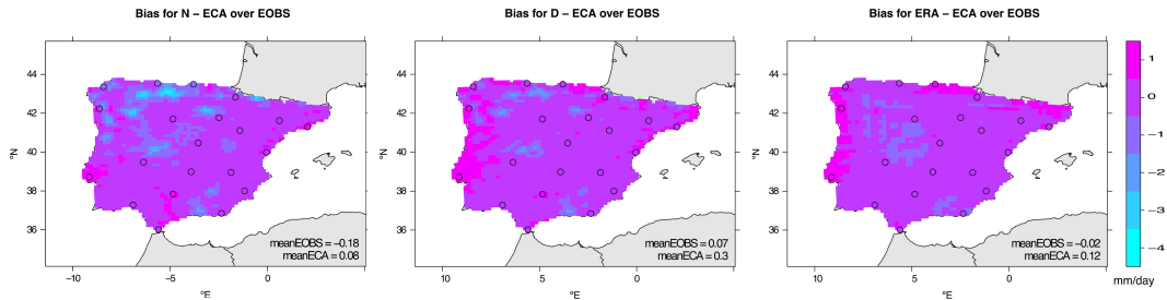
Figure 6. Same as Figure 5, but for bias (mm/day).
