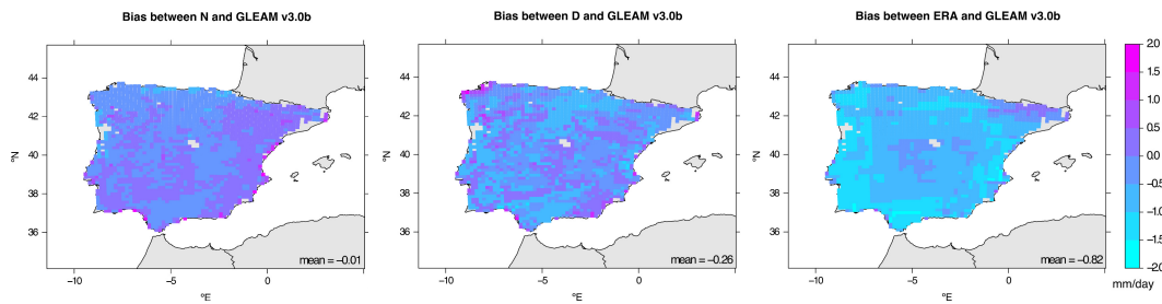
Figure 9. Same as Figure 8 but for bias (mm/day).
