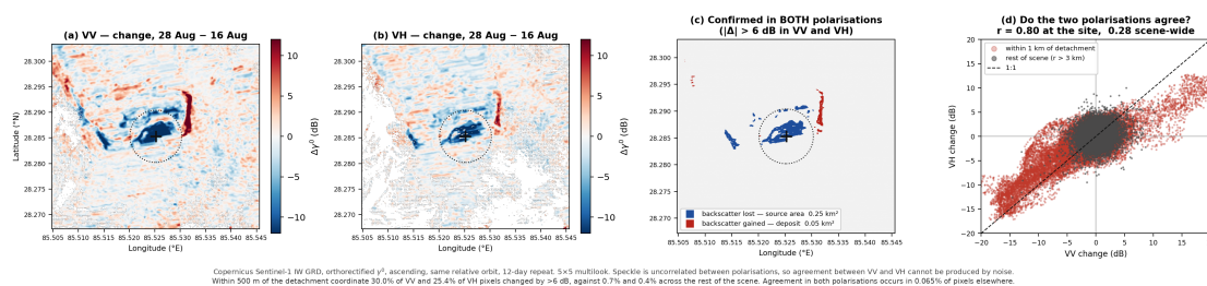
Figure 2. Independent confirmation from the second polarisation, and the correlation structure that distinguishes signal from speckle.
