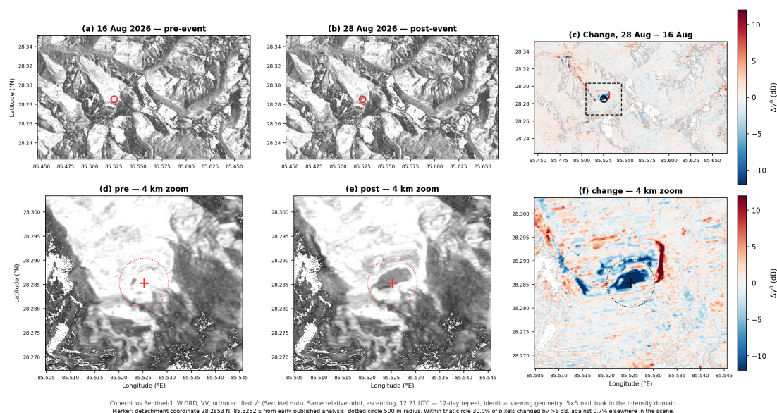
Figure 1. Pre-event, post-event and difference (28 August minus 16 August), VV, with a 4 km zoom. Blue: backscatter loss. Red: gain.
