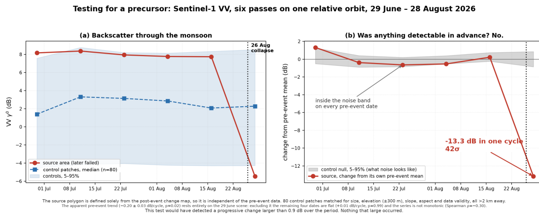
Figure 4. VV time series and anomaly relative to matched controls. The source area remains within the control noise band on every pre-event date.
