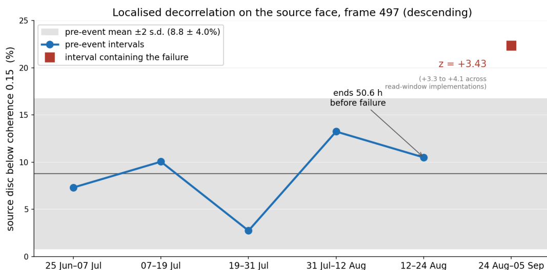
Figure 1. Localised decorrelation on the source face, track B. Fraction of the usable source disc falling below coherence 0.15, for six consecutive twelve-day intervals, the last of which spans the failure. Shaded band is the pre-event mean \pm 2 s.d. ( 8.8 \pm 4.0 per cent). The interval ending 50.6 hours before failure ranks fourth of five; the interval containing the failure departs by z = +3.43 . Sentinel-1D, path 19 frame 497, HyP3 INSAR_GAMMA at 10 \times 2 looks (40 m). Source disc of 500 m radius at 28.2853 °N, 85.5252 °E, restricted to local incidence \leq 70^\circ and no shadow, n = 219 pixels at the native 40 m posting.
