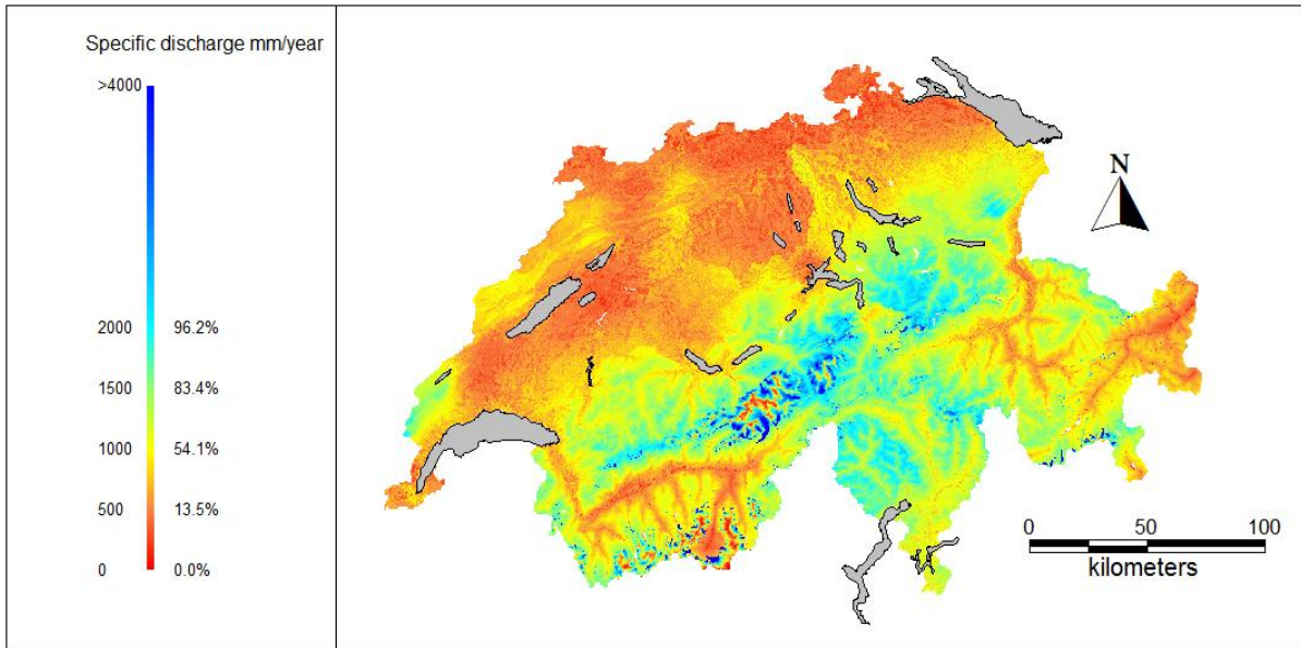
Figure S10: Spatial distribution of annual runoff for the period 1981-2000 in \text{mm yr}^{-1} . Source discharge data: [6]; source vector data: [8]
