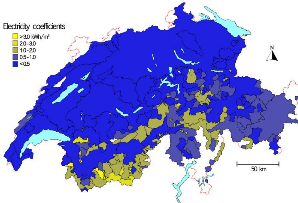
Figure 6: Spatial distribution of electricity coefficients of all HP schemes. The catchments are nested, lowland RoR catchments contain upstream catchments. Light blue corresponds to lake areas. The red line shows the Swiss national boarder.
