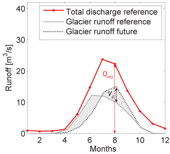
Figure S3: Sketch of the computation of relative glacier runoff volume changes \delta_{ij} (Equation 11 of the main text), obtained as V_{ij} divided by Q_{ref} .
