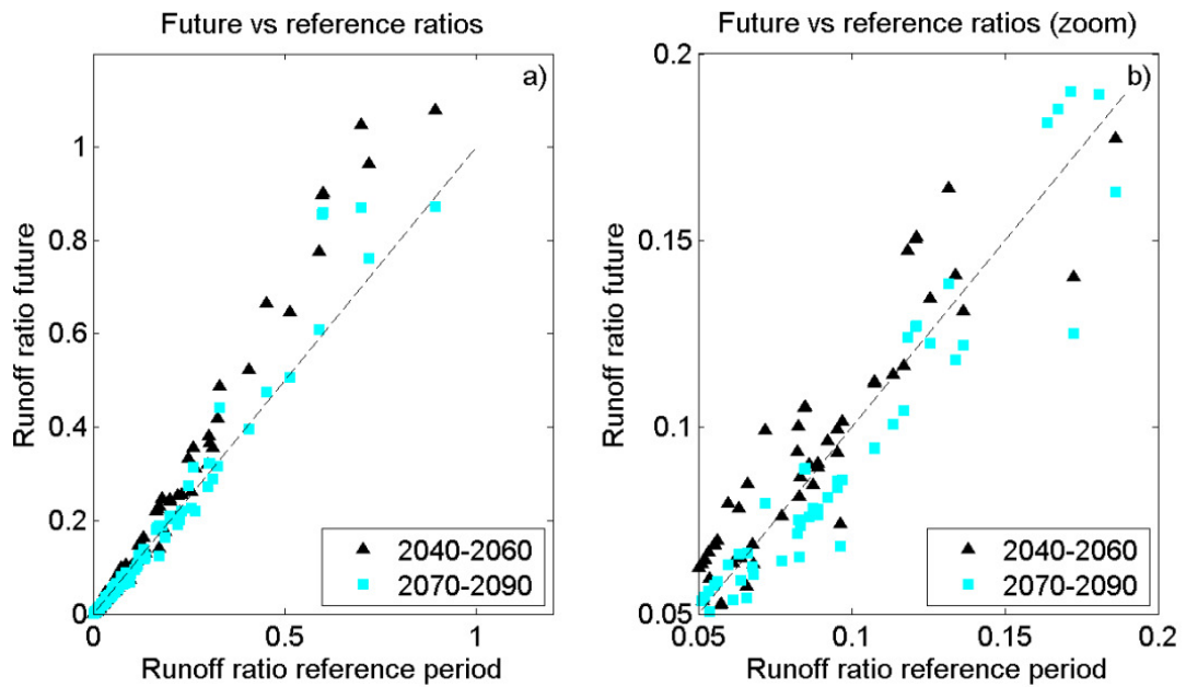
Figure S2: a) Ratio of simulated glacier runoff (total runoff from the glacier-covered part, including ice melt and runoff from rainfall and snowmelt over the glacier) divided by simulated total catchment runoff for all 172 HP schemes that have currently glaciers in their catchments and for three different periods; b) as a) but zoom on small ratios.
