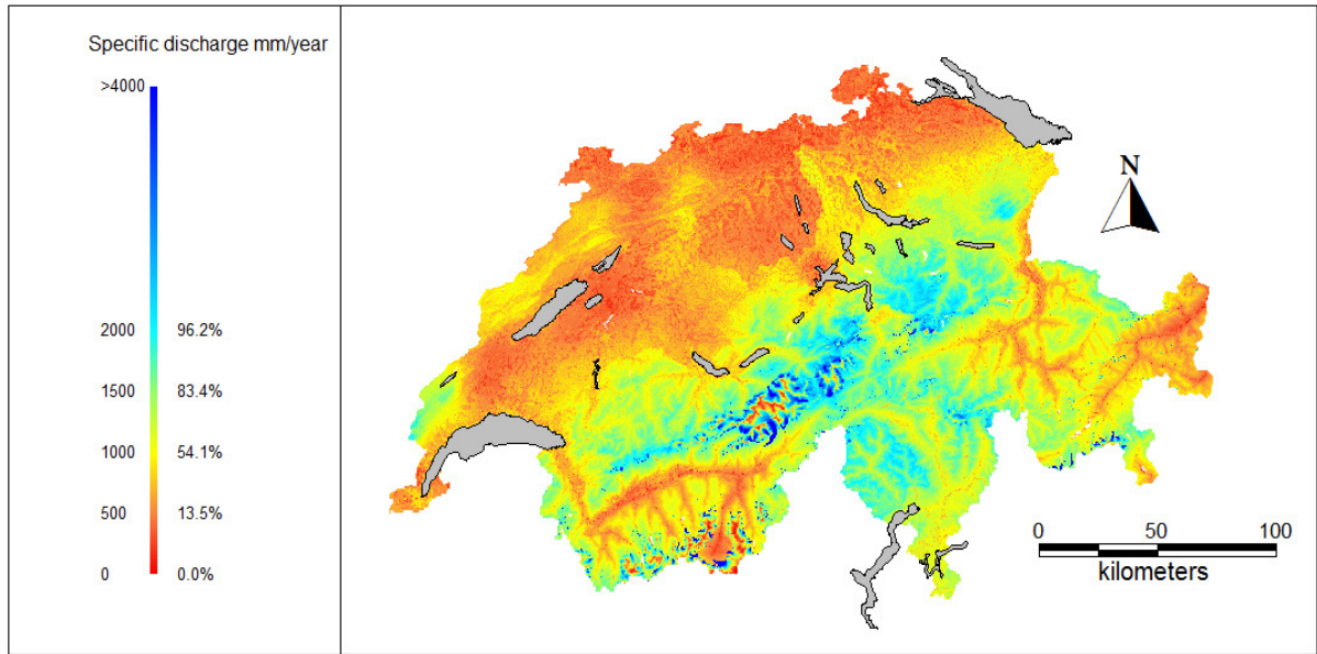
Figure S1: Spatial distribution of annual runoff for the period 1981-2000 in \text{mm yr}^{-1} . Source discharge data: (Zappa et al., 2012); source vector data: (SwissTopo, 2008)
