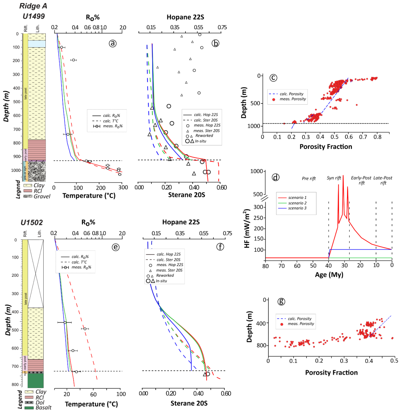
Figure 4 a) R_o\% calibration and calculated maximum temperatures of U1499 well; b) Hopane 22S and Sterane 20S calibration model, of U1499 well; c) measured and calculated porosity evolution with depths, of U1499 well; d) The figure shows the three scenarios used to fit po-rift data. Scenario 1: heat flow evolution at the ocean-continent transition according to Mckenzie heat flow model for rifted margin using a beta factor of 4 and considering results from Nirrengarten et al., (2020a); Scenario 2; constant heat flow to present day values in the syn and post rift stages and 70 \text{ mW/m}^2 in the pre-rift stage; Scenario 3: constant HF value of 70 \text{ mW/m}^2 ; e) R_o\% calibration and calculated maximum temperatures of U1502 well; f) hopane 22S and sterane 20S calibration model, of U1502 well; g) measured and calculated porosity evolution with depths, of U1502 well. RCI in the stratigraphic legend stands for red claystones, while Dol for dolomite.
