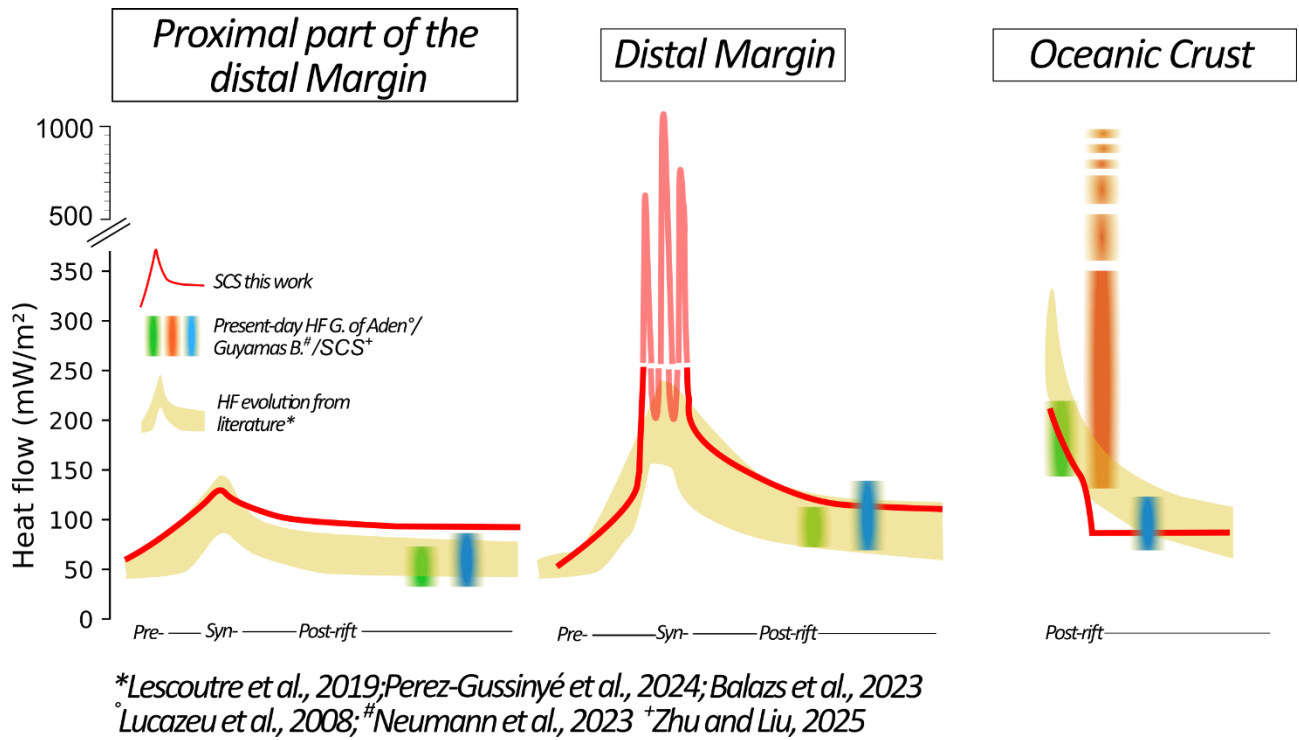
508 Figure 8 Comparison between the SCS thermal history calculated in this work and those from other studied margins and present-day 509 data.
