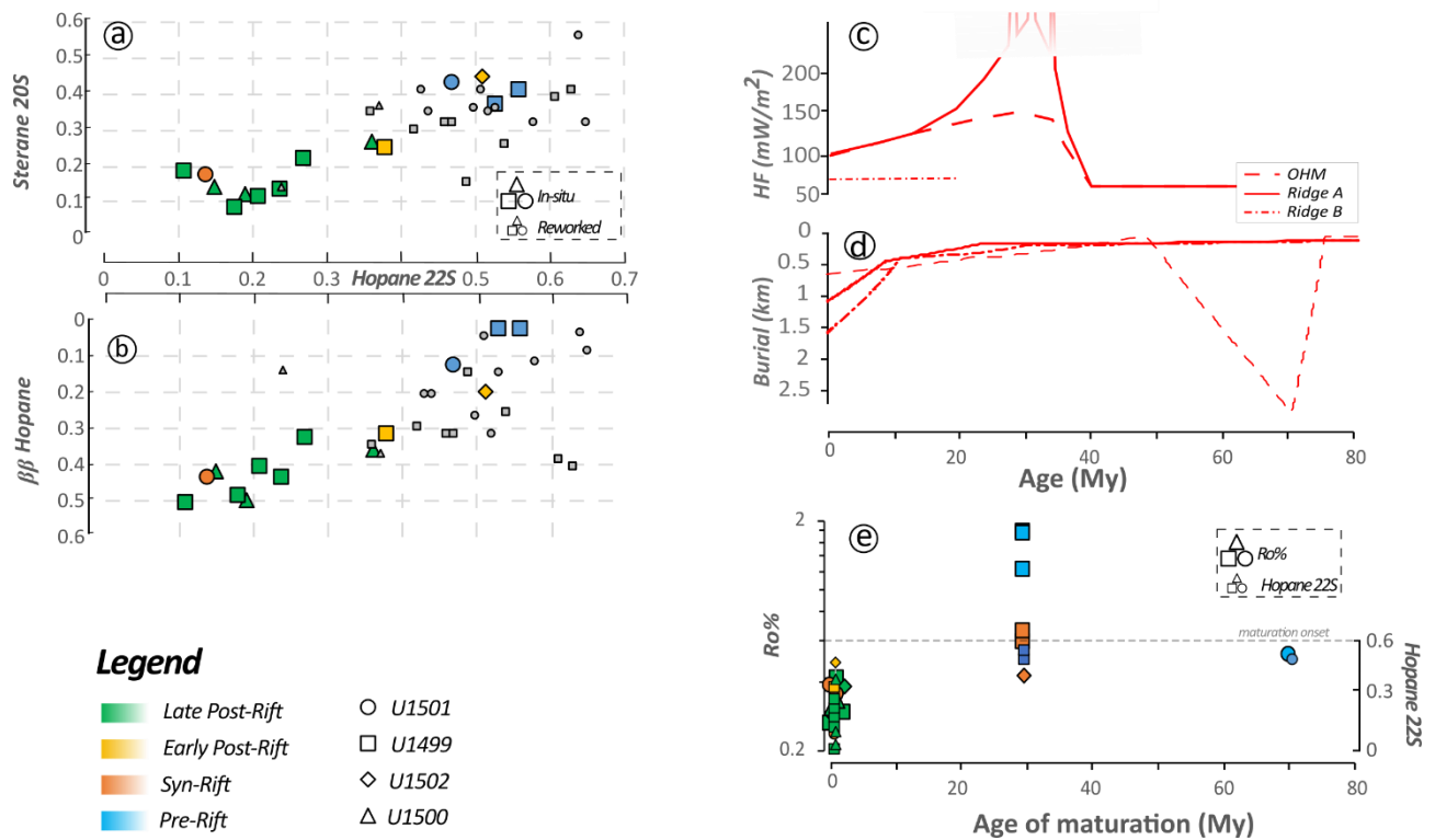
Figure 6 a) Sterane 20S and b) \beta\beta hopane data plotted against Hopane 22S (note here the inverse order of the y-axis). c) heat flow and d) burial histories used to model thermal maturity data. Sea-level variation has not been included in this graph but is has been used in modelling calibration. e) thermal maturity expressed as R_o\% and Hopane 22S against the age of maturation used in modelling. R_o\% in logarithmic scale. Note that reworked data has not been used in figure e.
