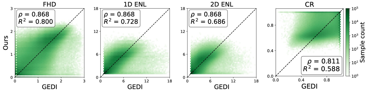
Figure 8: Agreement between diversity indices derived from the VSM and GEDI, at the footprint level.
