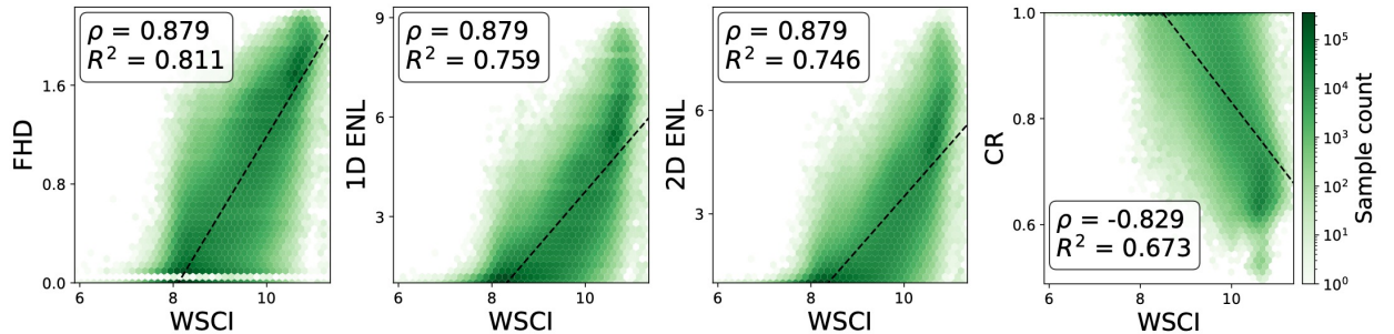
Figure 9: Agreement between VSM-derived diversity indices and the Waveform Structural Complexity Index (WSCI)[5] at 1 km resolution.
