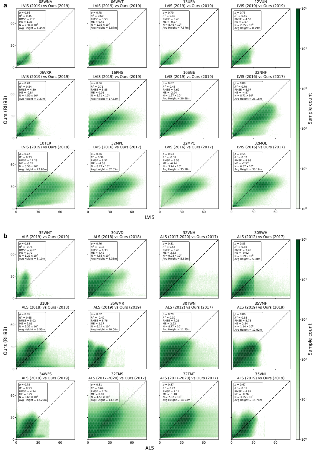
Extended Data Figure A2: Predicted canopy top height overall agrees with independent airborne LiDAR across diverse geographic regions. Density scatter plots comparing our canopy height estimates (RH98, y-axis) against independent airborne LiDAR reference data (x-axis) for a , 12 LVIS tiles across North and Central America and Africa, and b , 12 ALS tiles across Europe. Each scatter plot corresponds to a Sentinel-2 tile, with the acquisition years of the reference data and the corresponding prediction indicated in the title. Colour intensity indicates sample count on a logarithmic scale. The dashed line represents the 1:1 identity. Per-tile R^2 , RMSE, ME, sample count (N), and average reference height are reported.
