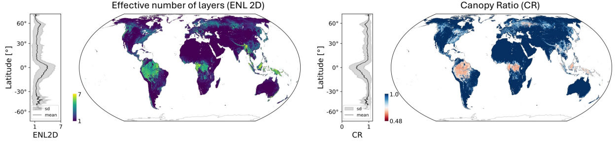
Figure 10: Global distribution of the VSM-derived diversity indices 2D effective number of layers (ENL) and canopy ratio (CR) at 1 km, with corresponding latitudinal profiles.
