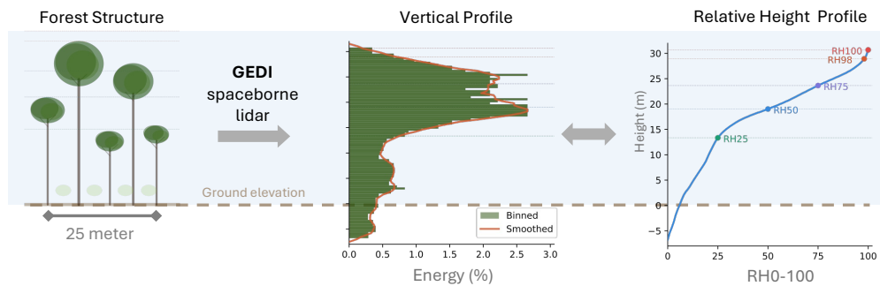
Figure 1: The GEDI sensor measures sparse vertical profiles of vegetation structure within a 25m footprint. This data is represented as 101 Relative Height (RH) metrics, each describing the height above ground at which a certain percentage of the laser energy is returned.
