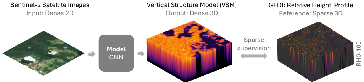
Figure 2: To densify these sparse GEDI measurements, a deep learning model computes a dense vertical structure model (VSM) from optical satellite images under sparse supervision.
