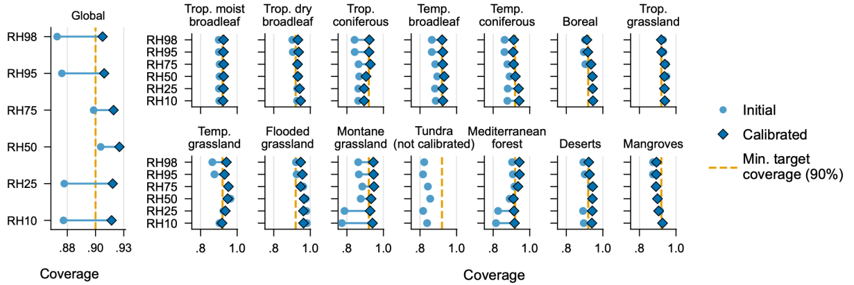
Figure 6: Coverage of prediction intervals improves after calibration with conformal prediction, evaluated globally (left) and stratified by biomes (right).
