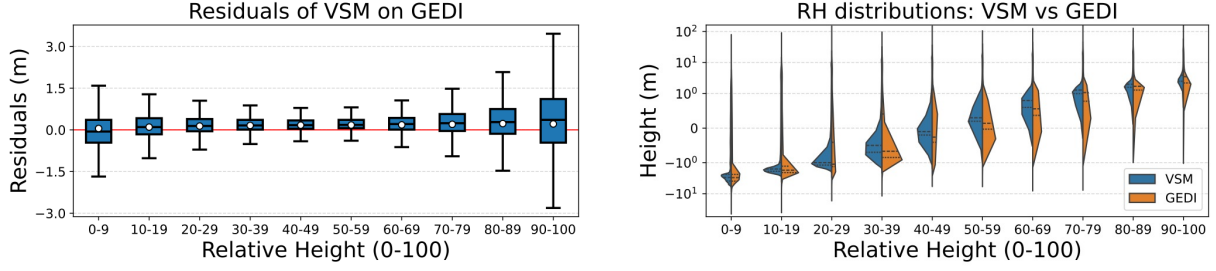
Figure 7: Error distribution (left) and absolute distribution (right) of the estimated RH metrics compared to hold-out GEDI reference data.
