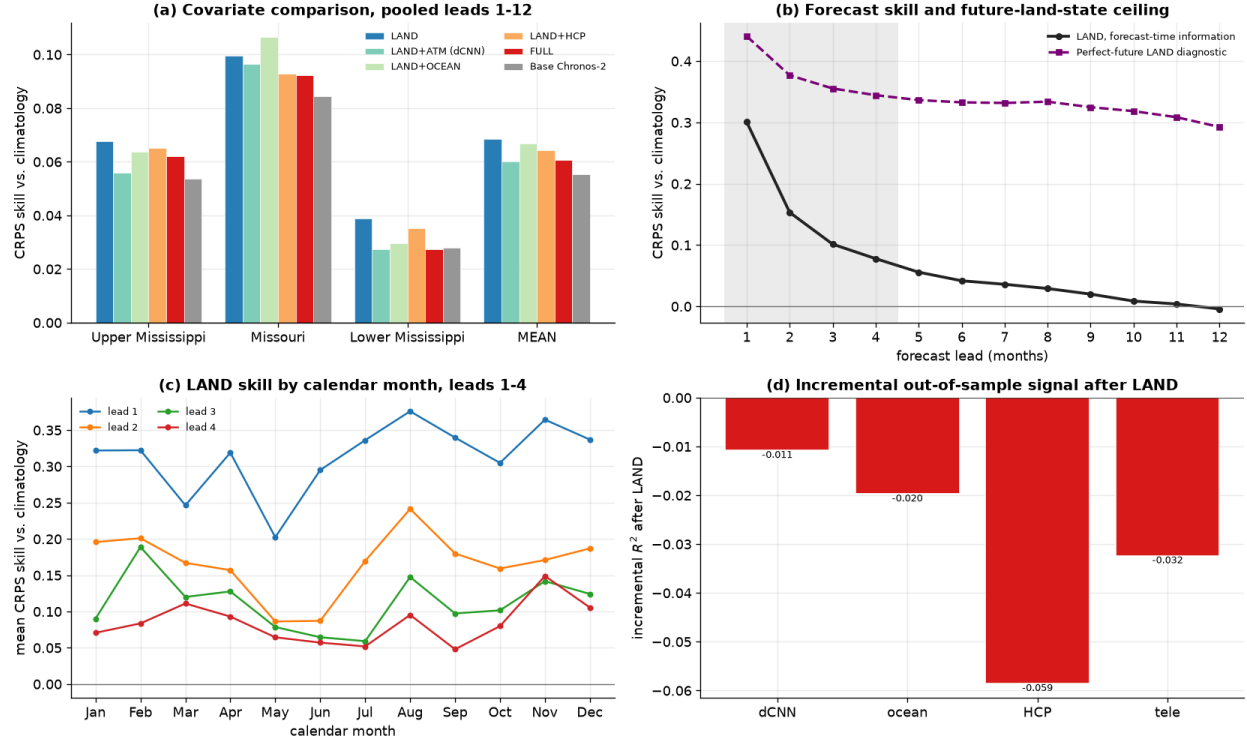
Figure 2. Forecast performance and covariate attribution. (a) CRPS skill versus climatology for the six forecast configurations, calculated using all forecasts from leads 1-12 over the common verification period. (b) Mean LAND skill by forecast lead compared with the perfect-future LAND diagnostic; the shaded region marks the 1-4 month core horizon. (c) Mean LAND skill by calendar month at fixed leads 1-4. (d) Incremental out-of-sample R^2 from adding each predictor block after LAND in the independent staged ridge diagnostic. dCNN denotes the deep convolutional neural-network representation of upper-air circulation; ocean is the learned ocean-to-atmosphere representation based on sea-surface temperature and 0-300 m ocean heat content; HCP comprises direct 0-300 m ocean heat-content precursor indices; and tele comprises scalar teleconnection indices, including Niño-3.4, AMO, IOD, PDO, and lagged Niño-3.4 measures.
