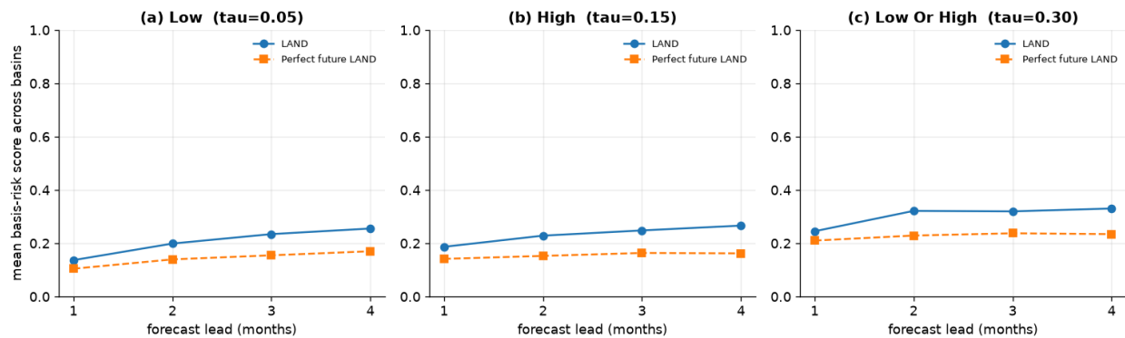
Figure 6. Mean basis-risk score across basins at leads 1-4 for low-water, high-water, and combined low-or-high risk. The score is the equal-weight mean of the missed-disruption rate and unnecessary-payout rate at the risk-specific probability cutoffs shown in Table 4. Solid lines show operational LAND and dashed lines show the perfect-future LAND diagnostic. High-water and combined results are subject to the empirical high-flow proxy limitation.
