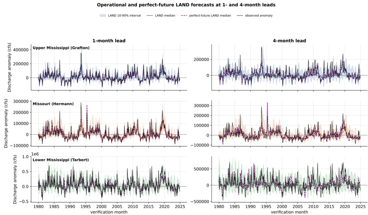
Figure 3. Operational LAND and perfect-future LAND discharge forecasts at 1- (left) and 4- (right) month leads. For each basin, the operational LAND median (solid color) and 10-90% predictive interval (shaded) are shown with the observed discharge anomaly (solid black), and the dashed line shows the perfect-future LAND median. Anomalies are relative to the historical mean for each rolling-origin forecast.
