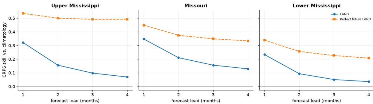
Figure S2. Basin-level CRPS skill versus climatology for operational LAND and perfect-future LAND across leads 1-4. The diagnostic gap is largest at longer leads and is especially pronounced for the Upper Mississippi.
