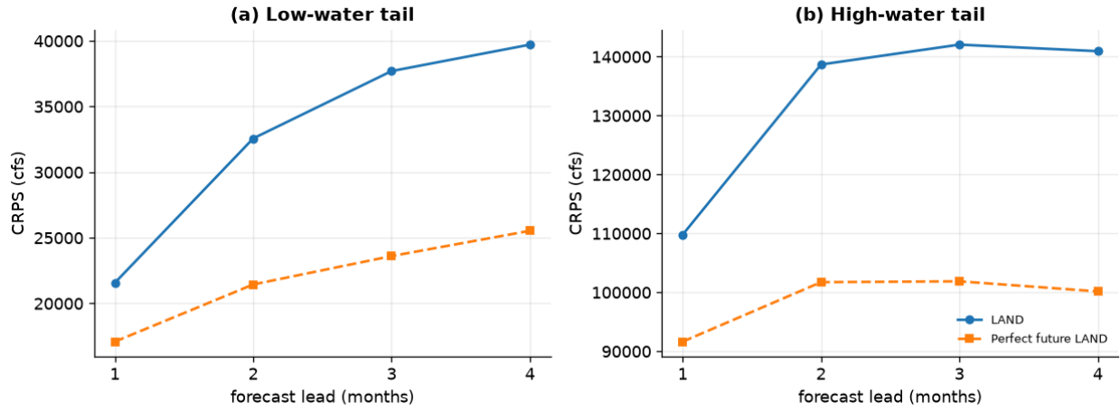
Figure 5. Low-water and high-water tails CRPS across leads 1-4 for operational LAND and perfect-future LAND. Lower CRPS indicates better probabilistic forecasts. Perfect-future LAND substantially reduces forecast error in both tails, with the gap between them increasing with lead.
