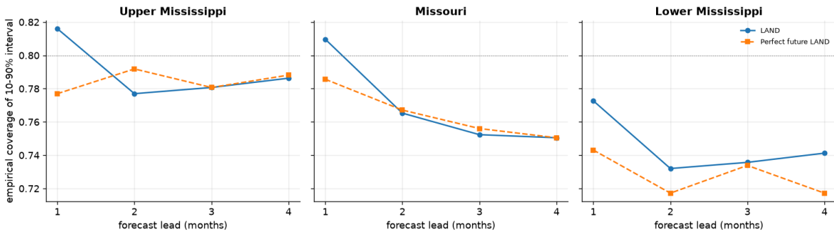
Figure S1. Empirical coverage of the 10-90% predictive interval at leads 1-4 for operational LAND and perfect-future LAND, shown by basin. The dotted line marks the nominal 0.80 coverage.
