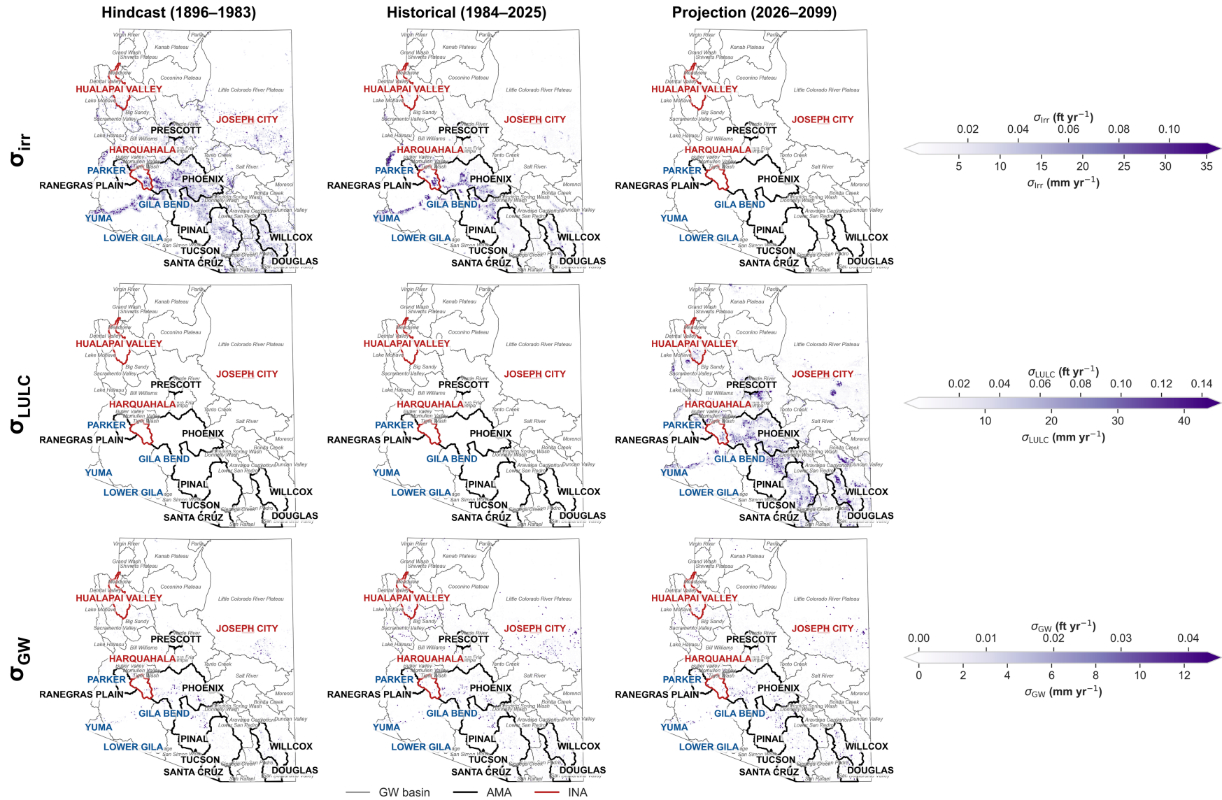
Fig. S3. As Fig. S2, for the management components: \sigma_{irr} (top; irrigated-area input, zero after 2025), \sigma_{LULC} (middle; land-use scenario spread, zero before 2026), and \sigma_{GW} (bottom; well-density input).
