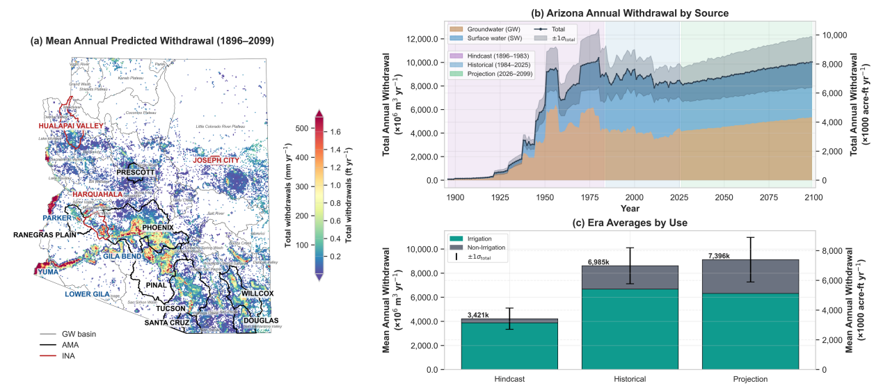
Fig 1. Dataset overview 28 . (a) Mean annual predicted withdrawal depth over 1896–2099, with groundwater basin boundaries and AMA/INA labels. (b) Statewide annual total withdrawal time series, including groundwater and surface water, with 1\sigma_{\text{total}} from the six-component uncertainty framework and era shading for the hindcast (1896–1983), historical (1984–2025), and projection (2026–2099) eras. (c) Era-average irrigation and non-irrigation withdrawal volumes with 1\sigma_{\text{total}} error bars. \sigma_{\text{total}} and the uncertainty framework are defined in Methods, Uncertainty quantification.
