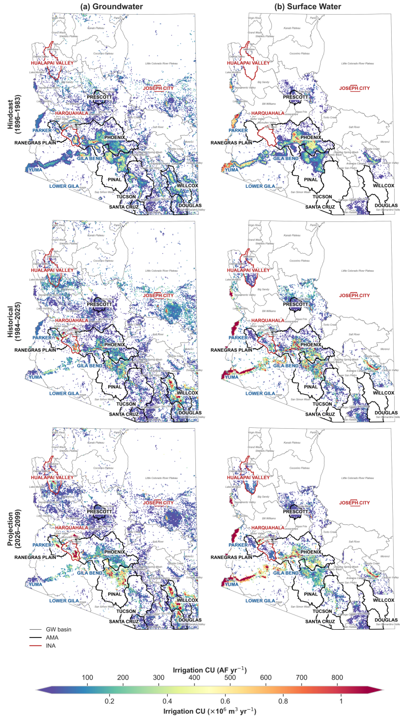
Fig 6. Era-mean annual irrigation consumptive use partitioned into (a) groundwater CU and (b) surface-water CU, with eras as rows (hindcast 1896–1983, historical 1984–2025, projection 2026–2099). The shared color bar shows consumptive-use volumes ( \text{m}^3 , bottom; AF, top).
