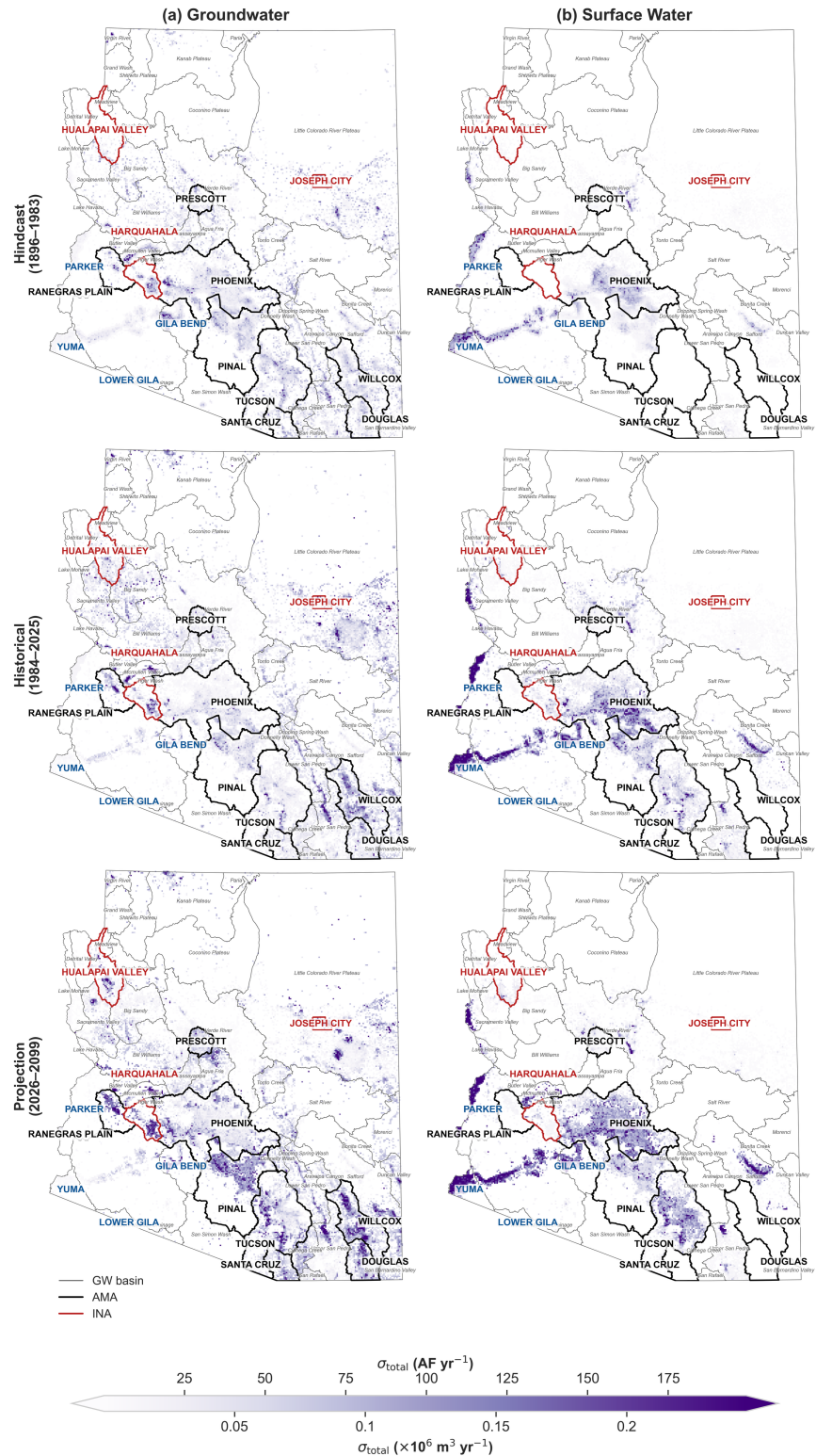
Fig 8. Era-mean annual \sigma_{\text{total}} (quadrature combination of the six uncertainty components) partitioned into (a) groundwater and (b) surface water, with eras as rows (hindcast 1896–1983, historical 1984–2025, projection 2026–2099). The shared color bar shows the per-pixel \sigma as volume ( \times 10^6 \text{ m}^3 , bottom; AF, top).
