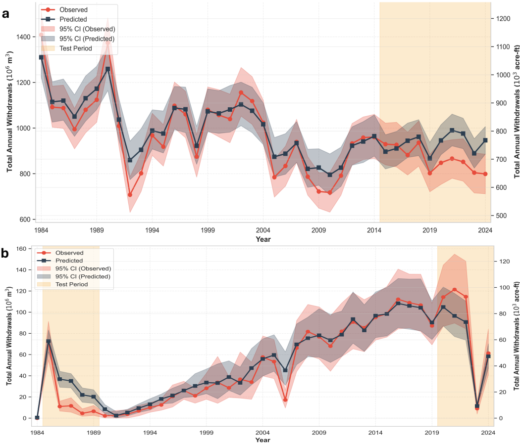
Fig 9. Held-out time series for the selected XGBRF model under two temporal holdout regimes and two management regimes. (a) Phoenix AMA, the largest GW-pumping basin, with mixed municipal and agricultural demand, under the T2 forward-extrapolation configuration (2015–2024 withheld from training). (b) Harquahala INA under the T5 dual-tail configuration (1985–1989 and 2020–2024 withheld simultaneously, forcing backward and forward extrapolation with no early- or late-record anchoring). Each panel shows the observed ADWR basin-summed metered total against the prediction, with the held-out periods shaded. The full per-basin panel sets for all eight temporal holdout configurations, and the seeded and unseeded spatial-LOO products are provided in the Zenodo repository 28 .
