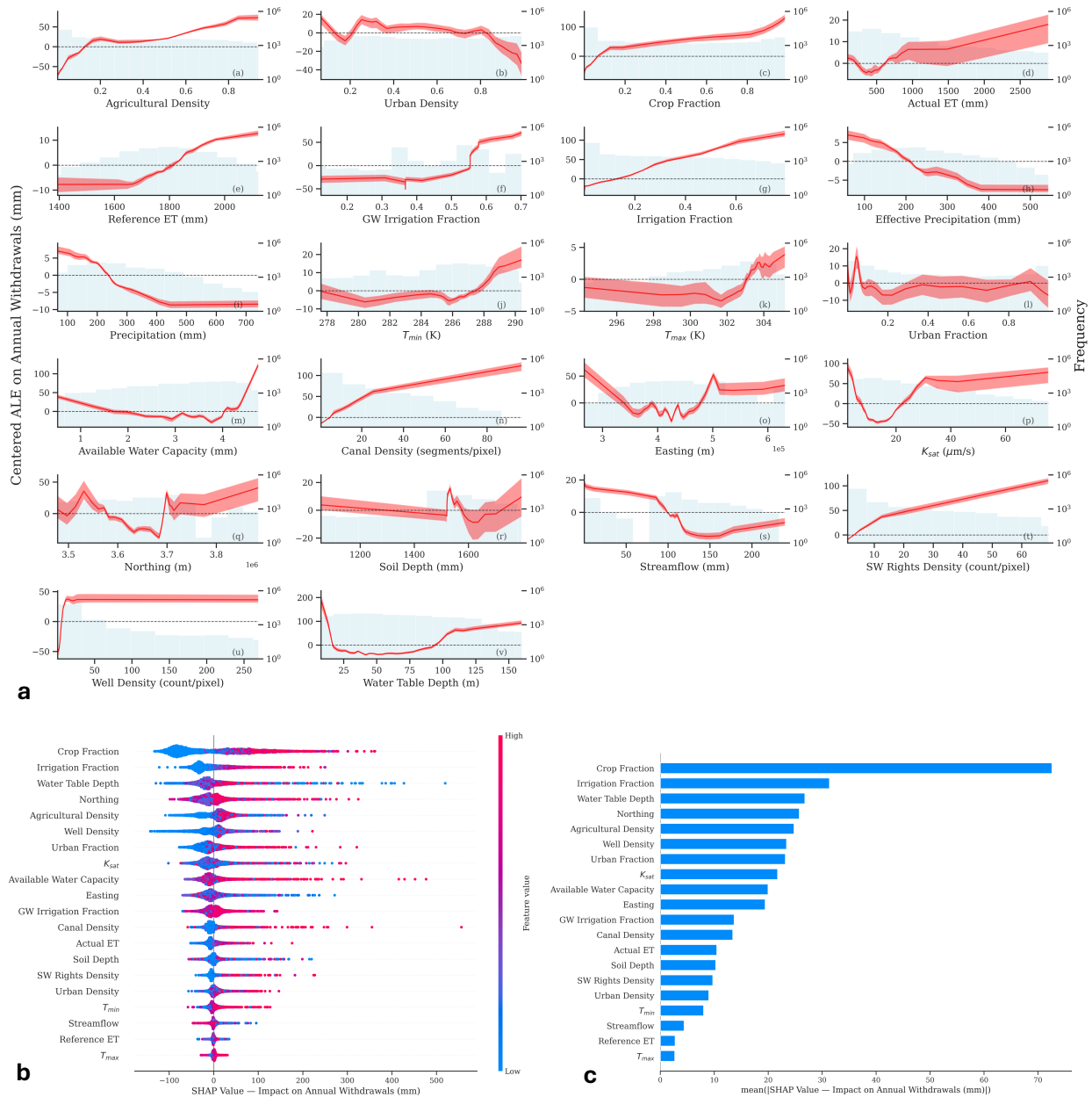
1125 Fig 10. Model interpretability for the selected XGBRF. (a) Accumulated local effects (ALE) on the 1126 training data, showing the marginal response of predicted withdrawal depth to each predictor. (b) SHAP 1127 summary (beeswarm): predictors ranked by (c) mean absolute SHAP value, each point one test sample 1128 colored by feature value, showing both the magnitude and the direction of each predictor's contribution. 1129 The permutation importances, per-era SHAP analyses, and per-feature SHAP dependence plots are 1130 provided in the Zenodo repository 28 .
