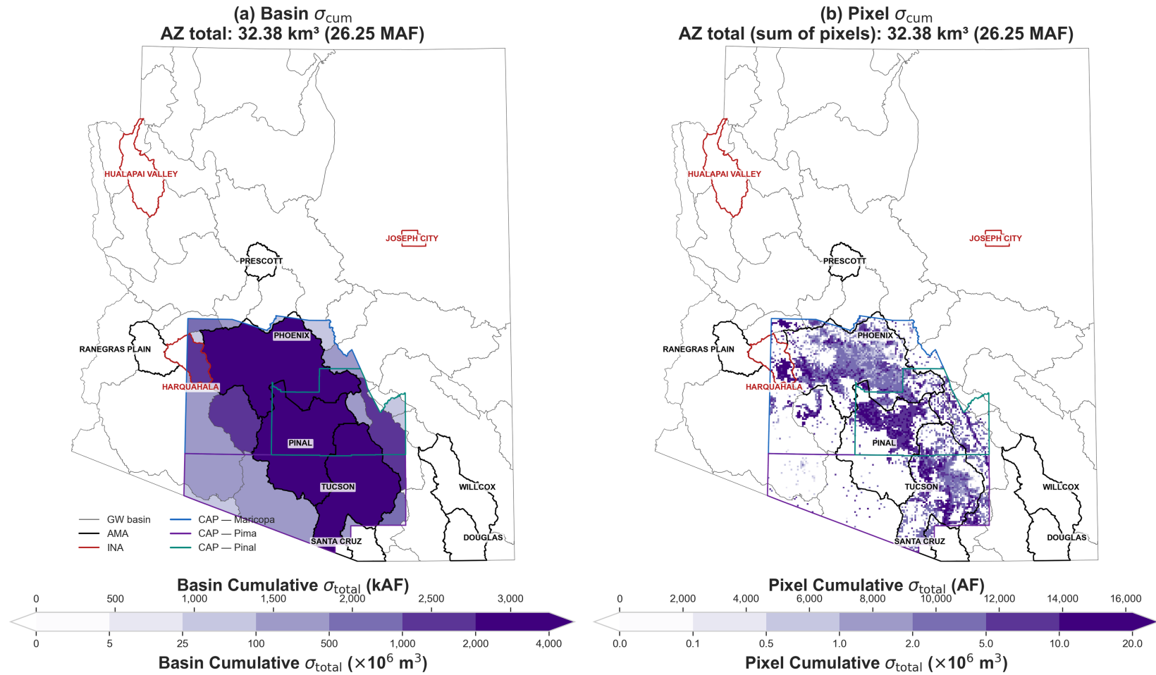
Fig. S9. Cumulative \sigma_{\text{total}} of groundwater withdrawal over the CAP service area, 2027–2099, (a) by basin and (b) by pixel. The CAP scenarios have no uncertainty ensemble of their own, so this central-run \sigma_{\text{total}} of TotalGW, restricted to CAP-service-area pixels and summed over the window, applies to every scenario (32.38 km 3 , or 26.25 MAF, statewide).
