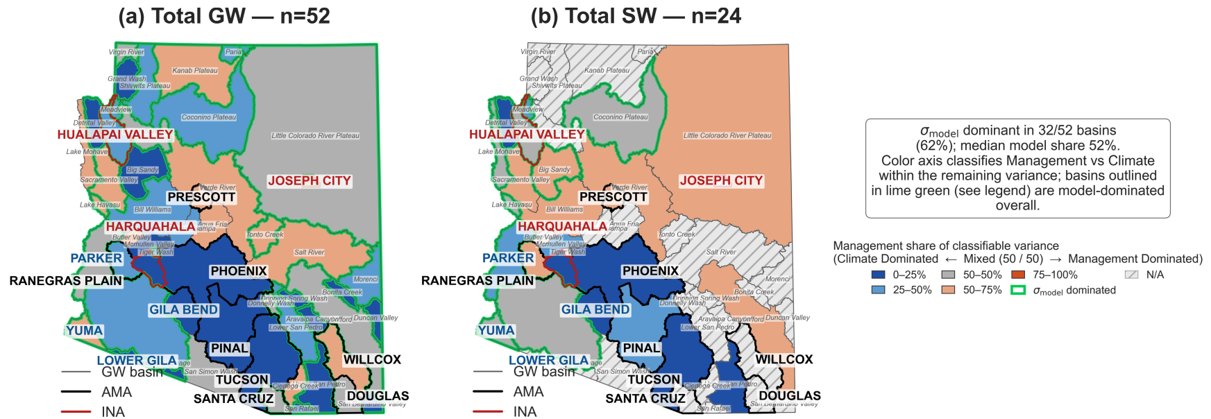
Fig. S5. Per-basin \sigma attribution of (a) total groundwater and (b) total surface-water withdrawal for the projection era (2026–2099), the withdrawal counterpart of the consumptive-use attribution in main-text Fig 3. Each basin is shaded by the management share of its management-plus-climate variance; basins where \sigma_{\text{model}} exceeds both classes are outlined in lime green, and hatched basins are not classified. Panel titles give the number of classified basins. The hindcast and historical maps and the per-year attribution series are in the Zenodo repository 1 .
