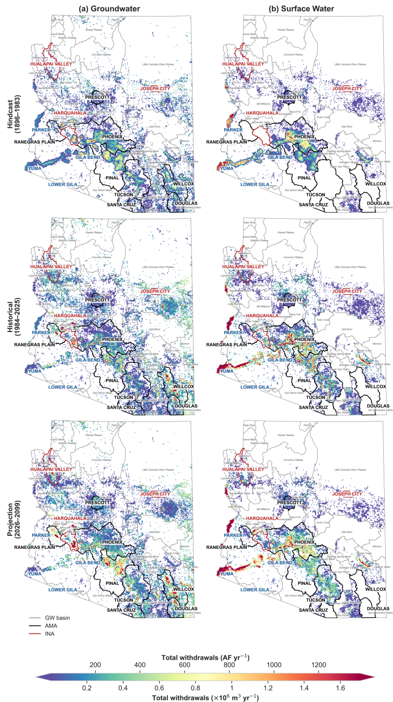
Fig 4. Era-mean partitioned annual withdrawal volumes. Columns are (a) total groundwater and (b) total surface water; rows are the hindcast (1896–1983), historical (1984–2025), and projection (2026–2099) eras, on a single shared volume scale. The groundwater maps concentrate in the alluvial AMA and INA basins, while the surface-water maps trace the SRP and CAP canal corridors and the Colorado River mainstem basins.
