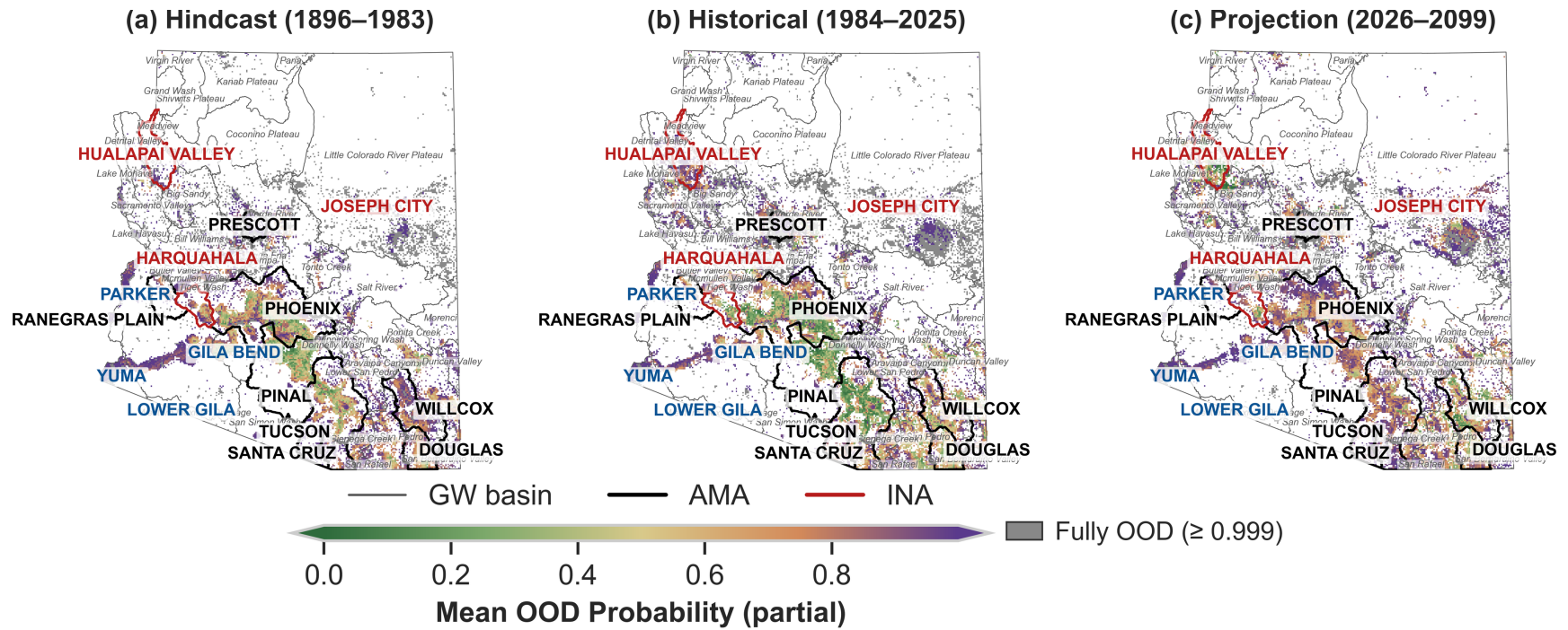
Fig. S6. Era-mean out-of-distribution (OOD) probability for the (a) hindcast, (b) historical, and (c) projection eras. The probability is the \chi^2(17) cumulative distribution of the squared Mahalanobis distance between a pixel's climate and land-use predictors and those of the training data (Methods, Out-of-distribution detection): 0 means in-distribution and values near 1 mean strong extrapolation. Gray pixels have an era-mean probability of at least 0.999.
