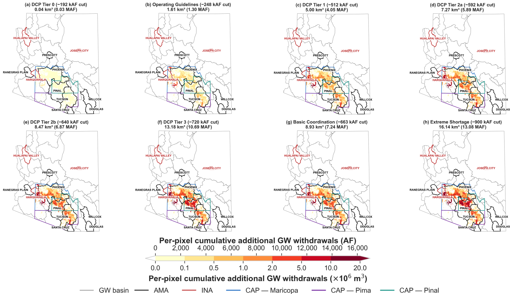
Fig. S8. Per-pixel cumulative additional annual GW pumping ( \Delta GW, AF per pixel) over 2027–2060 for the eight CAP shortage scenarios: (a) DCP Tier 0, (b) 2027–2028 Operating Guidelines 16 , (c)–(f) DCP Tiers 1, 2a, 2b, and 3, (g) WestWater Basic Coordination, and (h) WestWater Extreme Shortage. Panel titles give each scenario’s cut from the 900 kAF baseline delivery and the statewide total; the baseline, the cuts, and the pro-rata pixel distribution are as described for main-text Fig 5 and Table 12, which shows the 2027–2099 maps.
