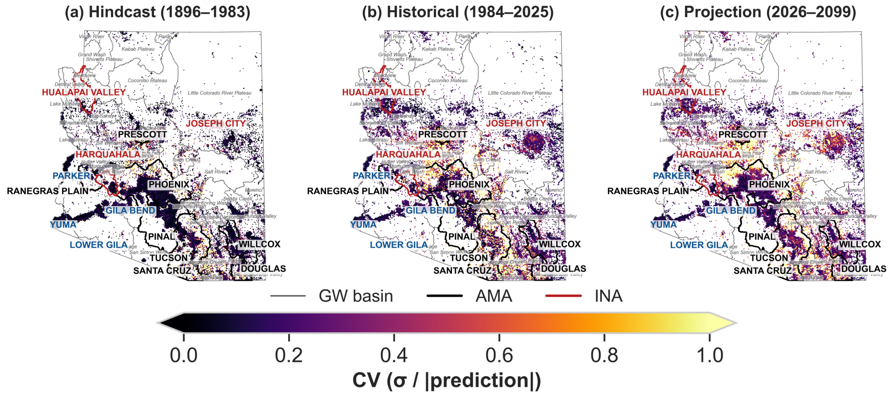
Fig. S4. Era-mean coefficient of variation ( CV = \sigma_{\text{total}} / |\text{prediction}| ) of annual total withdrawal for the (a) hindcast, (b) historical, and (c) projection eras. The color scale is capped at 1. The signal-to-noise ratio ( SNR = 1/CV ) is band 4 of every published raster 1 .
