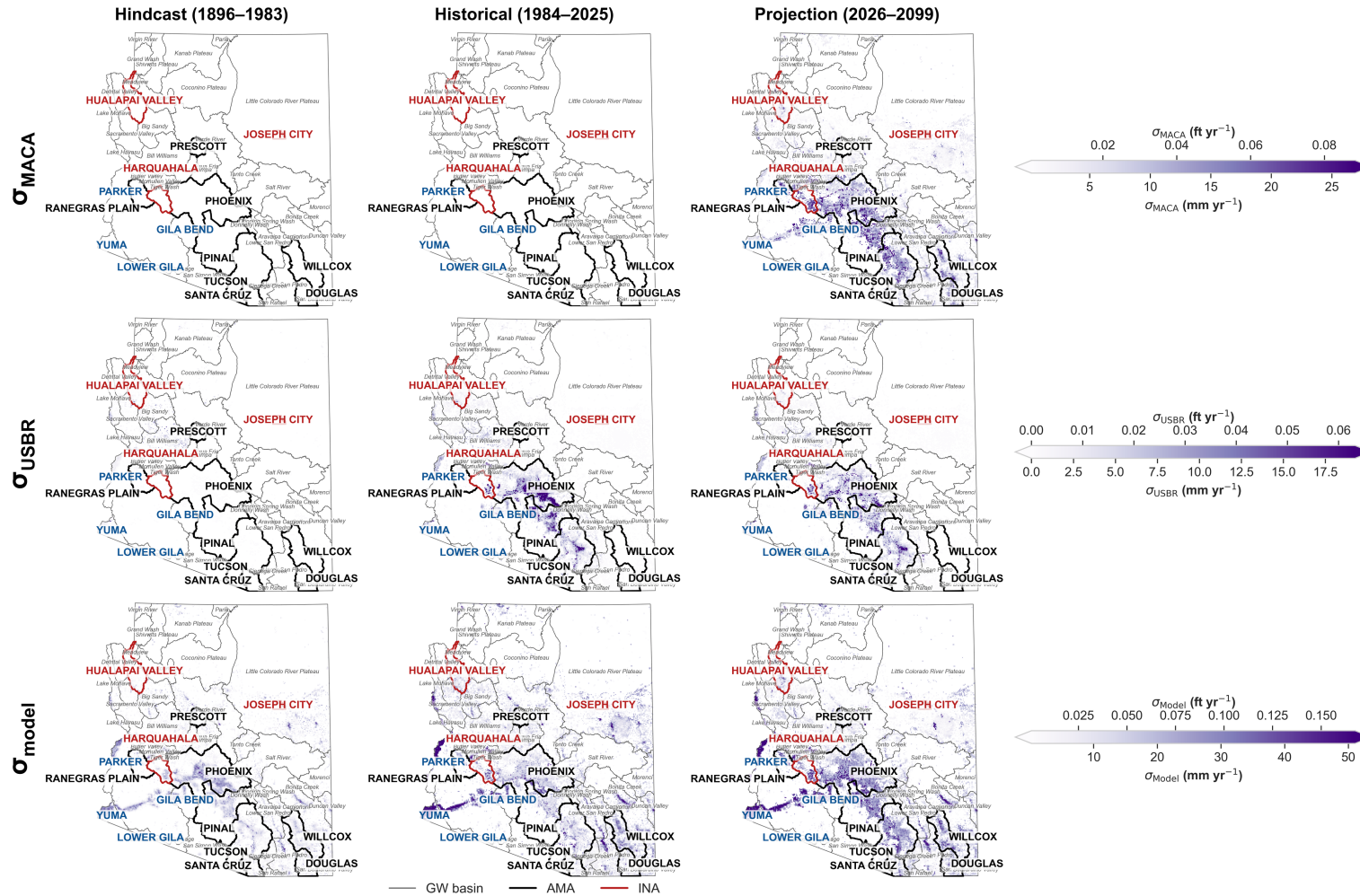
Fig. S2. Era-mean climate and model uncertainty components of annual total withdrawal depth, one per row: \sigma_{MACA} (top; downscaled-GCM spread, zero before 2026), \sigma_{USBR} (middle; Upper Colorado River streamflow spread, zero before 1950 and at CAP service-area pixels before 1985), and \sigma_{model} (bottom; ten-seed XGBRF ensemble), with the hindcast (1896–1983), historical (1984–2025), and projection (2026–2099) eras as columns. Each component has its own color scale ( \text{mm yr}^{-1} , bottom; \text{ft yr}^{-1} , top). The components are defined in Methods, Uncertainty quantification.
