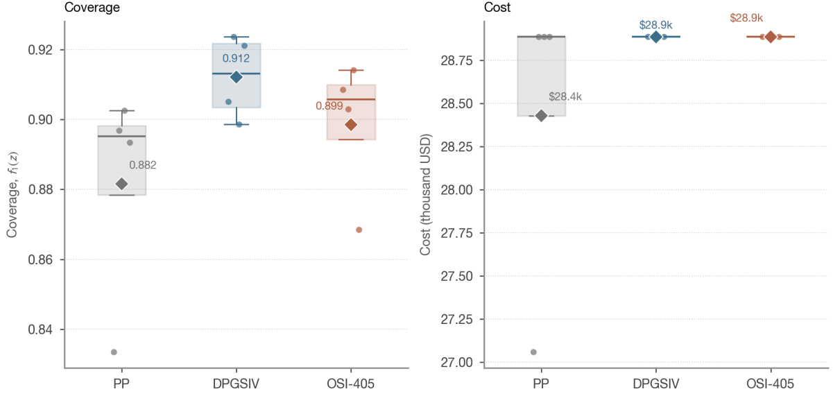
Fig. 12 Matched proposed-strategy performance by drift product. Boxes and whiskers summarise the four years complete in all three products (2018–2020 and 2023), points show annual values, and diamonds with direct labels mark means.
