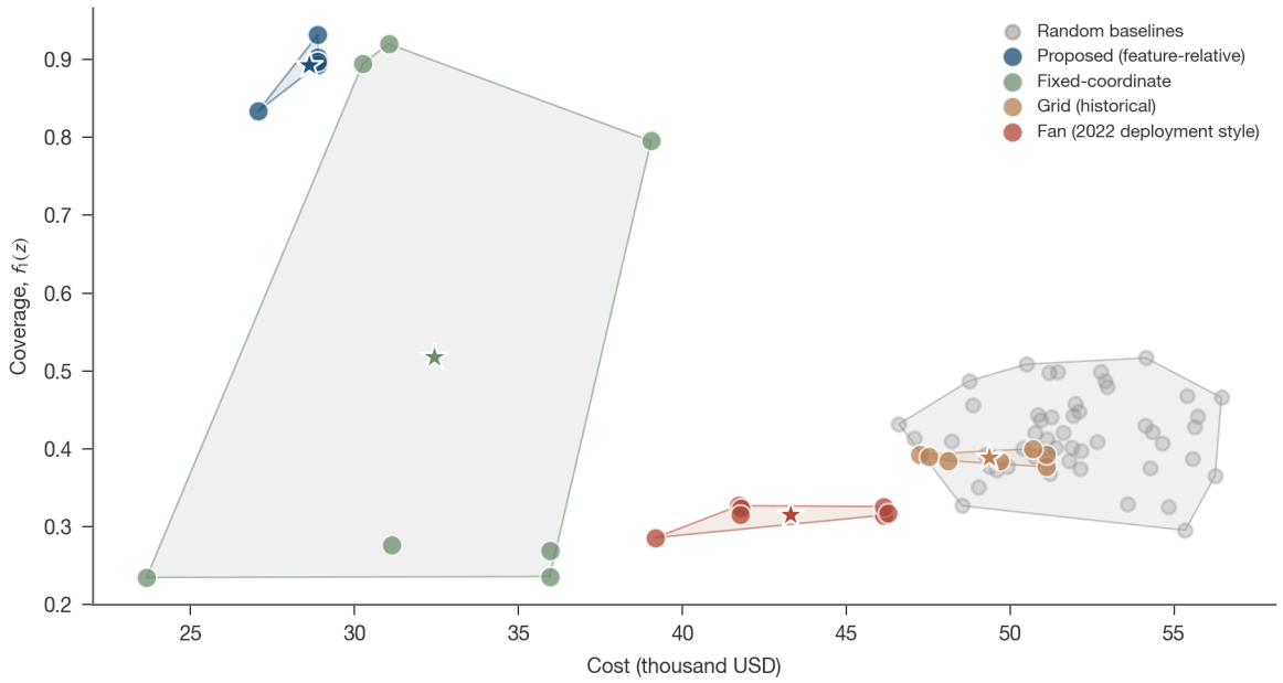
Fig. 8 Strategy comparison showing coverage and cost distributions across test years. The proposed feature-relative strategy (blue) achieves higher coverage with lower variance compared to fixed-coordinate (green), grid (orange), random (grey), and 2022-style fan (red) baselines. Coloured dots are individual test years, shaded polygons are the convex hull of each strategy’s points, and stars mark each strategy’s mean over the test years; the grey dots are the 50 random draws, each plotted at its own multi-year mean, of which the strongest is reported in Table 10.
