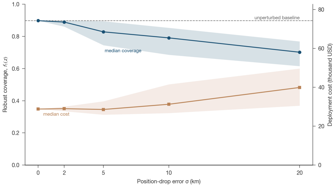
Fig. 10 Operational tolerance to buoy-drop position error. Median robust coverage (blue, left axis) and median deployment cost (orange, right axis) against Gaussian drop error; shaded bands show the 5th–95th percentile ranges across 50 paired perturbations per level.
