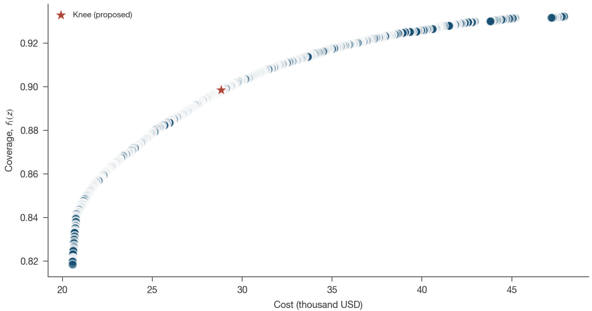
Fig. 3 Pareto front showing non-dominated solutions from robust multi-seed optimisation over 39 training years (300 individuals, 30 seeds, stopped at generations 228–400). The knee point (red star, ~$28.8k at a 39-year mean coverage of 0.898) is selected as the proposed strategy.
