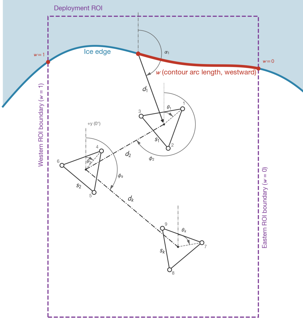
Fig. 2 Feature-relative genotype encoding. Cluster 1 selects a normalised east–west position w along the ice edge ( w = 0 at the eastern ROI boundary, matching the approach from Cape Town), anchors to the corresponding ice-edge point, and moves distance d_1 on heading \alpha_1 to the Cluster 1 centroid. Subsequent cluster centroids are chained by distance d_k on heading \varphi_k . All angular genes \alpha_1 , \theta_k and \varphi_k are measured clockwise from the grid +y axis of the analysis frame. Each cluster is an equilateral triangle with side length s_k ; vertices 1–3 denote buoy order.
