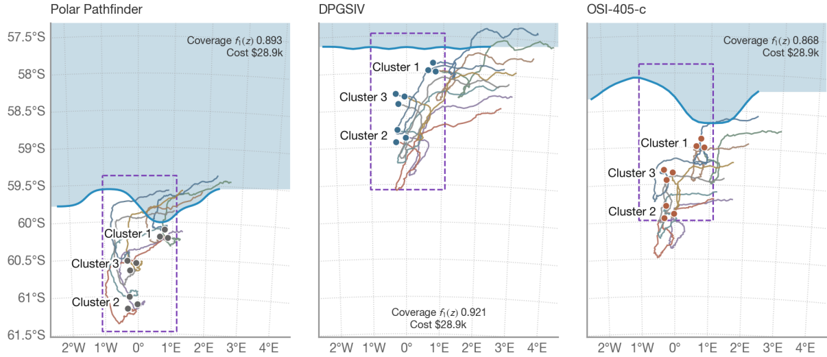
Fig. 11 Frozen feature-relative deployment transferred in 2023. The same PP-trained genes are decoded relative to each product's own feature boundary and then forced through that product's velocity field. Points mark initial positions, coloured lines show 14-day tracks, and each panel reports its own penalised coverage and cost, or the eligibility failure where the product cannot support the required fraction of the array.
