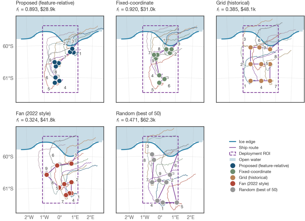
Fig. 7 Example deployment geometries for 2023. Each panel shows initial buoy positions (numbered), simulated 14-day drift tracks, the ice edge, deployment ROI, and optimised ship route for one baseline strategy; the random panel shows the strongest of 50 uniform draws of nine valid ice cells (no DKA cluster constraints). The annotated coverage and cost are those recorded for 2023 in the run’s baseline artifact, so they are directly comparable with Table 10.
