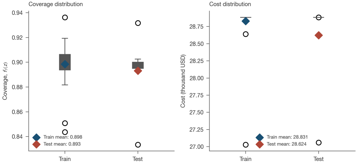
Fig. 6 Training vs. testing boxplots showing coverage and cost distributions across the 39 training and 7 test years; diamonds mark the training (blue) and test (red) means and open circles are outlying years. Test years cluster around the training median (99.4% retention), with 2018 visible as the low test-year outlier; cost is identical in every year except those in which a cluster centroid is clipped at the ROI boundary.
