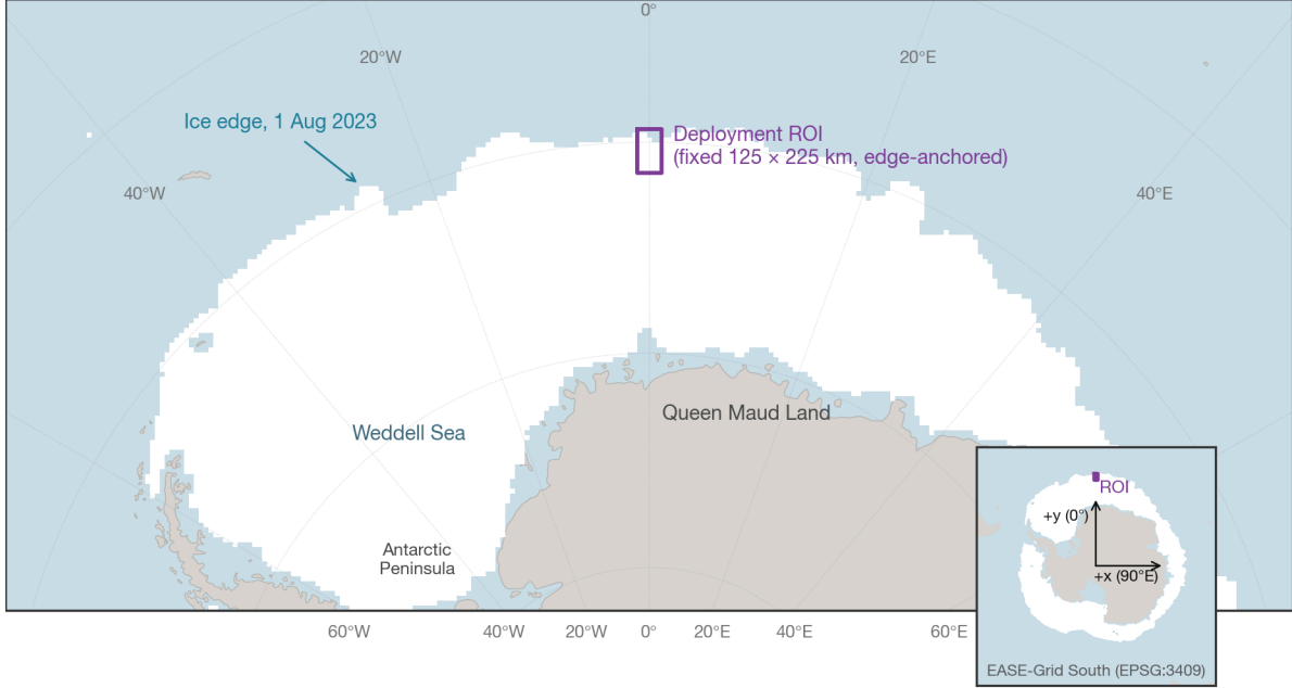
Fig. 1 Study region and valid Polar Pathfinder ice-motion support on 1 August 2023 (white, on a light-blue ocean), with the deployment ROI (purple): a fixed 125 \times 225 km rectangle in the analysis frame, with its eastern side on the line x = 64 km (close to 1^\circ\text{E} ) and its top 20 km north of the year’s most northerly ice-edge point within the rectangle’s width. Arrows in the inset give the axes of the EASE-Grid South analysis frame from its origin at the South Pole: +x points towards 90^\circ\text{E} and +y towards 0^\circ , so on this map x increases eastward and y increases northward near the ROI. The inset locates the ROI relative to the Antarctic continent on the full Southern Hemisphere domain.
