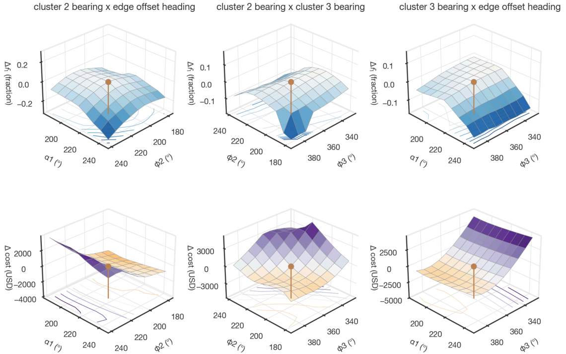
Fig. 9 Pairwise 3D local response surfaces for \varphi_2 \times \alpha_1 , \varphi_2 \times \varphi_3 , and \varphi_3 \times \alpha_1 on 9 by 9 grids; coverage (top row) and cost in USD (bottom row). Each diverging scale is centred at zero, the orange marker is the unperturbed strategy, the base plane shows the projected contour, and each panel is viewed from the surface’s low side so the height field never occludes itself.
