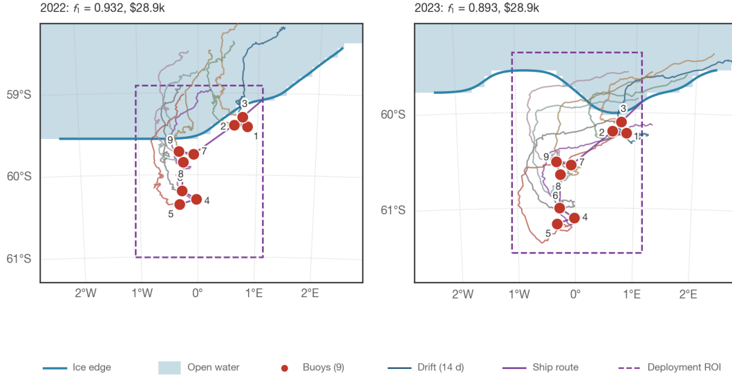
Fig. 5 Proposed strategy deployment for two held-out years. One frozen feature-relative genotype is decoded against the 2022 (left) and 2023 (right) ice edges, with deployed positions (markers), 14-day simulated drift trajectories (tracks), and the optimised ship route (solid violet) shown relative to that year’s ice edge and pack ice.
