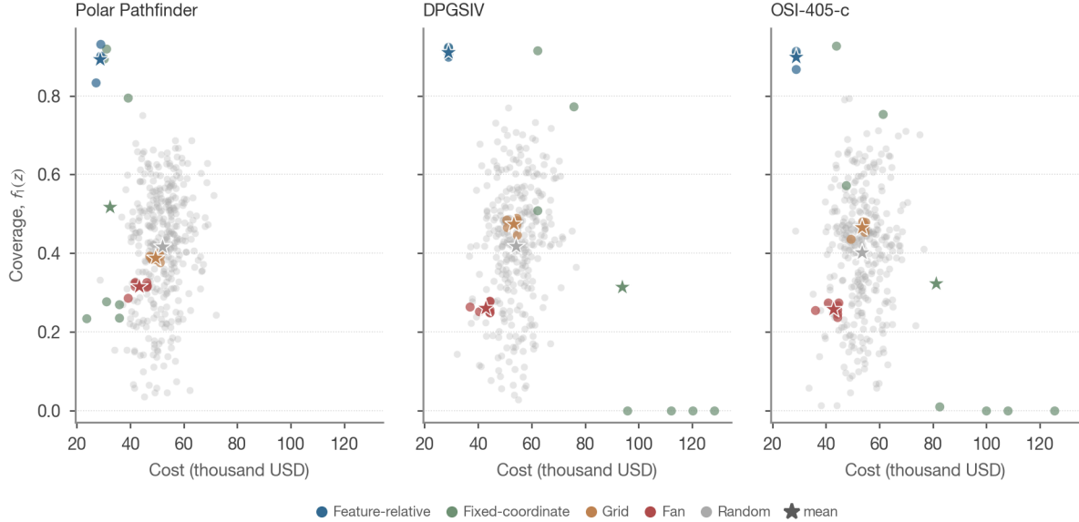
Fig. 13 Coverage–cost comparison for PP, DPGSIV, and OSI-405-c. Colour identifies strategy within each panel; circles are eligible annual or random evaluations and stars mark means. Only evaluations satisfying the product-specific support rules are included.
