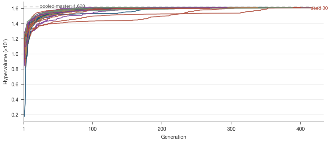
Fig. 4 Hypervolume convergence across the 30 independent seeds. Each line is the dominated coverage \times cost volume of the seed’s running non-dominated front versus optimisation generation, ending at the generation where the seed’s stagnation budget was exhausted or at the 400-generation ceiling; the dashed reference is the pooled master front after the local search. The flattening curves indicate the search has saturated and further generations of a single seed yield no improvement.
