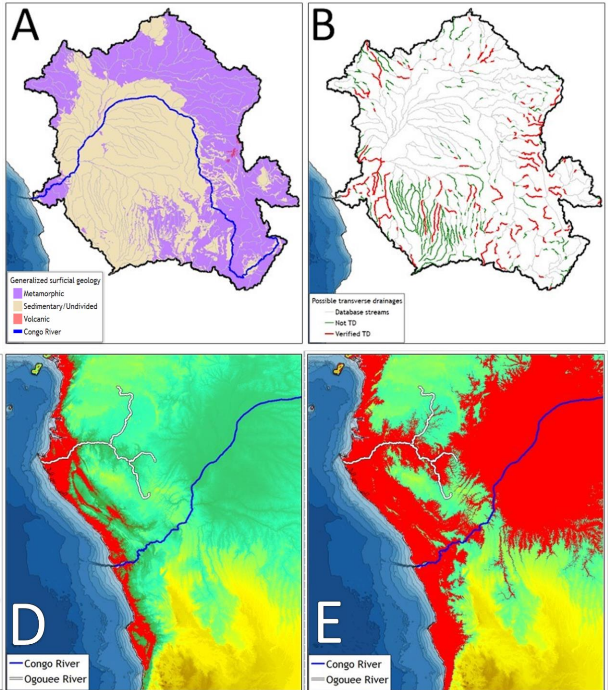
Figure 8. (A–E) Congo basin overview. (A) Simplified geologic map. (B) Locations of possible transverse drainages from database: visually verified TDs in red, negative identifications in green. (C) TDs in adjacent basins; database TDs as solid red lines, non-database transverse streams as dashed red lines. (D) HydroSHEDS DEM with elevations <150 shaded red, showing the oversized delta of the Ogooué and the Congo watersheds. (E) HydroSHEDS DEM with elevations <500m shaded red, illustrating the wind gap between the Ogooué and the Congo watersheds, as well as the narrowness of the Congo in its current channel.
