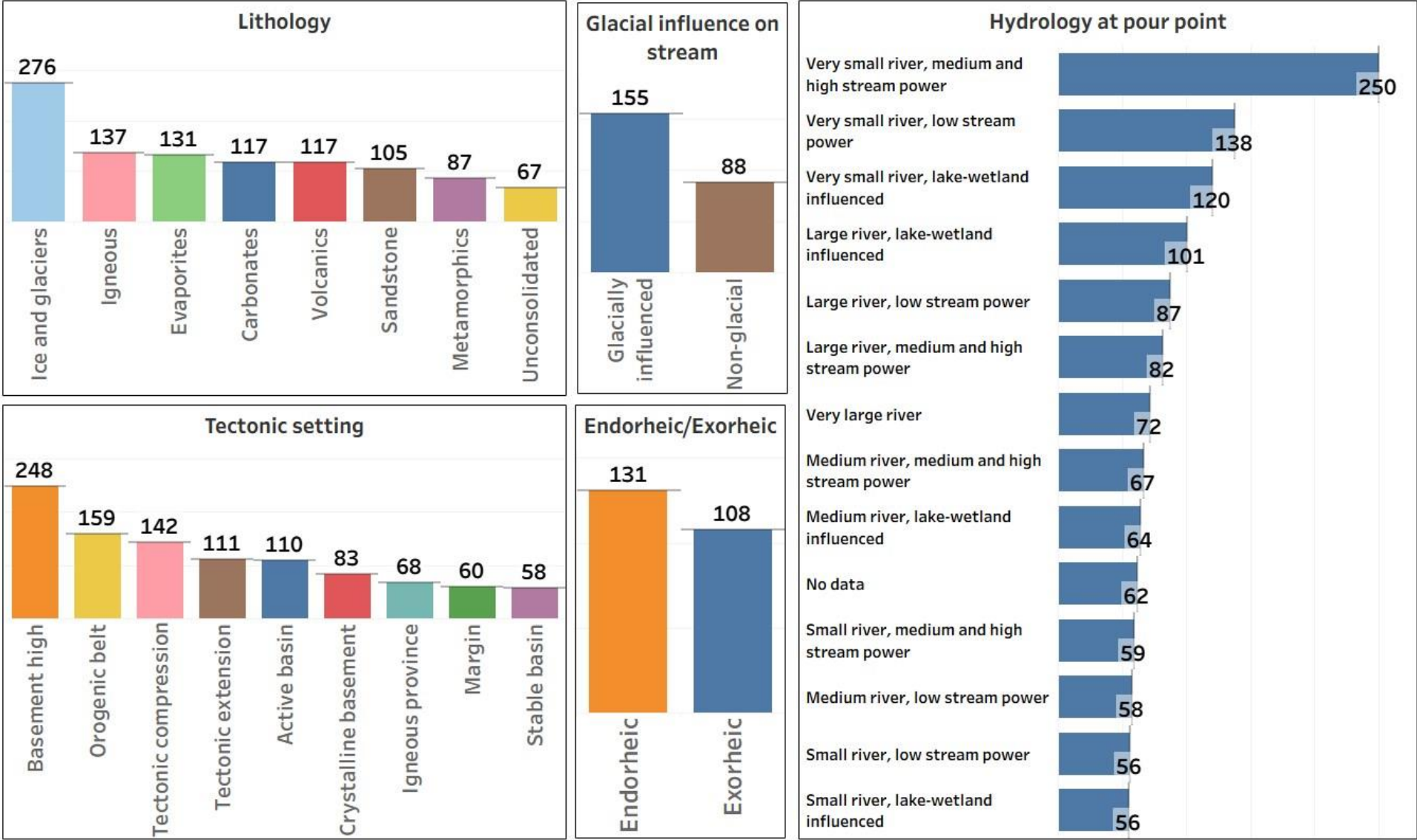
Figure 6A-E. Average maximum depth of verified TD reaches by attribute. Clockwise from top left: Lithology, Glacial influence, Stream hydrology at pour points, Endorheic vs exorheic, Tectonic setting.
