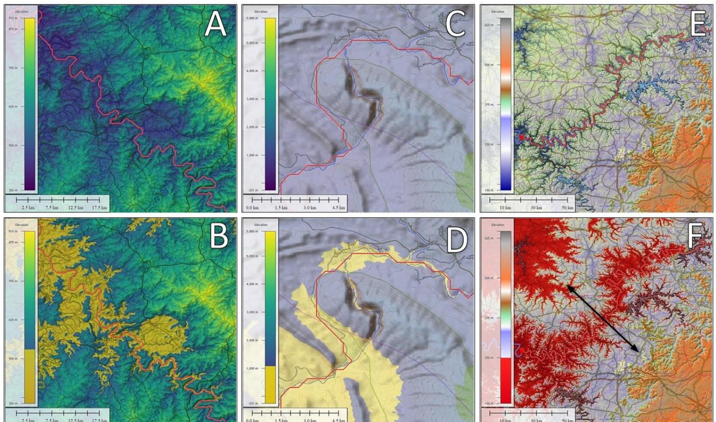
Figure 7A-F. TDs (red lines) on the Rio Chopim (Brazil), Qara Aghaj (Iran) and Cumberland River (Kentucky, United States). (A) Rio Chopim flowing northwest to its junction with the Iguazu River. (B) Rio Chopim TD, elevations below 530 m shaded yellow, showing the path of the river flowing into a meteor blume and then out across a ridge. (C) A portion of the TD of the Qarah Aghaj. The actual river flows through the narrow canyon in the anticline nose, but the HydroSHEDS stream in red passes around the nose because the channel was too narrow to be captured by the resolution of the DEM from which the streamline was generated. (D) Qara Aghaj, elevations below 1080 m shaded yellow, illustrating contour constriction upstream of the gap. (E) Cumberland River flowing from Kentucky into Tennessee. (F) Cumberland River, elevations below 250 m shaded red, showing the river breaching the Cincinnati Arch (arrow).
