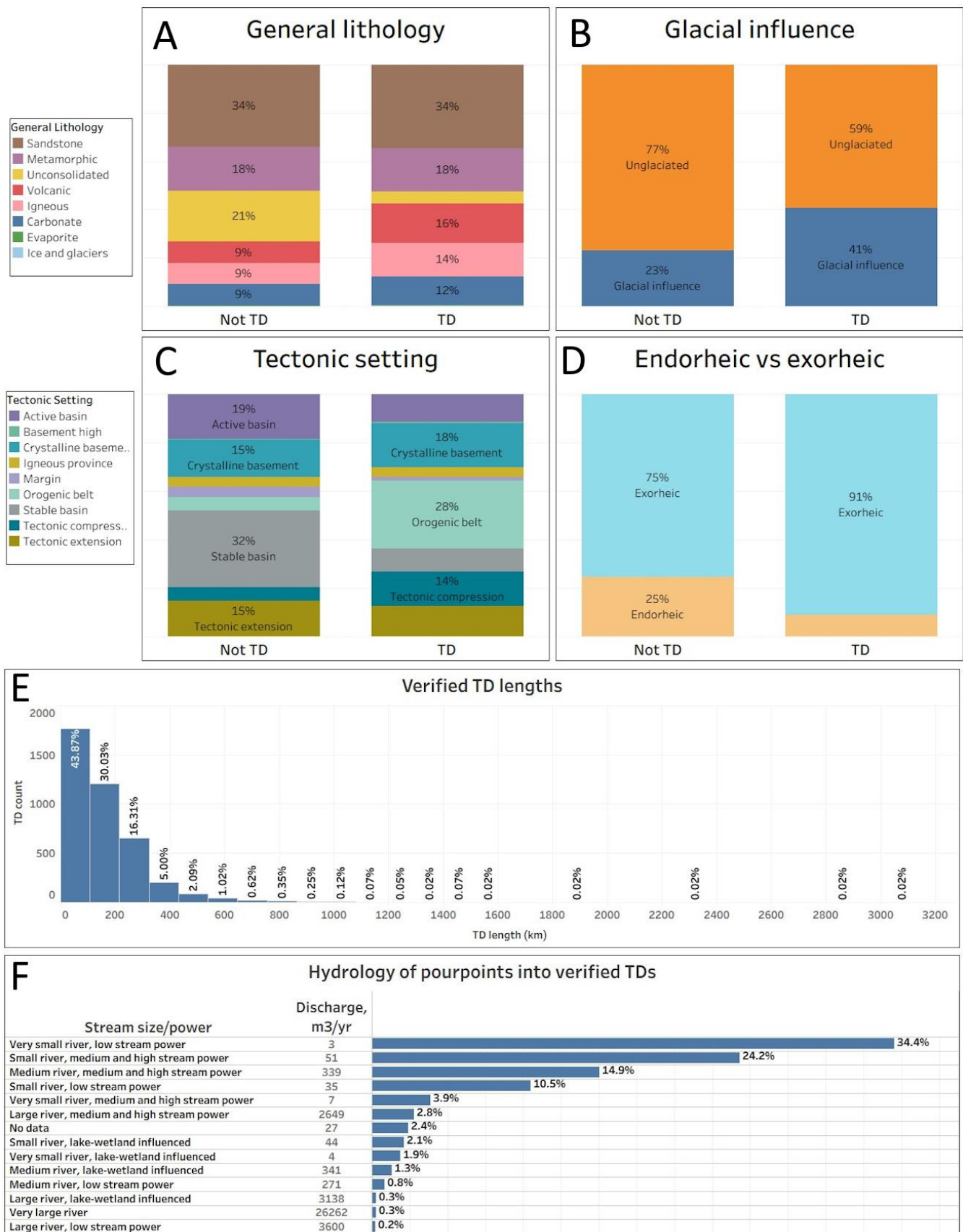
Figure 5A-F. (A-D) Comparison of TD vs non-TD attributes: A) Lithology of the maximum elevation of the reach; B) Distribution on glacially influenced streams; C) Tectonic setting; D) Percentage of exorheic vs endorheic streams. (E) Distribution of TD lengths. (F) Distribution of stream size and stream power at TD pour points.
