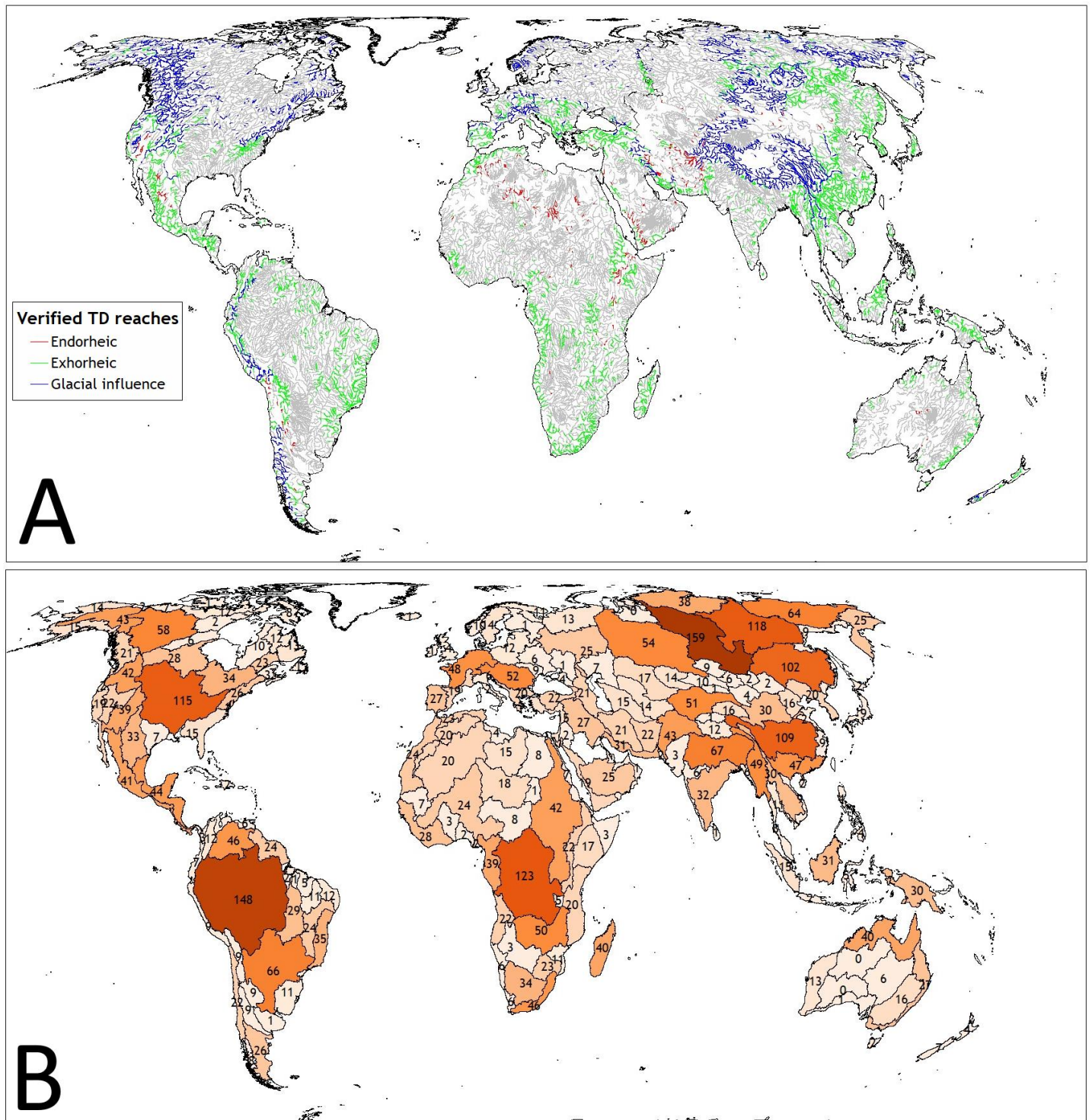
Figure 4A-B. (A) All visually verified TDs. Global river dataset in grey, glacially influenced TDs in blue, unglaciated exorheic TDs in green, unglaciated endorheic TDs in red. (B) Watershed basins shaded by TD density.
