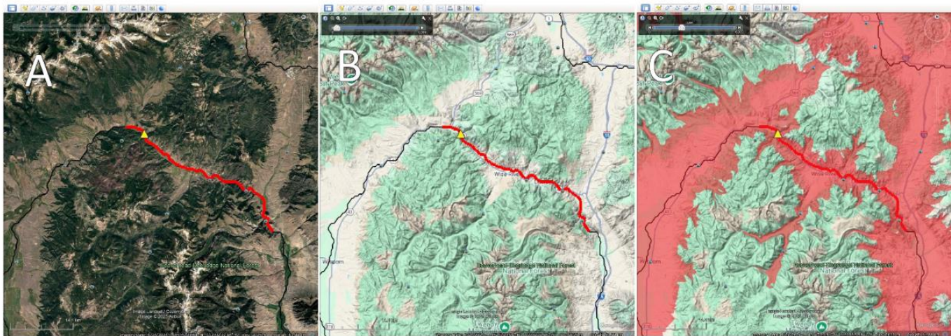
Figure 3. (A) Google Earth view of the TD of the Big Hole River through the Pioneer Mountains of Montana, US. Yellow triangle indicates pour point into the TD. (B) Same view with Google Maps Terrain overlay enabled. (C) Google Maps Terrain overlay with Sea Level Rise slider set to approximately 2000 m ASL, delineating more clearly the lower elevation terrain upstream of the TD.
