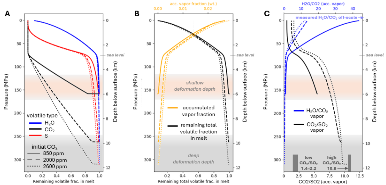
Figure S.7: Sulfur_X open-system isothermal degassing model for a Shishaldin basaltic melt using the CO 2 -H 2 O degassing model of Iacono-Marziano et al. (2012). Model conditions and figure symbology are the same as in Figs. 9 and 10 in the main text. Panel C shows CO 2 /SO 2 and H 2 O/CO 2 ratios of accumulated gas during open-system degassing behavior (compare to Fig. 10 of the main text, which shows instantaneous gas ratios for each pressure step). Airborne-measured gas compositions shown as bars along the bottom and top axes, with the measured H 2 O/CO 2 ratio being off-scale (see Table 2). Depth below the surface assumes a crustal rock density of 2700 kg/m 3 . Horizontal shaded regions indicate the approximate depth of the Shishaldin deformation sources (i.e., possible magma reservoirs) from Angarita et al. (this issue).
