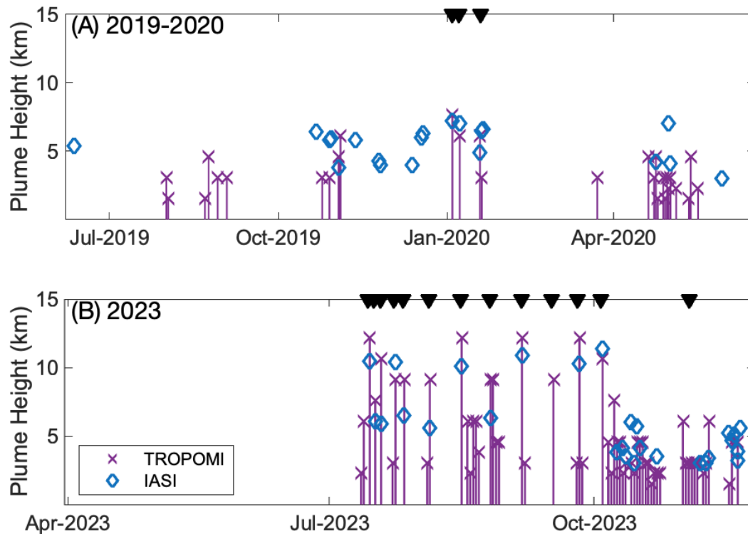
Figure S.1: Timeseries comparison between SO 2 plume heights derived from TROPOMI (purple) and IASI (blue) for the 2019-2020 (a) and 2023 (b) eruptions of Shishaldin Volcano. Black triangles on the upper x-axis mark explosive events (paroxysms).
