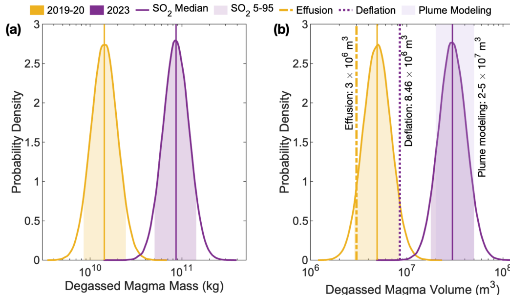
Figure 11: Results from the Monte Carlo simulation of cumulative degassed magma masses (a) and volumes (b) for 2019–2020 (yellow) and 2023 (purple) eruptions of Shishaldin Volcano. Median values are presented as vertical solid lines while 5-95 th percentile regions are shown as shaded regions. Degassed magma volumes are plotted in comparison to the 2019–2020 effusive volume (dot-dashed yellow line, Angarita et al., this issue), the modeled 2023 syn-eruptive deflation volume (dotted purple line; Angarita et al., this issue) and plume-modeling derived eruption volume (light purple shaded region; Mota et al, this issue).
