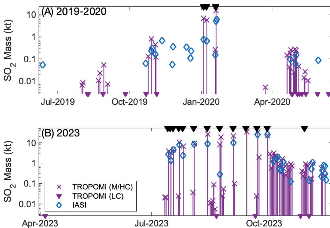
Figure 6: Time series observations of TROPOMI and IASI Shishaldin Volcano SO 2 detections and masses for the 2019–2020 (A) and 2023 (B) eruptive periods.
