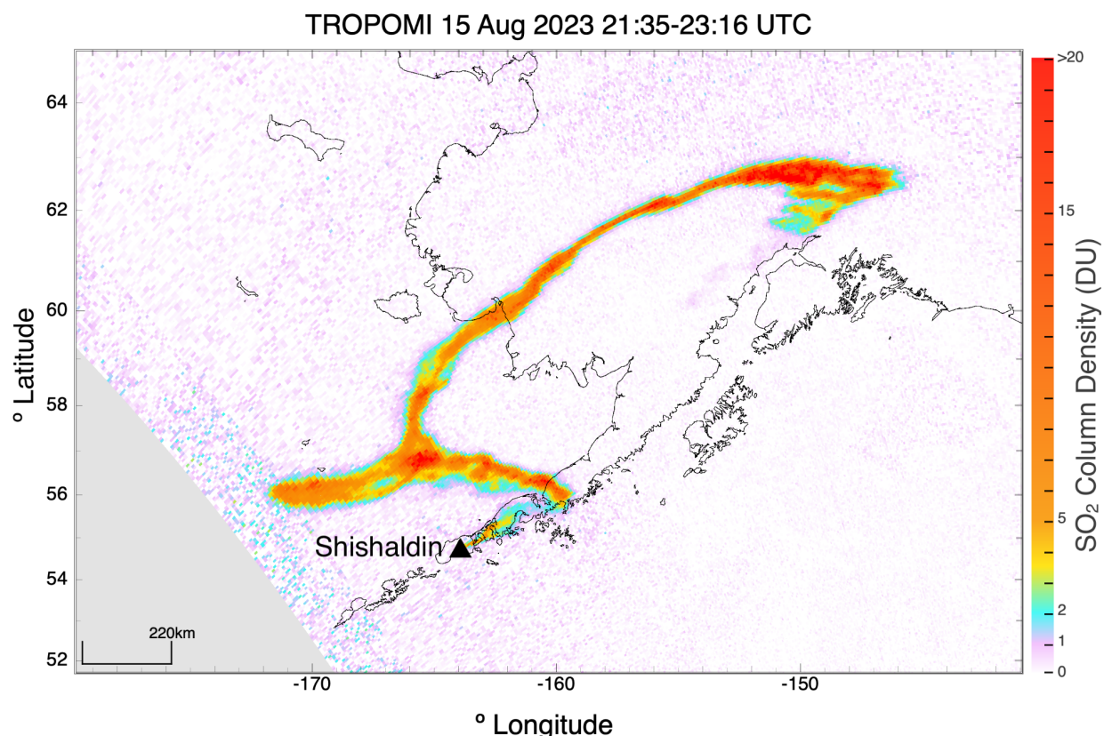
Figure 1: TROPOMI image acquired on 15 August 2023 at 21:35 UTC depicting the \text{SO}_2 plume produced during Event 7 of the 2023 eruption of Shishaldin Volcano (labeled triangle). This detection produced an \text{SO}_2 mass of 25.9 kt and a time-averaged emission rate of \sim 57,700 t/d. The color bar scale shows the \text{SO}_2 column density in Dobson Units (DU) based on the 7 km TROPOMI altitude product.
