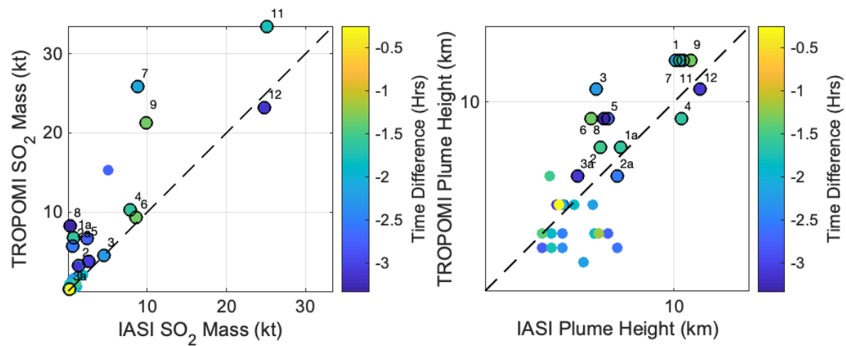
Figure S.2: Comparison between coincident IASI and TROPOMI Shishaldin SO 2 masses (left) and plume heights (right) throughout 2019–2020 and 2023 eruptive episodes as a function the time difference between TROPOMI and IASI overpass times in hours. Dashed black lines indicate a 1:1 agreement. All detections associated with paroxysmal events are labeled, with the 2019–2020 eruption events distinguished as “a”.
