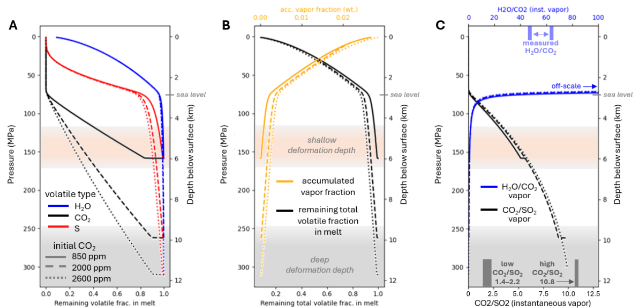
Figure 10: Sulfur_X open-system isothermal degassing model for a Shishaldin Volcano basaltic melt. Model conditions and figure symbology are the same as in Fig. 9. Panel C shows CO 2 /SO 2 and H 2 O/CO 2 ratios of gas released instantaneously during each pressure-step of open-system degassing (total accumulated gas ratios are shown in Fig. S.6). Note that for pressures less than 70 MPa, modeled instantaneously exsolved H 2 O/CO 2 ratios substantially exceed 100 and are not plotted here to improve readability. Airborne-measured gas compositions shown as bars along the bottom and top axes (see Table 2). Complete results can be found in Tables S.10-12.
