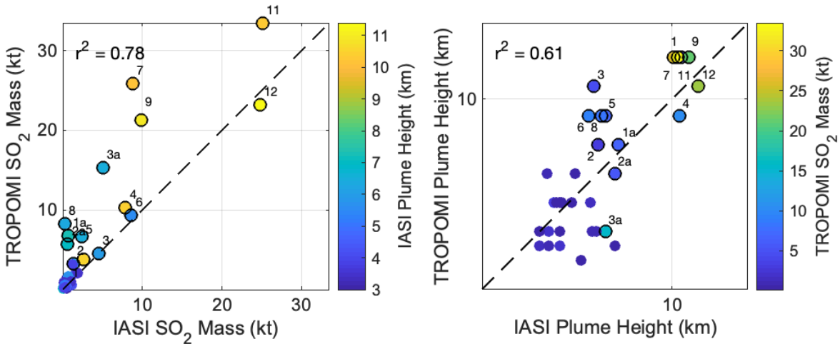
Figure 7: Comparison between coincident IASI and TROPOMI Shishaldin Volcano SO 2 masses (left) and plume heights (right) throughout 2019–2020 and 2023 eruptive episodes. Symbol colors reflect IASI plume height in km (left) and TROPOMI SO 2 mass in kt (right). Dashed black lines indicate a 1:1 agreement. All detections associated with paroxysmal events are labeled, with the 2019–2020 eruption events distinguished as “a”.
