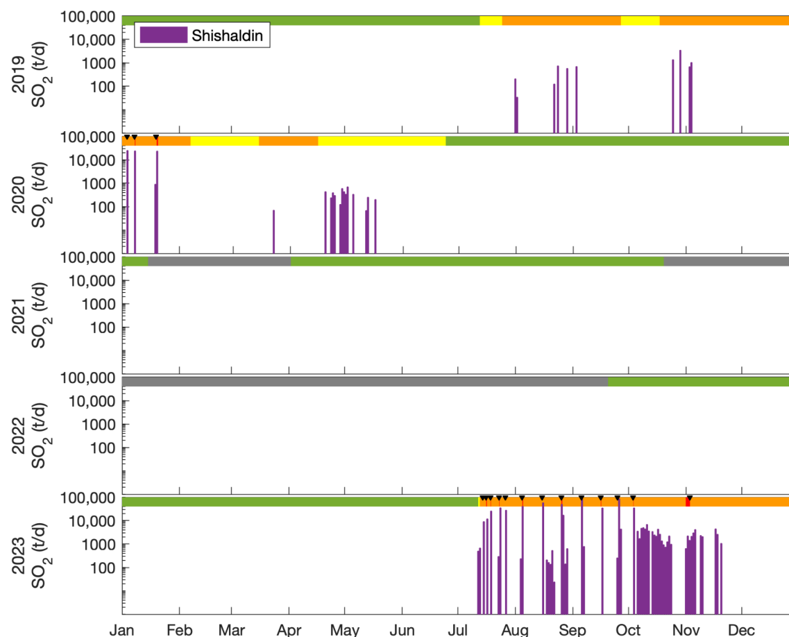
Figure 5: Five years of TROPOMI derived SO 2 emission rates (purple bars) from 2019 (top) through 2023 (bottom) plotted on a logarithmic scale. AVO's Aviation Color Code is plotted on the top of each figure reflecting AVO's public notices about volcano status, which we use here as a proxy for volcanic activity, acknowledging that this by nature sometimes lags volcanic activity. Here green represents background activity, yellow indicates above background activity, orange indicates an eruption is underway or imminent, red indicates that a substantial explosive eruption is underway or imminent, and gray indicates the monitoring network is impaired such that activity cannot be accurately characterized. Black triangles on the top of each figure mark major explosive events as identified by AVO (Loewen et al., 2026).
