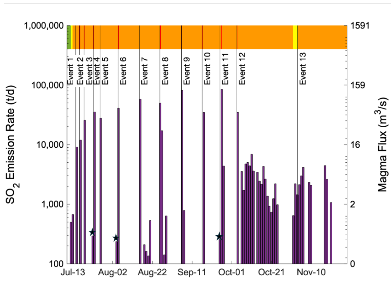
Figure 8: TROPOMI derived \text{SO}_2 emission rates (purple bars, left axis) and equivalent magma fluxes calculated from equation 2 (right axis) observed for the 2023 eruption and plotted on a log scale. Shishaldin Volcano's Aviation Color Code is plotted at the top as a proxy of volcanic activity. Each explosive event is marked by a vertical black line. Black stars indicate pre-paroxysmal degassing. Note that emissions from Event 13
