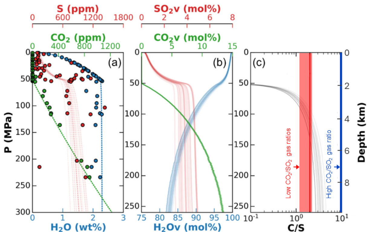
Figure S.6: Empirical degassing model fit to measured volatiles in melt inclusions from Shishaldin's 1999 eruption. A) Volatile concentrations measured in melt inclusions (circles) and the empirical degassing model result for remaining volatile species in the melt during magma ascent (curves). B) Modeled composition of the co-existing exsolving vapor during magma ascent. C) Modeled C/S ratios in the exsolved vapor, with ranges of low- and high-C/S gas measurements at Shishaldin indicated (red and blue bands, respectively). Initial volatile concentrations (2.3 wt% H 2 O, 1300 ppm CO 2 ) are based on analyses of primitive melt inclusions from the 1999 eruption (Rasmussen et al. 2018), and are similar to those presented in Figures 9 and 10 in the main text. Remaining S concentration in the melt is modeled and based on a K 2 O-SO 2 regression of measured values (see Werner et al., 2020). Depth below the surface assumes a crustal rock density of 2700 kg/m 3 .
