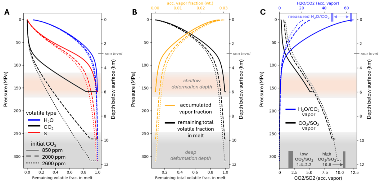
Figure 9: Sulfur_X closed-system isothermal degassing model for a Shishaldin Volcano basaltic melt (assuming 1120°C, f_{O_2} = \Delta FQM + 0.9 , S^{6+}/S^{total} 0.3–0.4) using the CO 2 -H 2 O degassing model of Iacono-Marziano et al. (2012). The modeled melt initially contains 1710 ppm S and 2.5 wt% H 2 O, and three different initial CO 2 concentrations are modeled: 850, 2000, and 2600 ppm (respectively solid, long dashed, and dotted lines across all panels). A) Fraction of S (red), CO 2 (black) and H 2 O (blue) remaining dissolved in the melt as magma ascends. B) Total volatile mass fraction remaining in the melt (black) and partitioned into an accumulated exsolved volatile phase (yellow). C) H 2 O/CO 2 (blue) and CO 2 /SO 2 (black) compositions of the accumulated exsolved vapor phase, with airborne-measured CO 2 /SO 2 and H 2 O/CO 2 gas compositions shown as bars along the bottom and top axes (see Table 2). Depth below the surface assumes a crustal rock density of 2700 kg/m 3 . Horizontal shaded regions indicate the approximate depth of the Shishaldin Volcano deformation sources (possible magma reservoirs) from Angarita et al. (this issue). See text and Tables S7-9 for further details.
