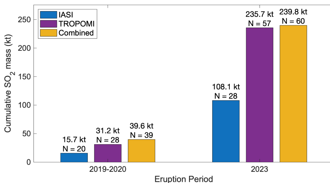
Figure S.4: Bar diagrams for the 2019–2020 (left) and 2023 (right) Shishaldin Volcano eruptions showing cumulative eruptive SO 2 mass determined from IASI only (blue), TROPOMI only (purple), and the best combined mass (largest per day) derived from either IASI or TROPOMI sensors (yellow). The number of detections (N) used to calculate the total masses and the total mass for each category are listed above their respective bars.
