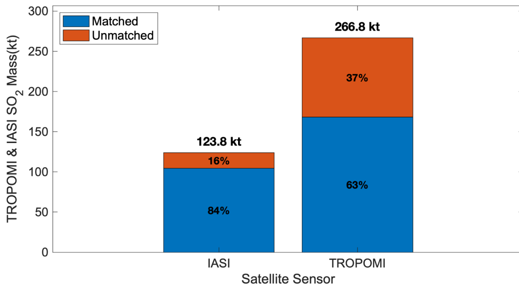
Figure S.3: Total SO 2 masses calculated by IASI (left) and TROPOMI (right) showing proportions of matched (blue) and unmatched (red) detections, where matches represent TROPOMI and IASI detections of SO 2 from Shishaldin Volcano acquired within 3.3 hours of each other.
