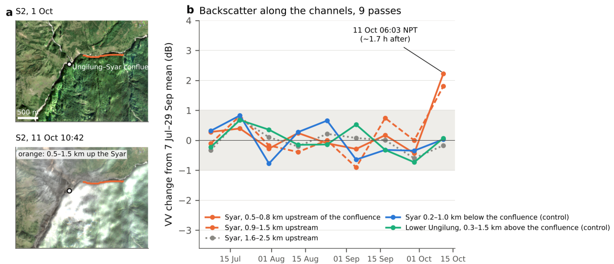
Figure 8. The Syar Khola blockage. (a) Sentinel-2 true colour on 1 October and 11 October 10:42 near the Ungilung–Syar confluence (white circle). Orange line: the Syar reach 0.5–1.5 km upstream of the confluence. (b) Sentinel-1 VV backscatter (descending track 19) along channel reaches, as the change from the mean of the passes from 7 July to 29 September. Grey band: \pm 1 dB.
