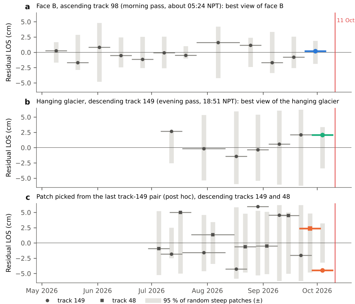
Figure 6. NISAR L-band interferograms (12-day pairs; three 24-day): residual line-of-sight displacement averaged over fixed outlines, after removing the phase that follows elevation. Horizontal bars span each pair; grey bars are the range containing 95 % of random steep patches in the same pair. Coloured: the last pair before the event on each track. (a) Face B on ascending track 98. (b) The hanging glacier on descending track 149. (c) The patch picked from the last track-149 pair, on descending tracks 149 (circles) and 48 (squares). Red line: 11 October.
