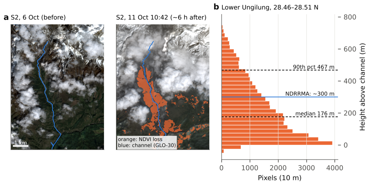
Figure 7. Vegetation loss along the lower Ungilung Khola. (a) Sentinel-2 true colour on 6 October and 11 October 10:42, with pixels that lost vegetation (orange) and the GLO-30 channel (blue). (b) Height above the channel of the vegetation-loss pixels between 28.46° and 28.51° N, with the median, the 90th percentile and the about 300 m given by NDRRMA (2026b).
