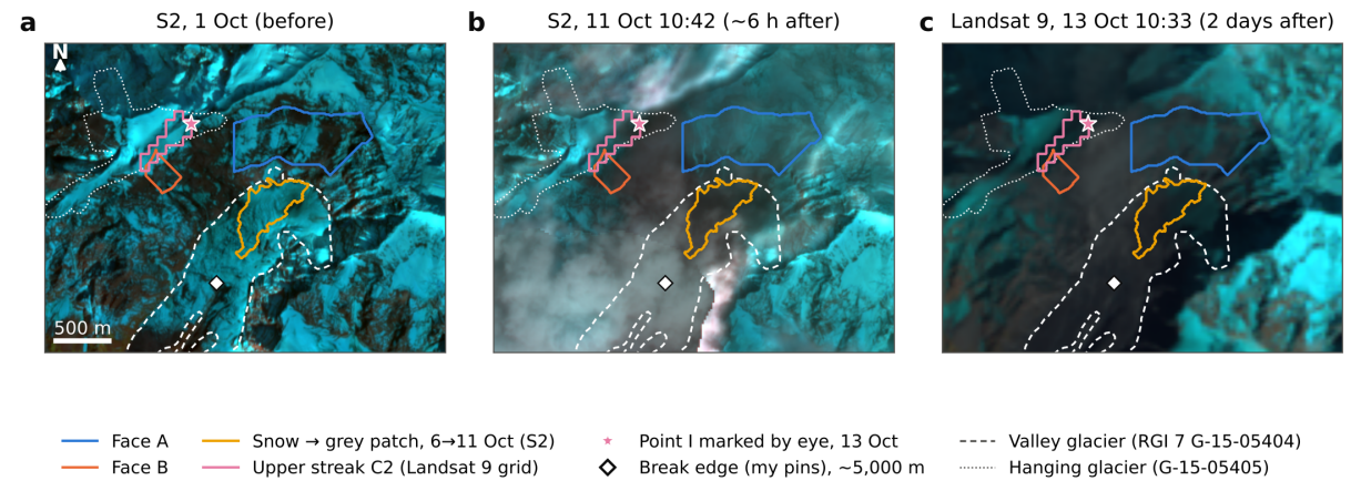
Figure 3. False-colour composites of the source area (SWIR1, NIR, green; snow and ice appear cyan, rock and debris brown or grey). (a) Sentinel-2, 1 October. (b) Sentinel-2, 11 October 10:42, partly cloudy. (c) Landsat 9, 13 October (bands 6, 5, 3). Outlines: face A (blue), face B (orange), Sentinel-2 snow → grey patch of 6 → 11 October (yellow), upper track C2 from the Landsat 9 grid test (pink), valley glacier and hanging glacier from RGI 7 (white dashed and dotted). Star: the possible failure point I marked by eye on 13 October that falls inside C2. Diamond: the break edge I marked on Google Earth images from 2006 to 2026.
