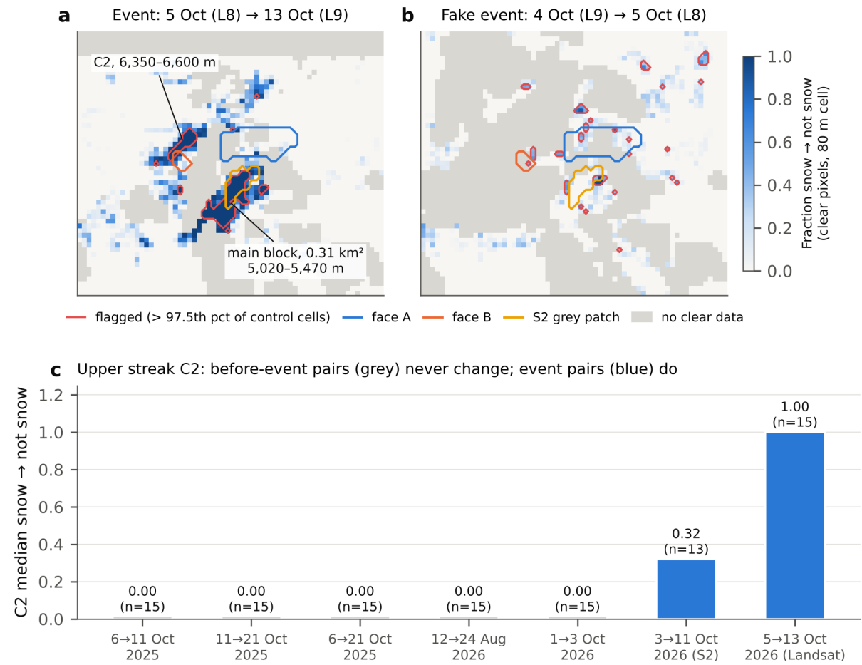
Figure 4. Grid-cell snow-loss test (80 m cells). (a) Event pair: Landsat 8, 5 October → Landsat 9, 13 October. (b) Fake pair: Landsat 9, 4 October → Landsat 8, 5 October. Red outlines: cells above the 97.5th percentile of control cells (0.98 in a, 0.35 in b). Grey: no clear data. (c) Median snow loss in the upper track C2 for five Sentinel-2 pairs taken before the event in which all 15 C2 cells were clear (grey), and for the two event pairs (blue). n is the number of valid cells.
