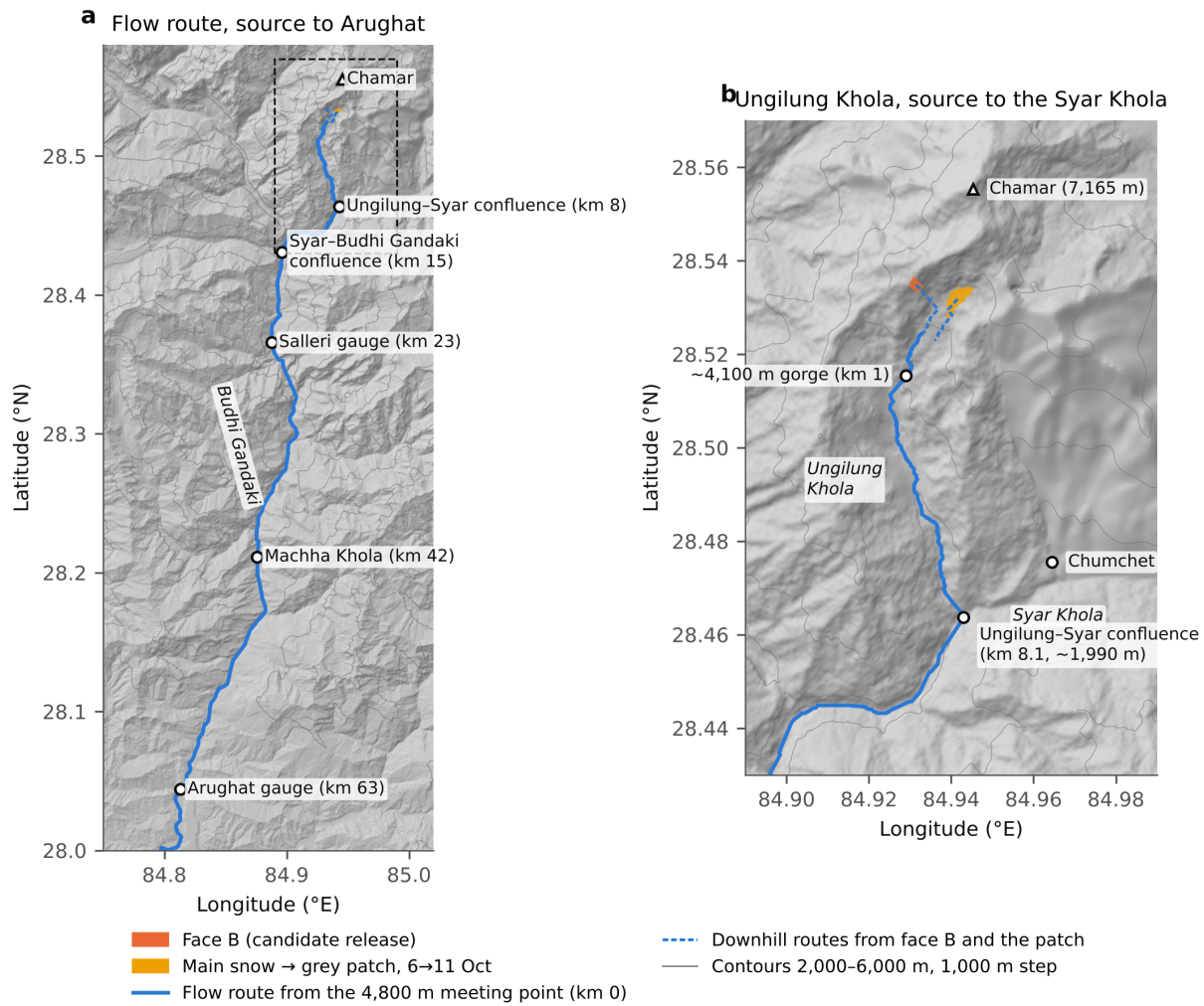
Figure 1. Location. (a) Flow route from the 4,800 m meeting point of the routes from faces A and B (km 0) to Arughat (km 63) on a GLO-30 hillshade, with river kilometres of the confluences and gauges. (b) The Ungilung Khola from the source to the Syar Khola. Orange: face B; yellow: the main snow → grey patch of 6 → 11 October (Sentinel-2); dashed blue: downhill routes from face B and from the patch. Contours every 1,000 m.
