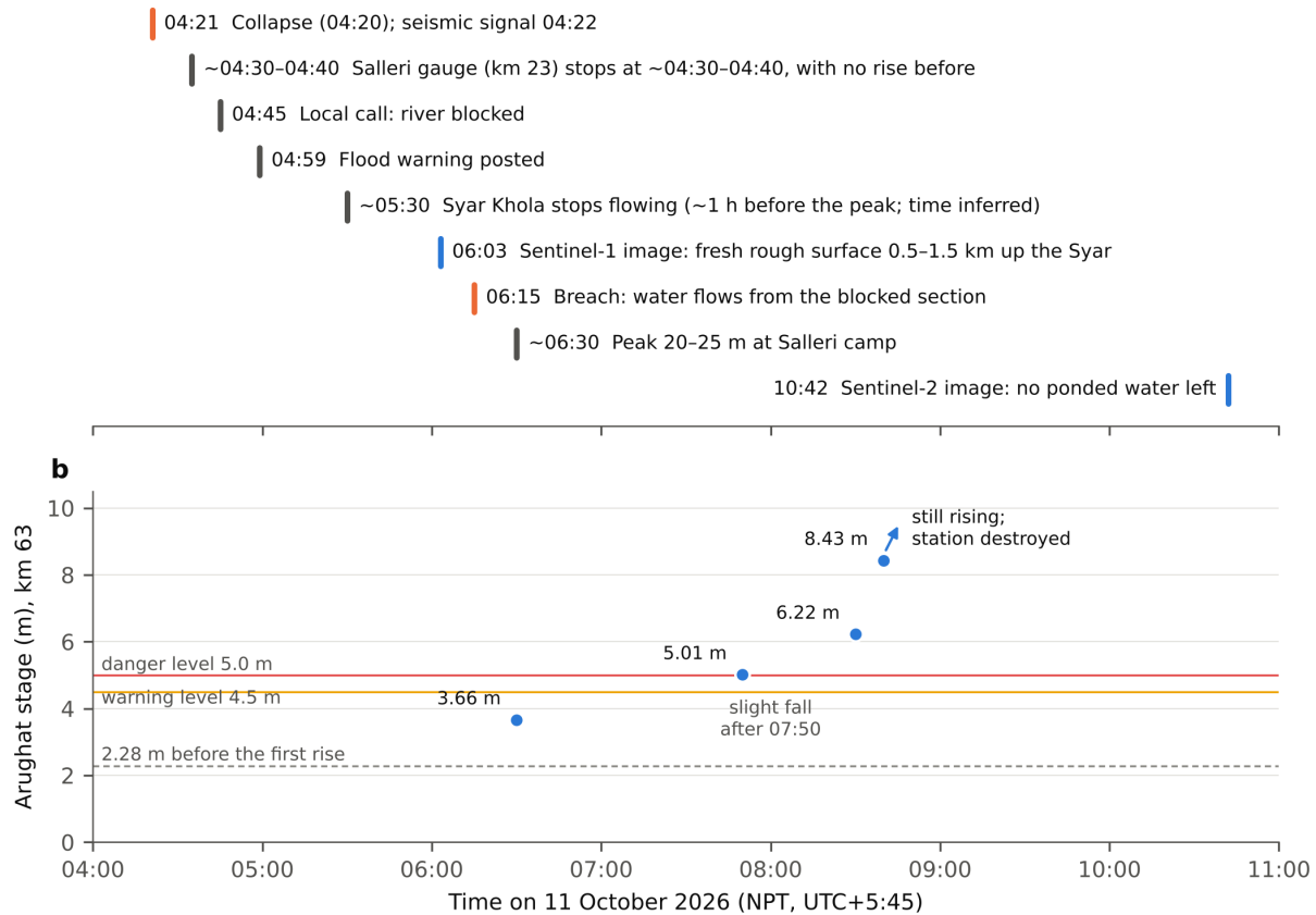
Figure 2. (a) Events on 11 October 2026, from the seismic record (Petley, 2026), NDRRMA (2026a, b), the Kathmandu Post (2026) and this study (blue). The end of the Salleri record is given as about 04:30–04:40. The time the Syar stopped flowing is inferred from “about one hour before the largest level”. (b) Arughat gauge readings (HWRRC, 2026). The report states that the level fell slightly after 06:30 and after 07:50; these falls were not given as values and are not plotted.
