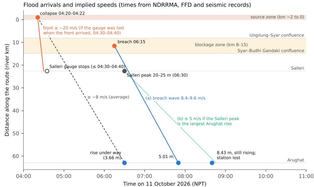
Figure 9. Distance–time diagram of the flood. River kilometres are measured from the point at 4,800 m where the routes from faces A and B meet; the source faces lie about 1.5–2 km upslope. Points are the times in Fig. 2. Lines are average speeds between them: the front to Salleri (orange) and the average to the first Arughat rise (grey). Blue and green are the two alternatives of Sect. 3.7: (a) the 06:15 breach wave reaching Arughat at 07:50; (b) the largest Salleri level reaching Arughat as the third rise.
