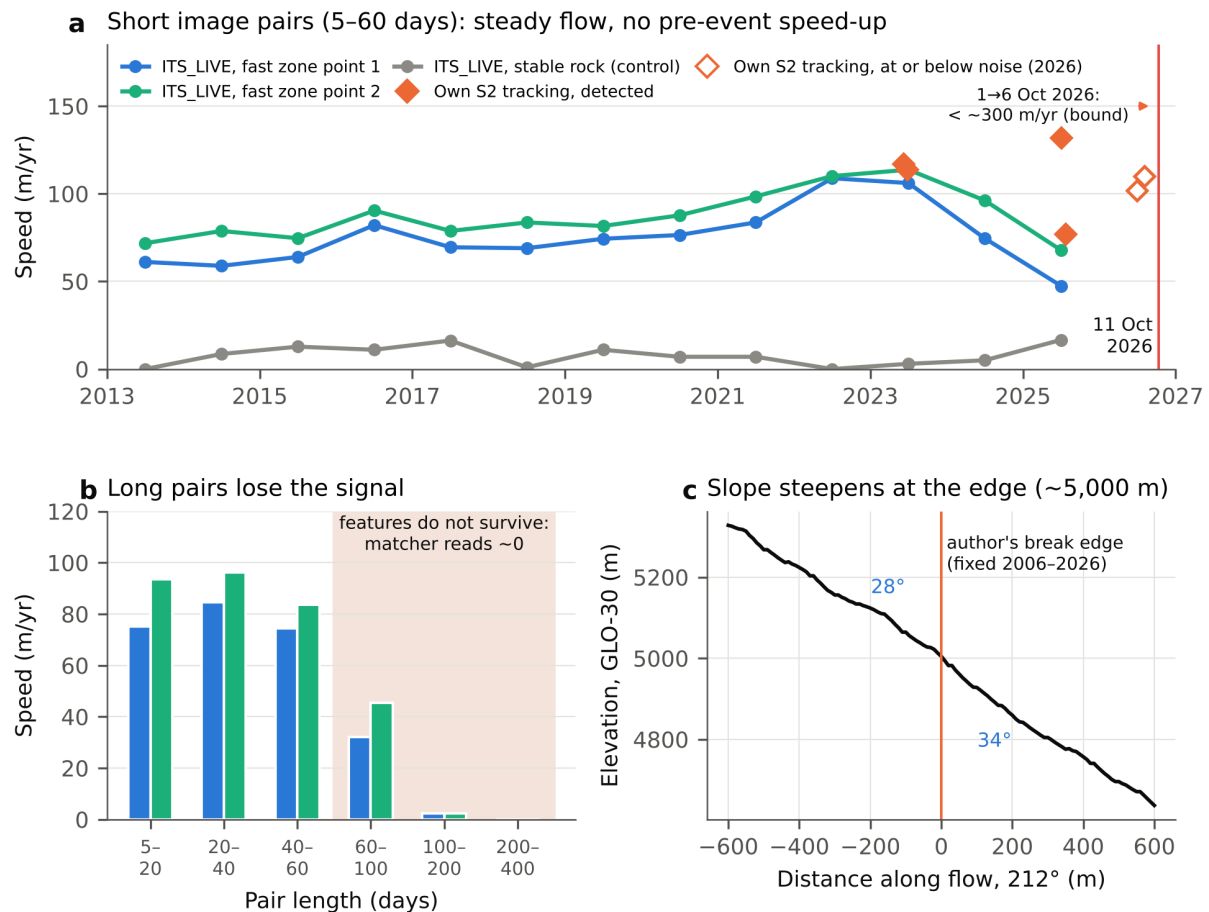
Figure 5. The glacier before the event. (a) Speed of the fast zone from ITS_LIVE image pairs of 5–60 days (vector median per year) at two points (blue, green) and at stable rock (grey), with my own Sentinel-2 feature tracking (filled: above noise; open: at or below noise). Arrow: upper bound for 1 → 6 October 2026. (b) Speed against pair length at the two points. (c) GLO-30 profile along the flow line (212°) through the break edge, with the mean slope 300 m above and below it.
