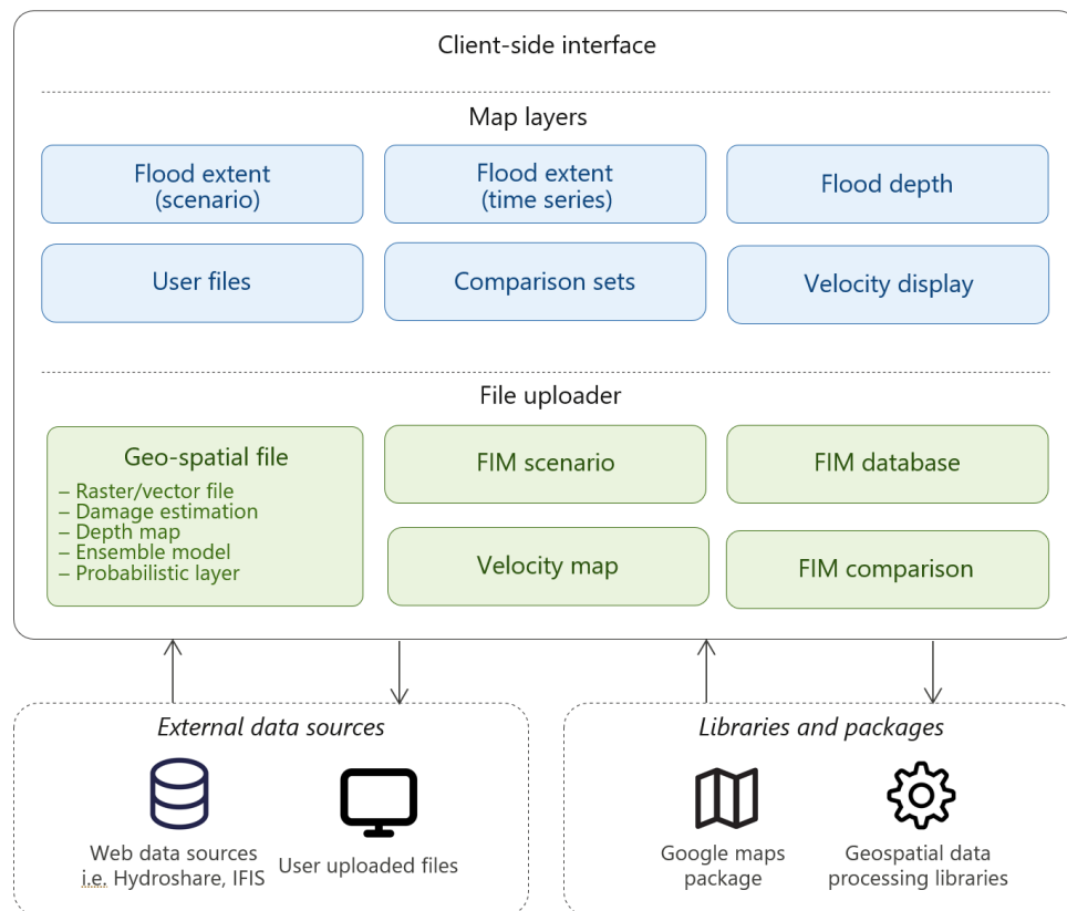
Figure 1. Software architecture of FIMApp. It comprises two core components: Map Layers and File Uploader, each with distinct functions for dynamic dataset ingestion and use.
