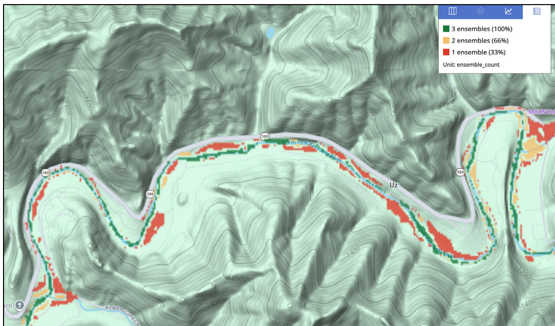
Figure 9. Ensemble agreement map for a section of the North Fork Kentucky River, rendered as a classified raster. Each class represents the number of models predicting inundation at that location, with green for three, orange for two, and red for one model. The class value colors are read from the GDAL_METADATA tag in the file header.
