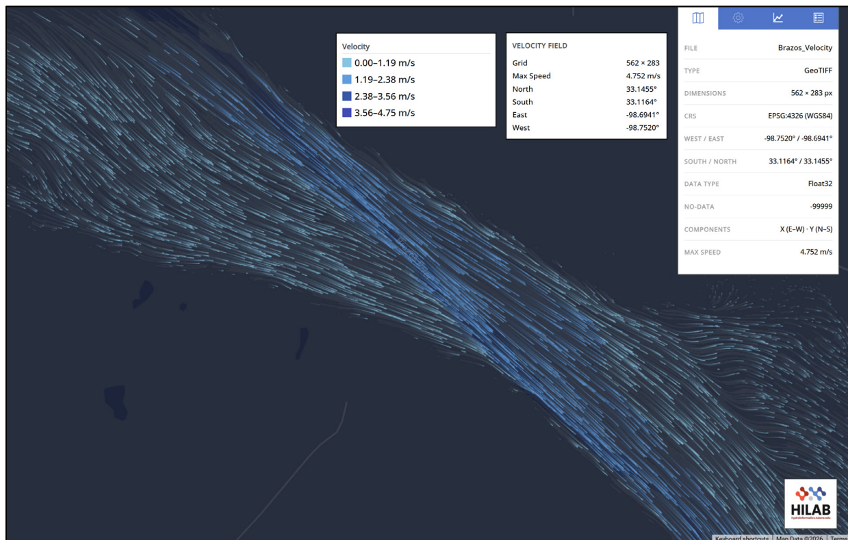
Figure 14. An animated velocity field for a scenario on the Brazos River. We have changed the map type to night to make moving particles easier to trace. Particle streak movement and color indicate velocity.
