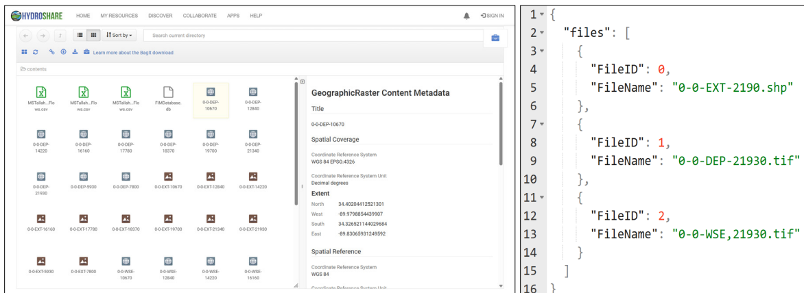
Figure 2. (Left) Screenshot of the HydroShare platform showing the BYU FIM Database with a list of available files. (Right) An excerpt from the FIMDatabase.json file describing the data structure for the FIM Database format. This self-describing structure lets users provide a simple yet scalable file structure that can be shared across multiple instances.
