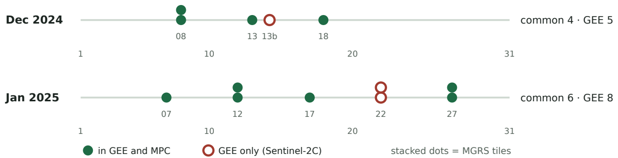
Figure 3. Scenes entering the December 2024 and January 2025 monthly composites (scene cloud cover \leq 20\% ). Filled dots are scene-tile records present in both catalogues; open dots are Sentinel-2C records present only in GEE; stacked dots are the two tiles of one acquisition. On 13 December two datatakes occurred, one present in both catalogues and one Sentinel-2C datatake present only in GEE; the second is drawn offset.
