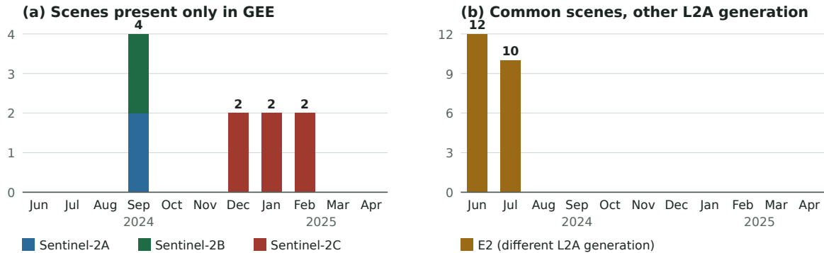
Figure 2. Catalogue reconciliation over the study farm, June 2024 to April 2025 (queries of 24 September 2026). (a) Scene-tile records present only in GEE, by month and satellite; no record was present only in MPC. (b) Records present in both catalogues but with different L2A generations of the same acquisition (E2), by month.
