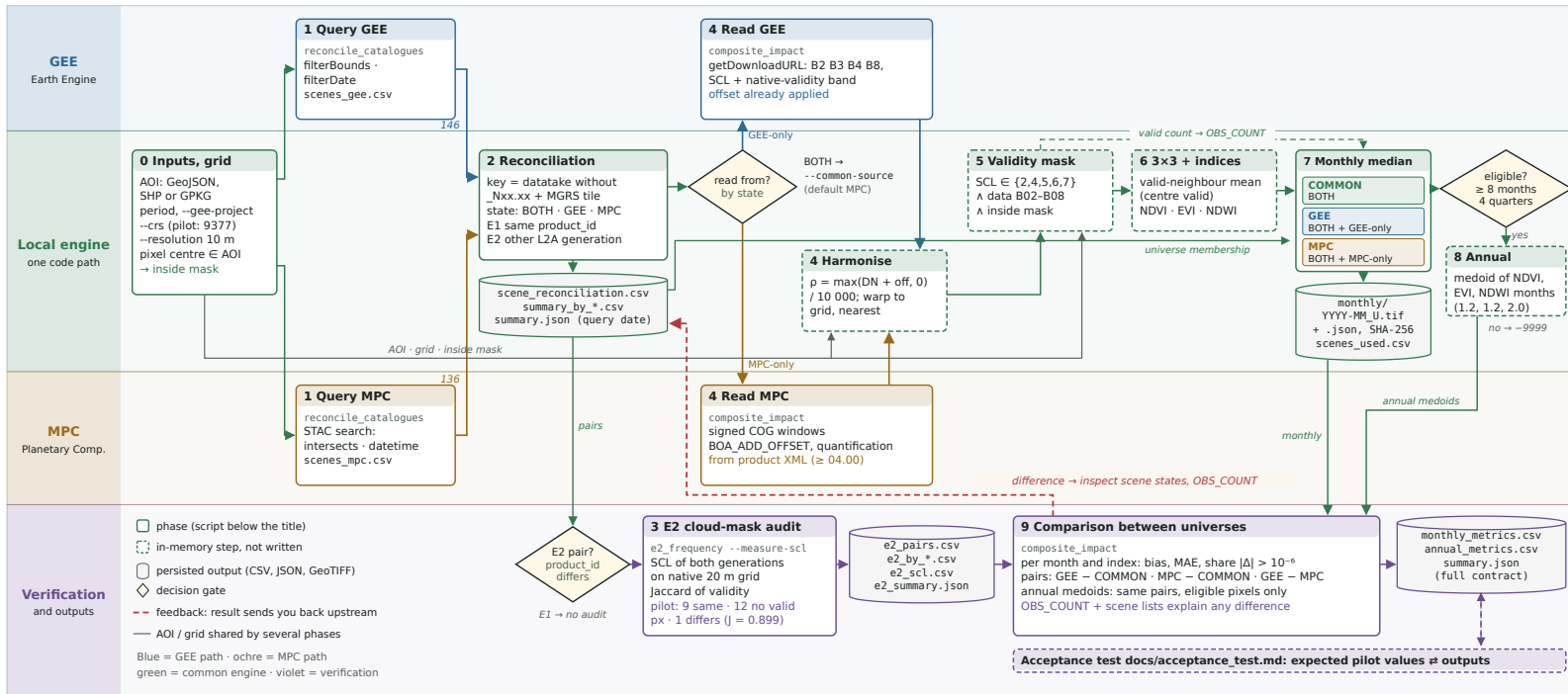
Figure 1. (A) Study design: four comparison levels, each isolating one source of difference while holding constant what the previous level established. Levels 1 and 4 correspond to the scene-universe layer of Table 1, and levels 2 and 3 to the product and processing layers. The dashed red arrow marks the feedback that redirected the investigation from processing to the scene catalogues. (B) Data flow of the released toolkit in swimlanes (GEE, local engine, MPC, verification). Phases are numbered 0–9; each shows its operation, inputs and outputs, with the script below its title. Cylinders are files written to disk, dashed boxes are in-memory steps and diamonds are decision gates. The reconciliation state of each scene decides which catalogue it is read from and which scene universes it enters. Values from this study appear in italics or after “pilot”. Python libraries and versions are given in Section 2.4.
