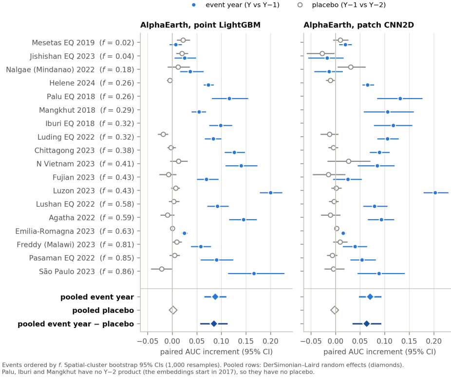
Fig. 2. Event-year and placebo increments for the 18 events (AlphaEarth), for the point model on the 10 m vector (left) and the patch model on 11 \times 11 cells of 30 m (right). Bars are spatial-cluster bootstrap 95% CIs. Diamonds show the DerSimonian-Laird pooled event-year increment, placebo and placebo-corrected increment. Events are ordered by f .
