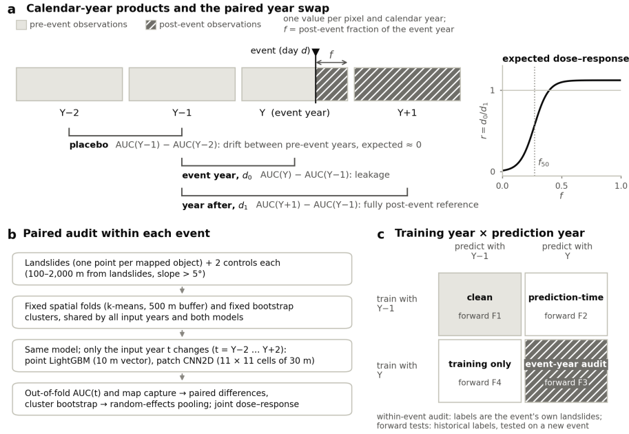
Fig. 1. Study design. (a) Annual products summarize one calendar year. For an event on day d of year Y , the event-year product contains a post-event fraction f = (365 - d)/365 of the year. The paired year swap compares out-of-fold AUCs of the same model with inputs from different years. The contrasts are the event-year increment d_0 ( Y vs Y-1 ), the placebo ( Y-1 vs Y-2 ) and the year-after increment d_1 ( Y+1 vs Y-1 ). If leakage follows the post-event share of the year, the ratio d_0/d_1 should rise with f (inset). (b) The audit pipeline within each event. (c) The training-year \times prediction-year grid. The within-event audit uses the event's own landslides as labels. The forward tests use earlier landslides as labels and a new event for testing; their scenarios F1–F4 occupy the same four cells.
