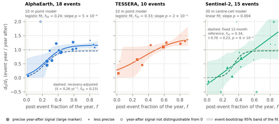
Fig. 4. Dose–response in three annual representations: the ratio of the event-year to the year-after increment against f . AlphaEarth and TESSERA use the 10 m point model. The Sentinel-2 panel uses LightGBM on the central 30 m cell of the composite patches, for which a fixed 12-month reference exists; the 10 m point model of Table 2 gives a weaker calendar-reference slope ( p = 0.046 ). Marker area scales with the precision of the year-after signal. Small open markers are events whose year-after increment is indistinguishable from zero, so their ratios carry little information. Ratios beyond -0.5 or 2 are drawn at the axis limits. Solid lines are joint random-effects fits (logistic, or linear where the logistic fit degenerated to a step), and shaded bands are 95% event-bootstrap ranges of these fits. Dashed lines are fits with references free of the recovery coupling: year-after increments rescaled for the recovery measured from the year after next (AlphaEarth), and the fixed 12-month post-event reference (Sentinel-2).
