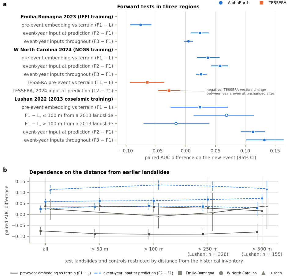
Fig. 7. Forward tests. (a) Paired AUC differences on the new event in three regions (95% cluster-bootstrap CIs). F1 – L compares legitimate pre-event embeddings with static factors, F2 – F1 adds event-year inputs at prediction, and F3 – F1 uses event-year inputs throughout. For Lushan, open circles split F1 – L by whether the test landslide lies within 100 m of a 2013 landslide. Squares show the TESSERA comparisons in North Carolina: pre-event TESSERA against static factors (T1 – L) and 2024 TESSERA inputs at prediction (T2 – T1). (b) The same differences when test landslides and controls are restricted to sites farther from the earlier inventory. Solid lines show F1 – L and dashed lines F2 – F1. The Lushan subsets beyond 250 m and 500 m contain only 326 and 155 test landslides.
