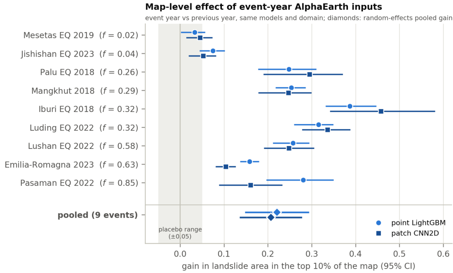
Fig. 6. Map-level effect for nine events with complete inventories: the gain in landslide area within the top 10% of the map when the event-year AlphaEarth product replaces the prior-year product (95% spatial-cluster bootstrap CIs). The shaded band marks the range of the single-event map placebos (about \pm 0.05 ). Diamonds are random-effects pooled gains.
