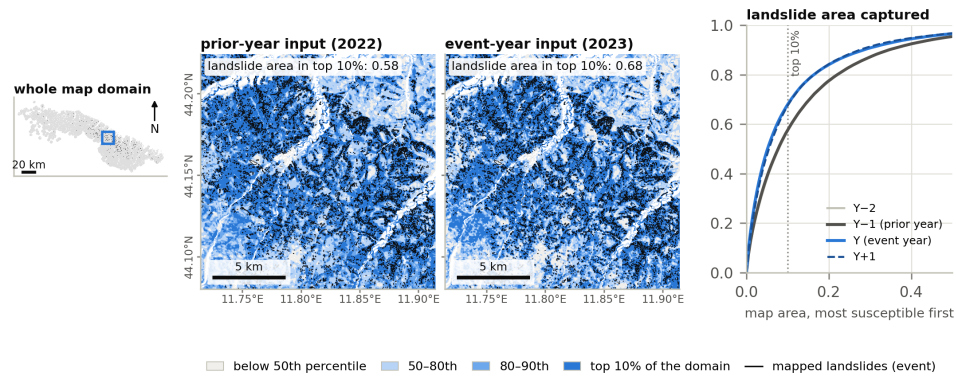
b Emilia-Romagna rainfall, 16 May 2023 ( f = 0.63 ); out-of-fold patch CNN2D maps
