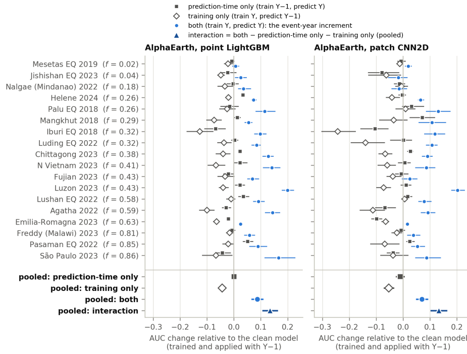
Fig. 3. Training-year × prediction-year decomposition within each event (AlphaEarth; same points, folds and bootstrap clusters as Fig. 2). Markers give the AUC change relative to the clean model, which is trained and applied with Y-1. Squares show event-year inputs at prediction only, open diamonds in training only, and circles in both, which is the event-year increment. The bottom rows are random-effects means, including the pooled interaction (triangles). Within each event the increment equals the sum of the three components; the pooled rows are pooled separately and need not add up exactly.
