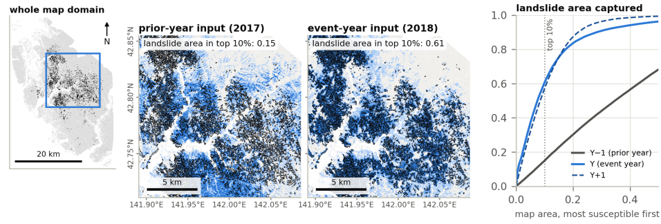
a Eastern Iburi earthquake, 6 Sep 2018 ( f = 0.32 ); out-of-fold patch CNN2D maps
