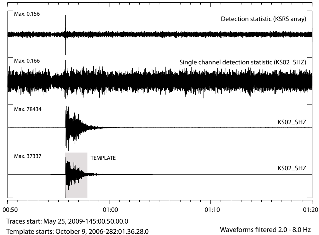
Fig. 13. Correlation of a 120 second long template from the October 9, 2006, DPRK test with a 30 minute long data segment on May 25, 2009, on the KSRS array in the Republic of Korea. Only the channel KS02_SHZ is shown although the array detection statistic trace is constructed using all 19 short period vertical channels of the array. The template waveform is aligned with the 2009 signal according to the time of the maximum of the detection statistic trace. The importance of the stacking the single channel detection statistic channels over the array is evident. The DSSNR in the above plot is 65.0, in comparison with 106.7 for the calculation on the MJAR array.
