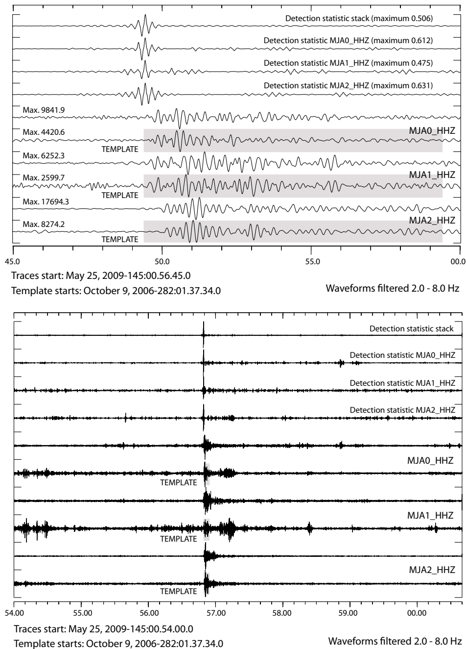
Fig. 6. Waveforms from three channels of the MJAR array from the May 25, 2009, DPRK nuclear test aligned with the corresponding waveforms from the October 9, 2006, event. The corresponding individual channel detection statistic traces are displayed with the array stack. The upper panel is a close-up of the lower panel.
