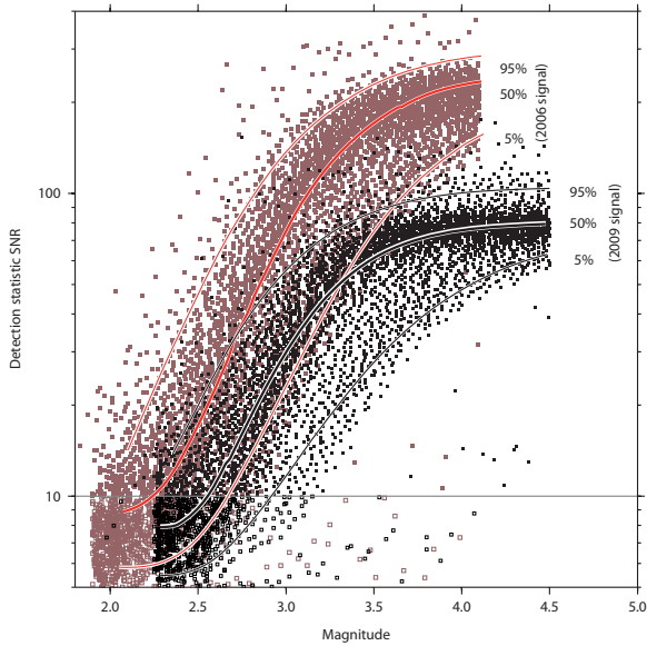
Fig. 12. Detectability using a multi-channel correlator on the MJAR array of signals from the 2006 and 2009 explosions, scaled down into different segments of background noise, using the signal from the 2006 explosion as a template. The m_b magnitudes for the 2006 and 2009 events are assumed to be 4.1 and 4.5 respectively and the magnitude of the simulated events are taken to be 4.1 + \log_{10}(\varepsilon) and 4.5 + \log_{10}(\varepsilon) where \varepsilon is the factor that the explosion signal is scaled by before adding to the background noise at a given time. Only one in 50 of the points used to estimate the detectability curves is plotted on the graph. The detectability curves are based on the points contained in intervals of 0.05 magnitude units.
