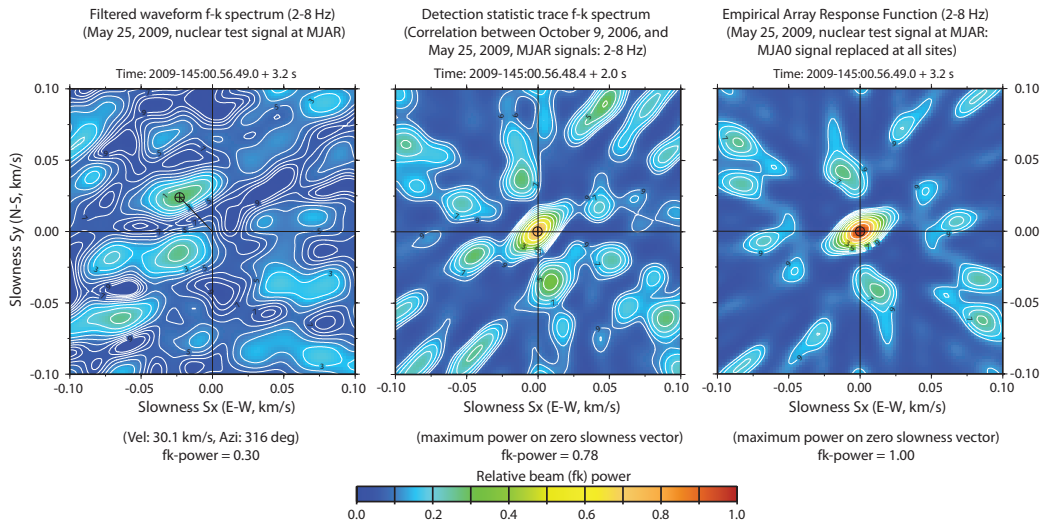
Fig. 7. Frequency-wavenumber spectrum on the MJAR array of (left) a 3.2 second long data window for Pn arrival for the 2009 test, (center) for the single channel detection statistic traces for a 2.0 second window centered at the time of the local maximum (see Fig. 6), and (right) an estimate of the broadband Array Response Function (ARF). The calculations involved in obtaining the f-k spectra in the left and right panels are identical except that, for the ARF, the waveforms at all sites have been replaced with the filtered waveform on the MJA0 sensor. This illustrates how the array would respond to a perfectly coherent wavefront, with the same frequency content as the nuclear test signal, approaching all sensors simultaneously.
