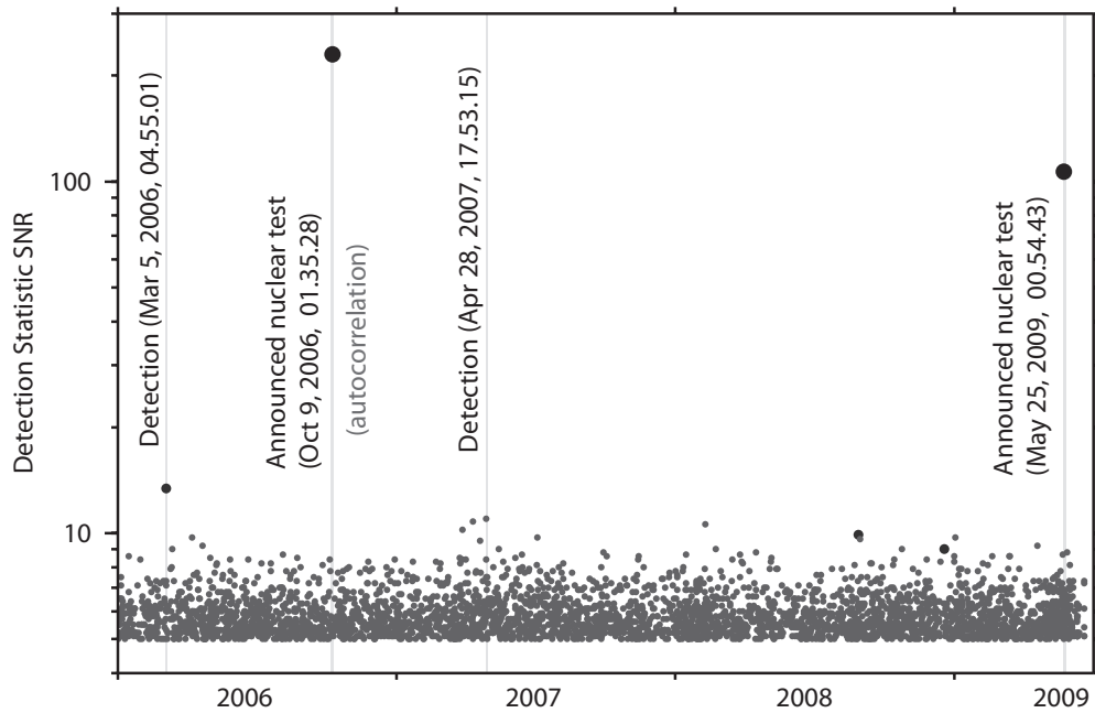
Fig. 8. Detections from the correlator on the MJAR array where the 8 second long signal template is begins at a time 2006-282:01:37.32.6. The value denoted “Detection statistic SNR” is described in the text and measures the ratio between the array detection statistic C(t) defined in Equation 3 and the background level of the same quantity. Vertical bars indicate the times of the four highest values obtained in the period January 1, 2006, to June 20, 2009.
