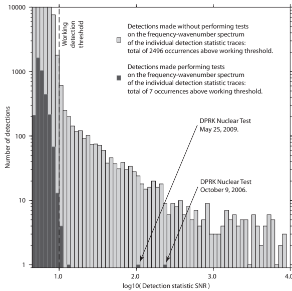
Fig. 9. Histograms of correlation detections with and without f-k post-processing on the individual channel detection statistic traces. The number of detections in each bin corresponds to the time-interval displayed in Fig. 8. 209 detections obtained without the f-k post-processing exceed the detection statistic SNR for the autocorrelation. All of these detections are the result of faults in the data (e.g. gaps).
