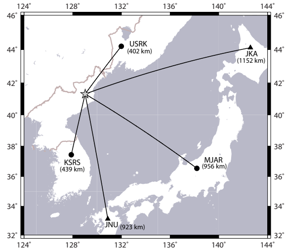
Fig. 1. Location estimate for the May 25, 2009, North Korea nuclear test with respect to the closest five IMS stations. Circles indicate primary seismic array stations and triangles indicate auxiliary 3-component stations.
