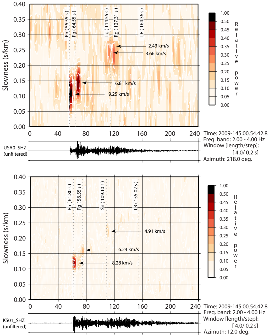
Fig. 2. Vespagrams [17] for the 2009 event signals on the USRK and KSRS arrays. Each panel displays a relative power (the ratio of energy in the beam to the mean energy of the individual traces) where the beam is constructed according to time-delays determined by the fixed backazimuth and an apparent velocity v_{app} = 1/s \text{ kms}^{-1} . A single channel trace is displayed for each array.
