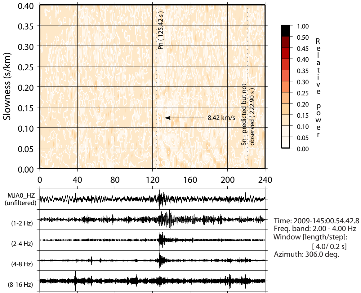
Fig. 4. Vesogram for the 2009 event signal on the MJAR array. The MJA0_HZ channel is displayed both unfiltered and bandpass filtered as indicated.
