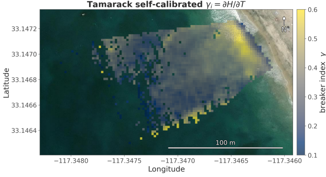
Figure 3: Map of the per-cell tide slope \gamma_i = \partial H / \partial T at Tamarack in the Fall-2025 window (20 September–3 October 2025), fitted separately in each 2 m cell with Eq. (10) from the individual pocket heights and drawn over satellite imagery with a north arrow and a 100 m scale bar true at 33.147°N. The index \gamma_{sc} itself is read from the index table on 3 m cells (Secs. 2.2.1 and 2.2.5). Cells whose tide bins span less than 0.20 m are left out, because two adjacent tide bins give a two-point slope; slopes outside 0–1.6 are not drawn, and the map is shown with a 3 \times 3 -cell running mean. The color scale runs from \gamma_i = 0.1 (dark blue) to 0.6 (yellow). The band 10–20 m seaward of the landward edge, along the active whitewater line, gives \gamma_i \approx 0.45 –0.55 (yellow), around \gamma_{sc} = 0.50 . Seaward of it \gamma_i falls to 0.30–0.35 and, beyond 60 m, to about 0.25 (blue to gray).
