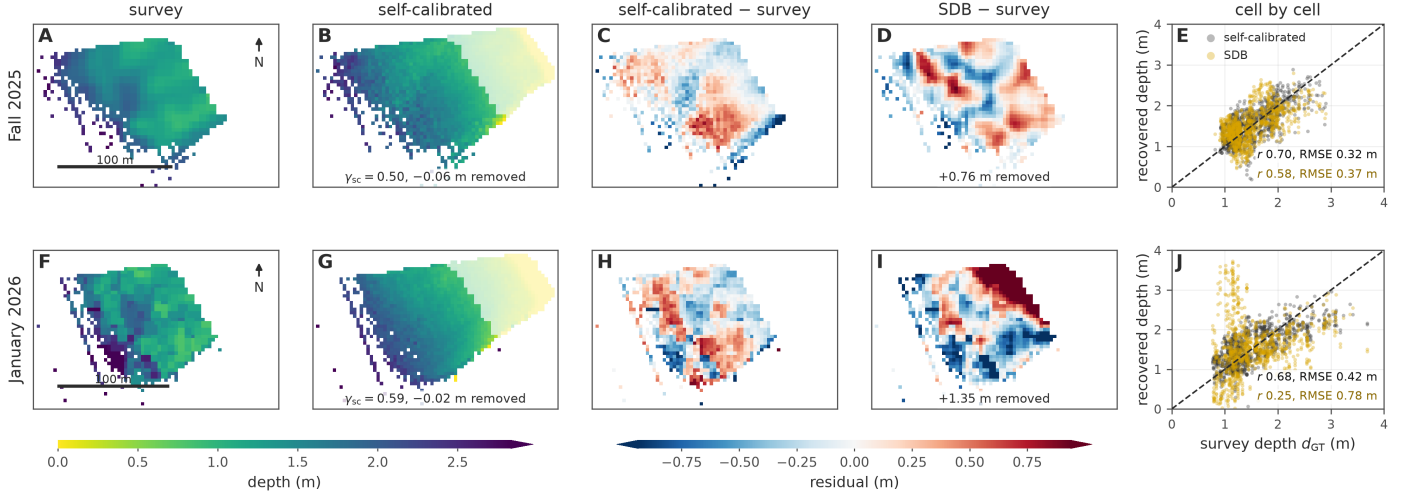
Figure 4: Self-calibrated depth and Sentinel-2 SDB compared with the two surveys at Tamarack, Fall 2025 (A–E, 1,098 cells, 9,900 m 2 ) and January 2026 (F–J, 1,053 cells, 9,500 m 2 ), on the cells of Table 1. (A, F) Survey depth, with a north arrow and a 100 m scale bar true at 33.147°N. (B, G) Self-calibrated depth with the index of each period, \gamma_{sc} = 0.50 and 0.59 , on the depth scale of A and F; the cells beyond the survey are faded. (C, H) Its residual against the survey. (D, I) The residual of Sentinel-2 SDB with the published method, calibrated on ICESat-2 and sampled onto the 3 m camera grid, on the same diverging scale. Each field is shown with its constant offset to the survey removed, and the amount removed is printed on B, D, G and I. (E, J) Cell-by-cell scatter of both fields against the survey (black: self-calibrated; gold: SDB), with r and the RMSE after offset removal. The figure compares the spatial pattern recovered by the camera inversion and by SDB with the survey in both periods.
