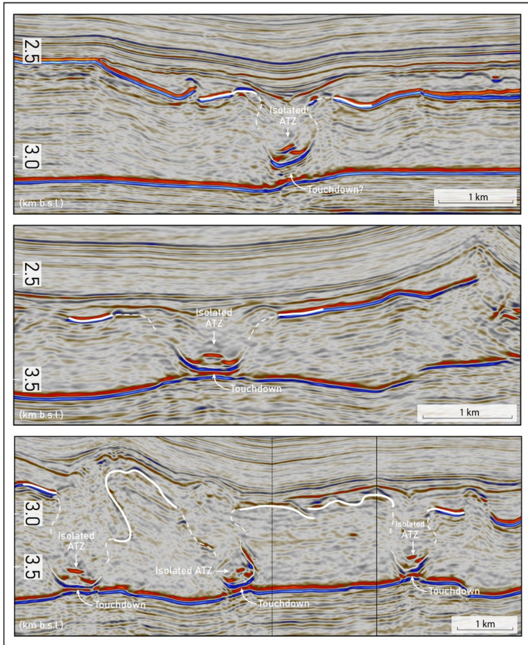
Fig. S8. Isolated ATZs that have reached the base of the salt. In each section the thickened body is detached from the adjacent Z3a (dashed) and rests on the Base Zechstein reflection ("touchdown"), in contrast to the suspended position of ATZs within a continuous sheet. Depth in km below sea level.
