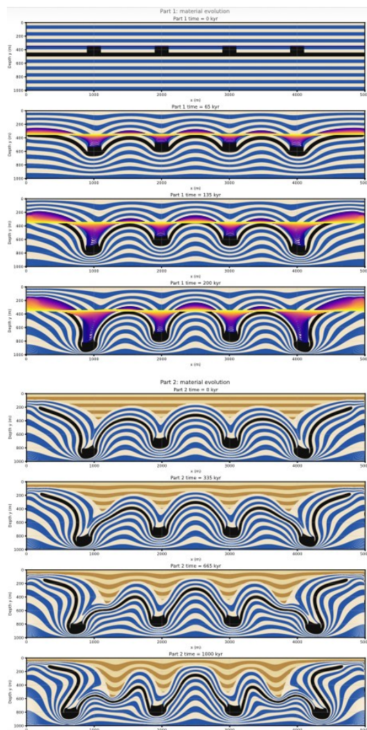
Fig. S12. Material evolution of the reference (attached) experiment during Phase 1 (Fig. 4A, Stages 1–3; density-driven foundering; 0–200 k.y.) and Phase 2 (Stages 4–5; sand loading; 0–1000 k.y. after the end of Phase 1).
