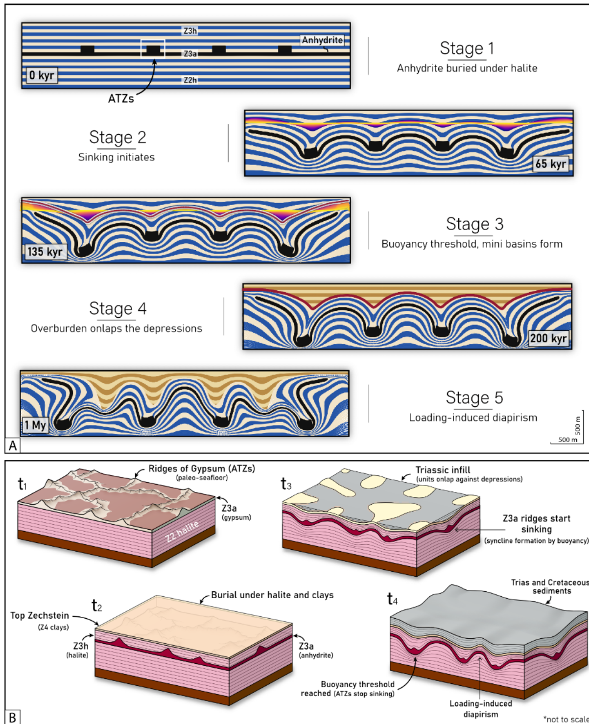
Figure 4. Numerical and conceptual models of ATZ foundering and minibasin nucleation.
