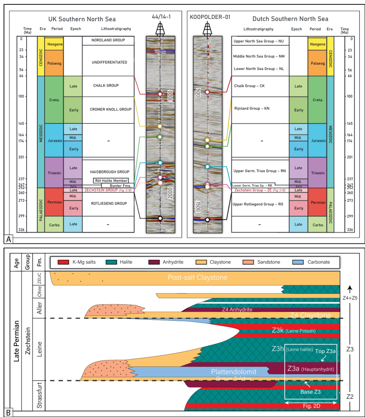
Fig. S2. Stratigraphic framework. (A) Chrono- and lithostratigraphy of the UK (left) and Dutch (right) Southern North Sea on a common time scale, tied to wells 44/14-1 (TWT) and Koopolder-01 (depth); colored markers are the horizons mapped in this study. (B) Zechstein lithostratigraphy, showing the Z3a (Hauptanhydrit) and the interval imaged in Figure 2D.
