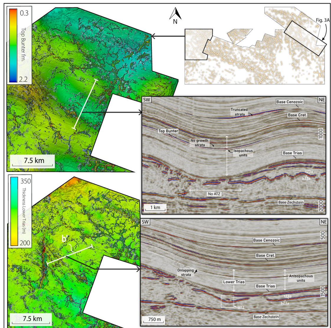
Fig. S7. Synclines with and without an underlying ATZ. Top: a syncline with no ATZ in its hinge; Triassic units are isopachous through the structure and no growth strata are developed. Bottom: an ATZ-cored syncline in the same area, with lower Triassic strata thickening into the low and onlapping its flanks. Maps are Top Bunter time-structure and Lower Triassic thickness.
