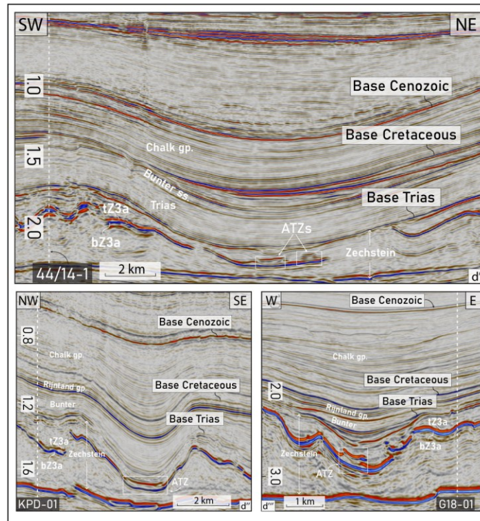
Fig. S3. Regional sections d', d'' and d''' of Figure 2D, enlarged. ATZs (boxes) occupy the cores of synclines whose axes persist upward to the Base Cenozoic. Wells 44/14-1, KPD-01 and G18-01. tZ3a, bZ3a: top and base Z3a.
