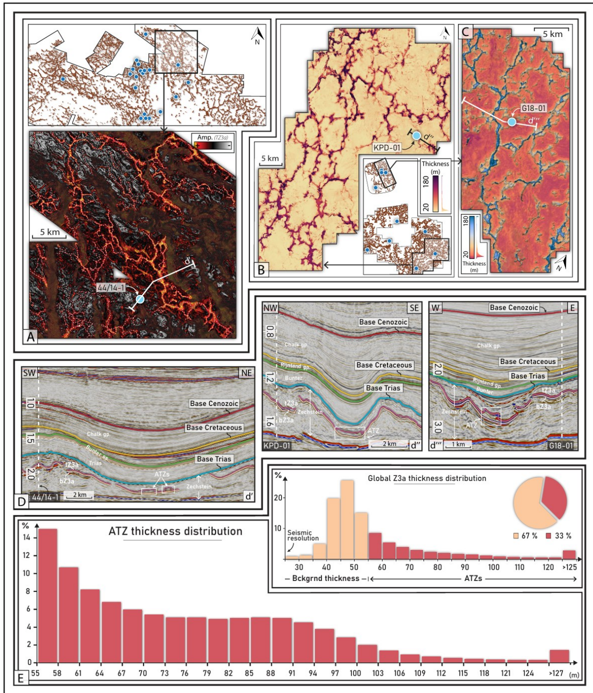
Figure 2. Distribution, thickness and seismic expression of the Z3a ATZ network. (A) UK sector: root-mean-square amplitude on the Top Z3a. (B, C) Dutch sector: Z3a isopachs. (D) Sections (d', d'', d''') tied to wells 44/14-1, KPD-01 and G18-01, showing ATZs in the cores of synclines expressed upward to the Base Cenozoic (enlarged in Fig. S3). (E) ATZ thickness distribution (inset: full Z3a). tZ3a, bZ3a: top and base Z3 anhydrite.
