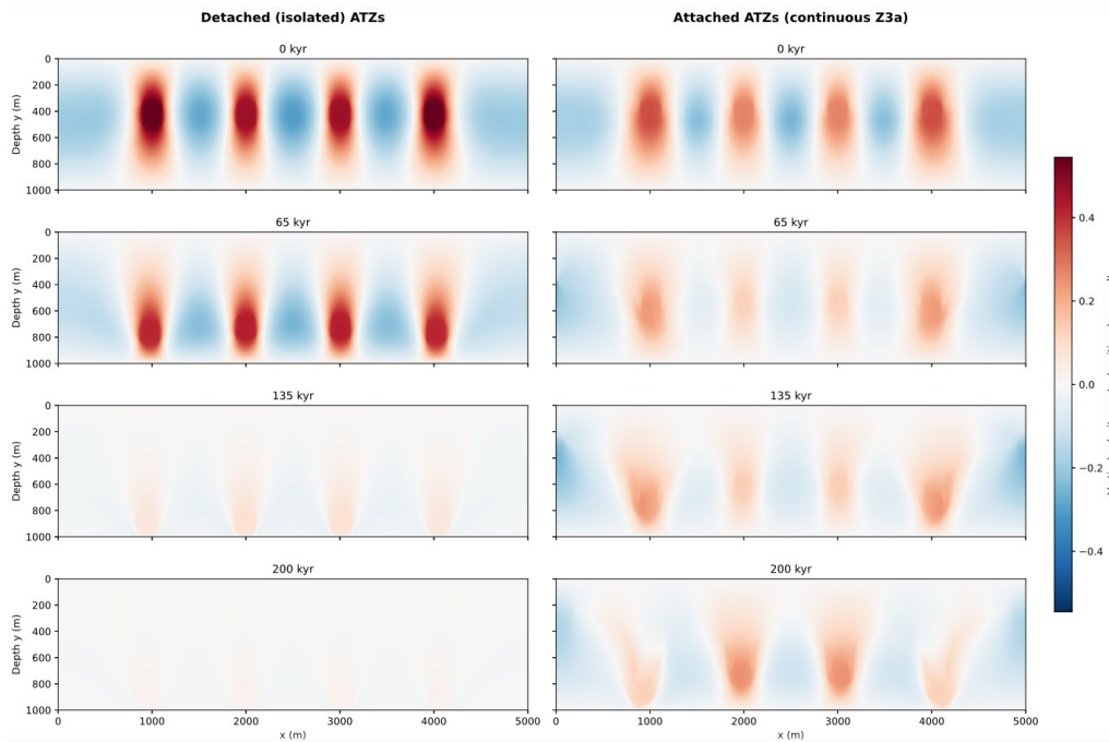
Fig. S11. Vertical velocity in the detached (left) and attached (right) ATZ experiments at 0, 65, 135 and 200 k.y., shown on a common color scale (positive downward). Detached ATZs sink faster, initially \sim 0.54 cm/yr against \sim 0.35 cm/yr when
