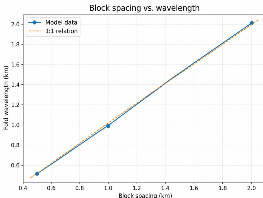
Fig. S16. Effect of anhydrite block spacing on the wavelength of overburden folds. The model results closely follow the 1:1 relationship (dashed line), indicating that fold wavelength is primarily controlled by the spacing between adjacent anhydrite blocks.
