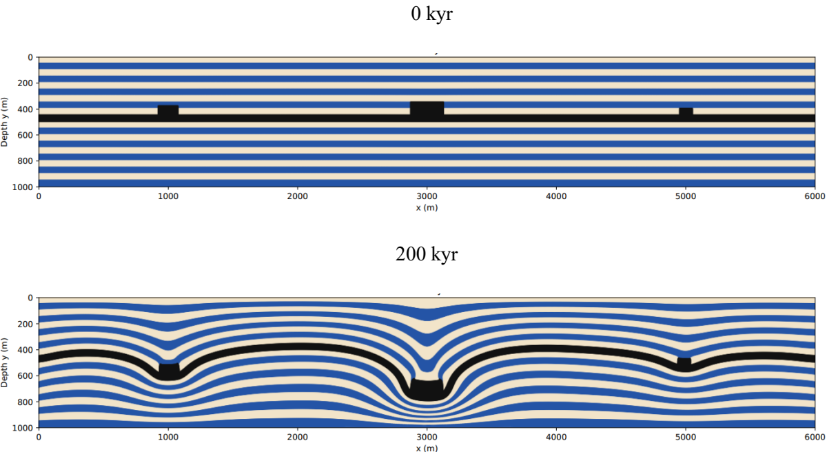
Fig. S14. Effect of anhydrite block geometry on sinking behavior and overlying synclinal depressions. The model contains three anhydrite blocks of different dimensions: left ( l = 150 m, h = 120 m), middle ( l = 250 m, h = 150 m), and right ( l = 100 m, h = 100 m), where l and h denote block length and height, respectively. The blocks exhibit different sinking rates, illustrating the influence of block geometry on gravitational sinking through halite.
