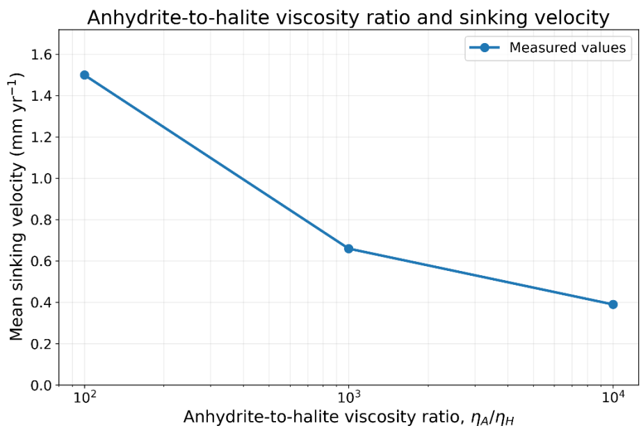
Fig. S13. Effects of density contrast (keeping viscosity ratio constant at 100) and viscosity ratio (keeping density contrasts constant at 700 kg/m 3 ) on anhydrite sinking velocity in the reference models. The measured values represent the mean sinking velocity of the two central anhydrite blocks.
