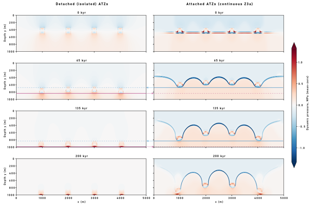
Fig. S10. Dynamic pressure (mean-zero) in the detached (left) and attached (right) experiments at 0, 65, 135 and 200 k.y., on a common color scale; values beyond \pm 1.3 MPa, at ATZ corners and basal contacts, are saturated. At 65 and 135 k.y., solid lines mark the depth of the deepest ATZ in each configuration, and dashed lines repeat it in the other panel for comparison.
