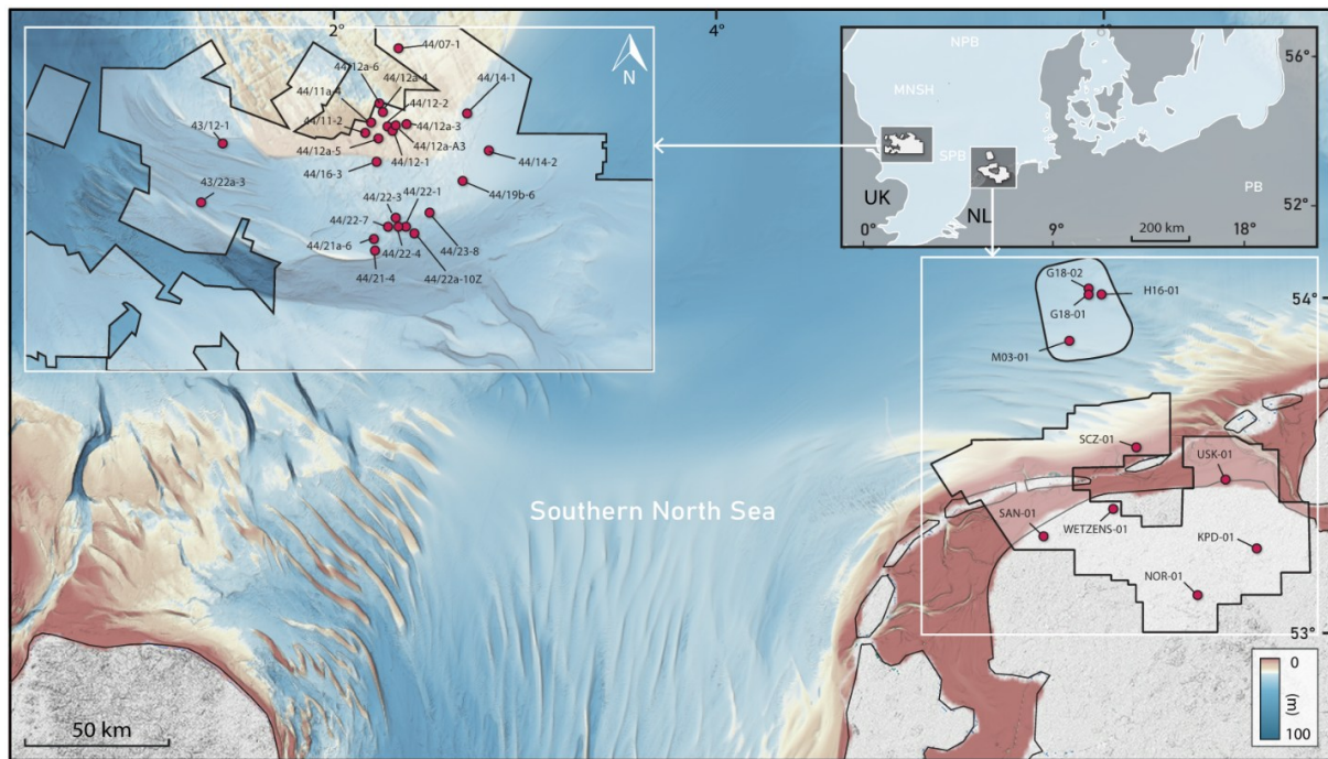
Fig. S1. Seismic and well database. Outlines of the 3-D surveys interpreted in the UK (left) and Dutch (right) sectors of the Southern North Sea, with the 34 calibration wells (circles). Inset: regional setting (MNSH, Mid North Sea High; NPB, Northern Permian Basin; SPB, Southern Permian Basin; PB, Polish Basin). Bathymetry in meters.
