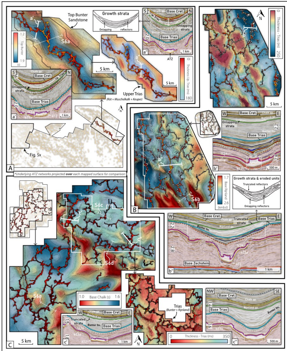
Figure 3. ATZs, post-salt synclines, and the stratal geometries above them. ATZ network (dark red) overlain on each map. (A) UK sector: Top Bunter time-structure and Upper Triassic isopach; a' and a'' show Lower Triassic onlap onto the flanks of ATZ-cored synclines (inset defines the geometry). (B) Dutch sector: Base Rijnland depth-structure and Triassic isopach; b' shows onlap, and b'' Triassic strata truncated beneath the Base Cretaceous over the flanking high. (C) Dutch sector: Base Chalk time-structure and Triassic isopach; c' and c'' show the same relationships. Enlarged sections, maps without the overlay, and regional sections in Figs. S4–S6.
