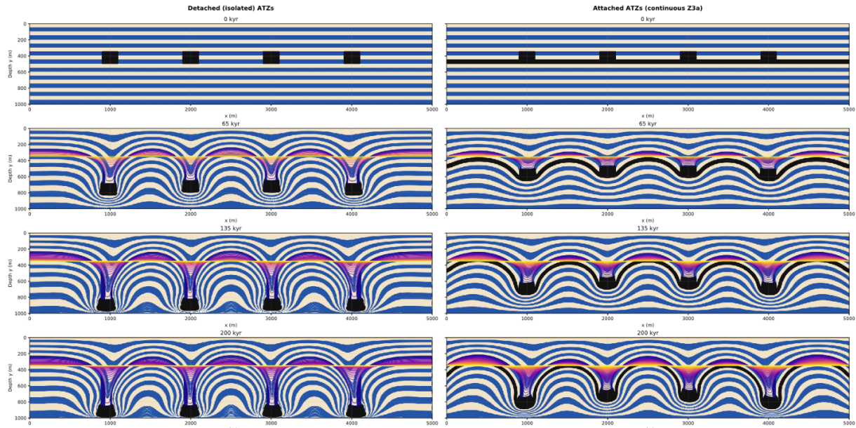
Fig. S9. Effect of stringer connectivity. Material evolution of the detached (left) and attached (right) experiments at 0, 65, 135 and 200 k.y.; anhydrite in black, halite with passive marker layers.
