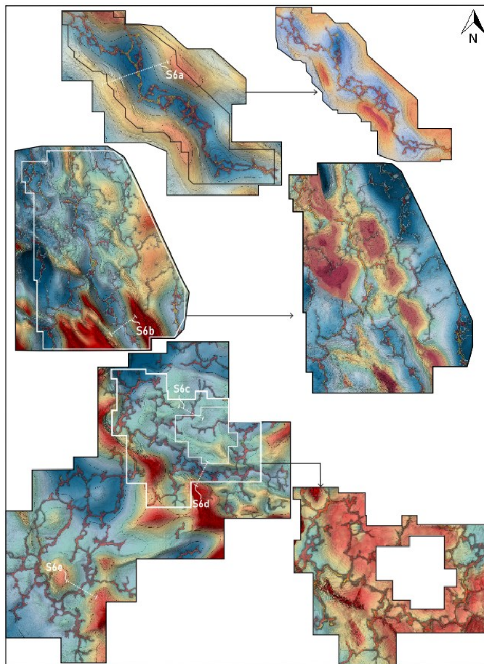
Fig. S5. Structure and thickness maps of Figure 3 with the ATZ network superimposed. Dashed lines locate the sections of Figure S6.
