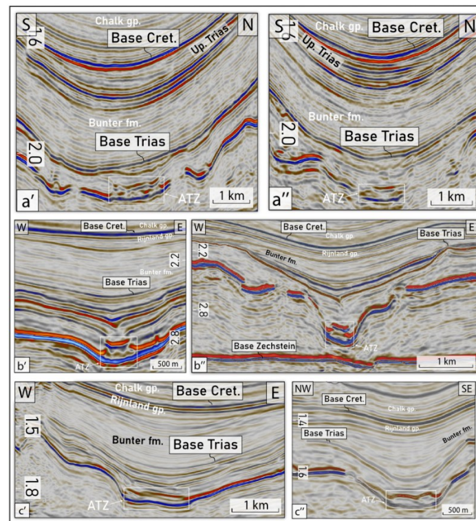
Fig. S4. Sections a'–c'' of Figure 3, enlarged. Lower Triassic strata onlap the flanks of ATZ-cored lows (a', a'', b') and are truncated beneath the Base Cretaceous over the intervening highs (b'', c', c'').
