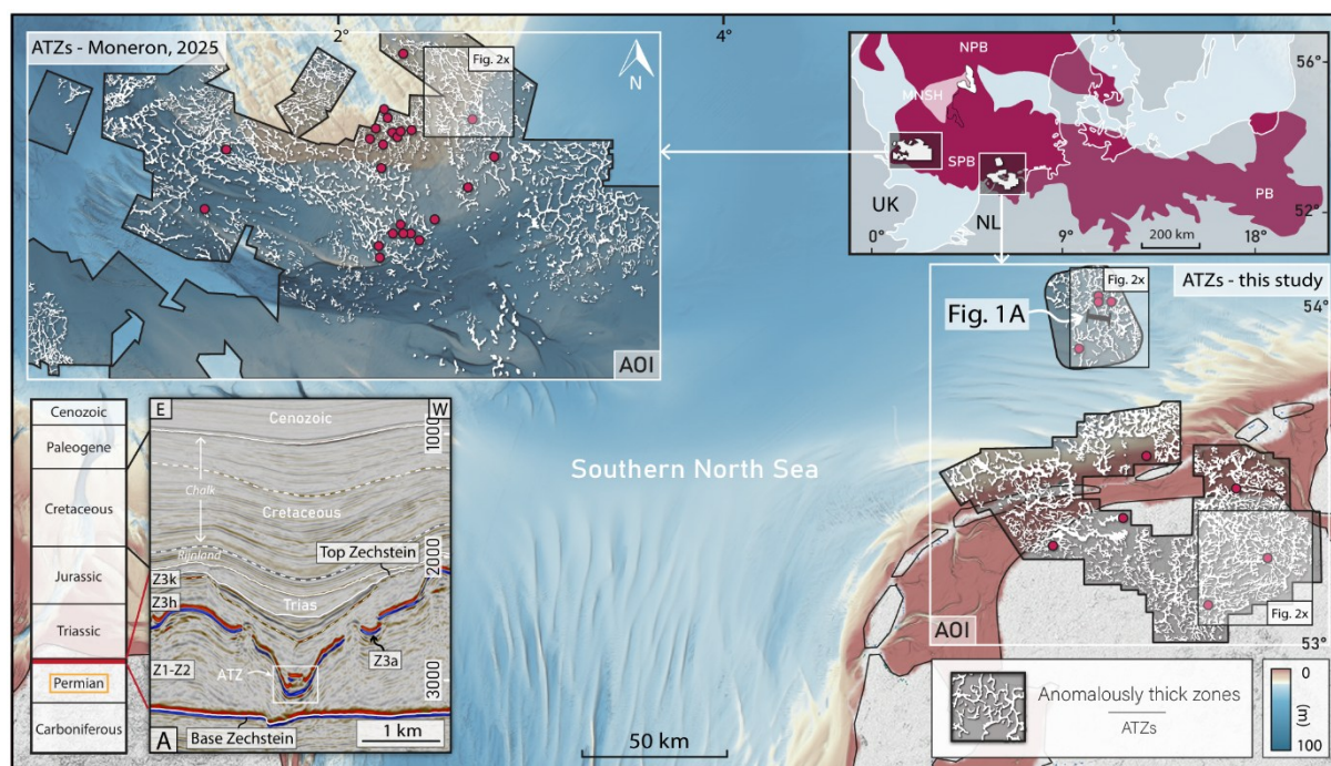
Figure 1. Setting and Z3 anhydrite (Z3a) network of anomalously thick zones (ATZs). Inset: Southern Permian Basin (SPB), adjacent basins (NPB, Northern Permian Basin; PB, Polish Basin; MNSH, Mid North Sea High) and Zechstein extent. Main panels: ATZ network (white) in the UK and Dutch areas of interest (AOIs), with 3-D seismic coverage (outlines) and wells (circles). (A) Seismic section through the UK AOI: an ATZ cores a syncline that persists into the Cenozoic. Full chronostratigraphy in the Supplemental Material (Fig. S2).
