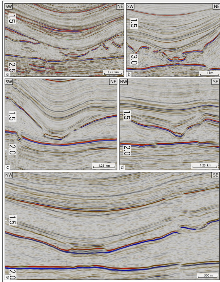
Fig. S6. Regional sections across the mapped synclines, located on Figure S5. The Base Zechstein (lowermost pick) is near-planar in all five, while the Top Zechstein and the overlying markers are folded into synclines beneath which the Zechstein thins, locally toward a weld (e). Vertical scale in seconds TWT except for b which is in km.
