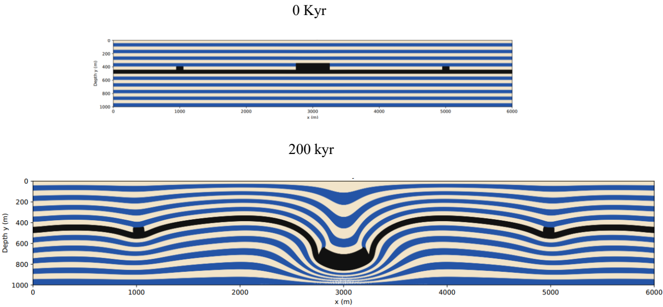
Fig. S14. Effect of anhydrite block geometry on sinking behavior and overlying synclinal depressions. The model contains three anhydrite blocks of different dimensions: left ( l = 150 m, h = 120 m), middle ( l = 250 m, h = 150 m), and right ( l = 100 m, h = 100 m), where l and h denote block length and height, respectively. The blocks exhibit different sinking rates, illustrating the influence of block geometry on gravitational sinking through halite.
