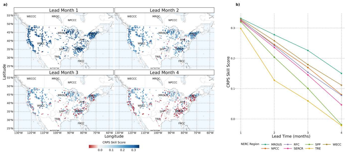
Figure 8. Hydropower-generation forecast skill measured by CRPSS at lead months 1–4. (a) Facility-level CRPSS at each lead and (b) regional median CRPSS by NERC region. Positive values indicate improvement over the climatological reference.
