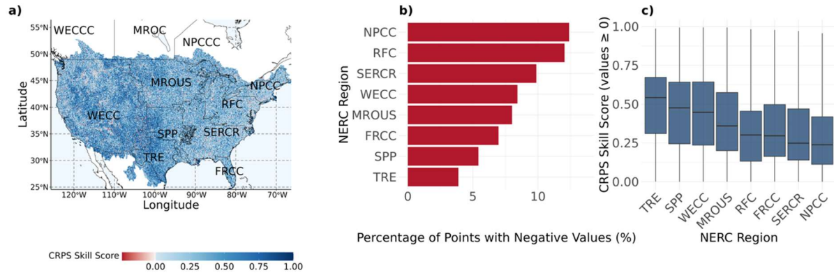
Figure 6. Spatial and statistical evaluation of CRPSS for the UMAL-LSTM across NERC regions. (a) Spatial CRPSS over the conterminous United States. (b) Fraction of grid cells with negative CRPSS by region. (c) Conditional distributions of positive CRPSS by region.
