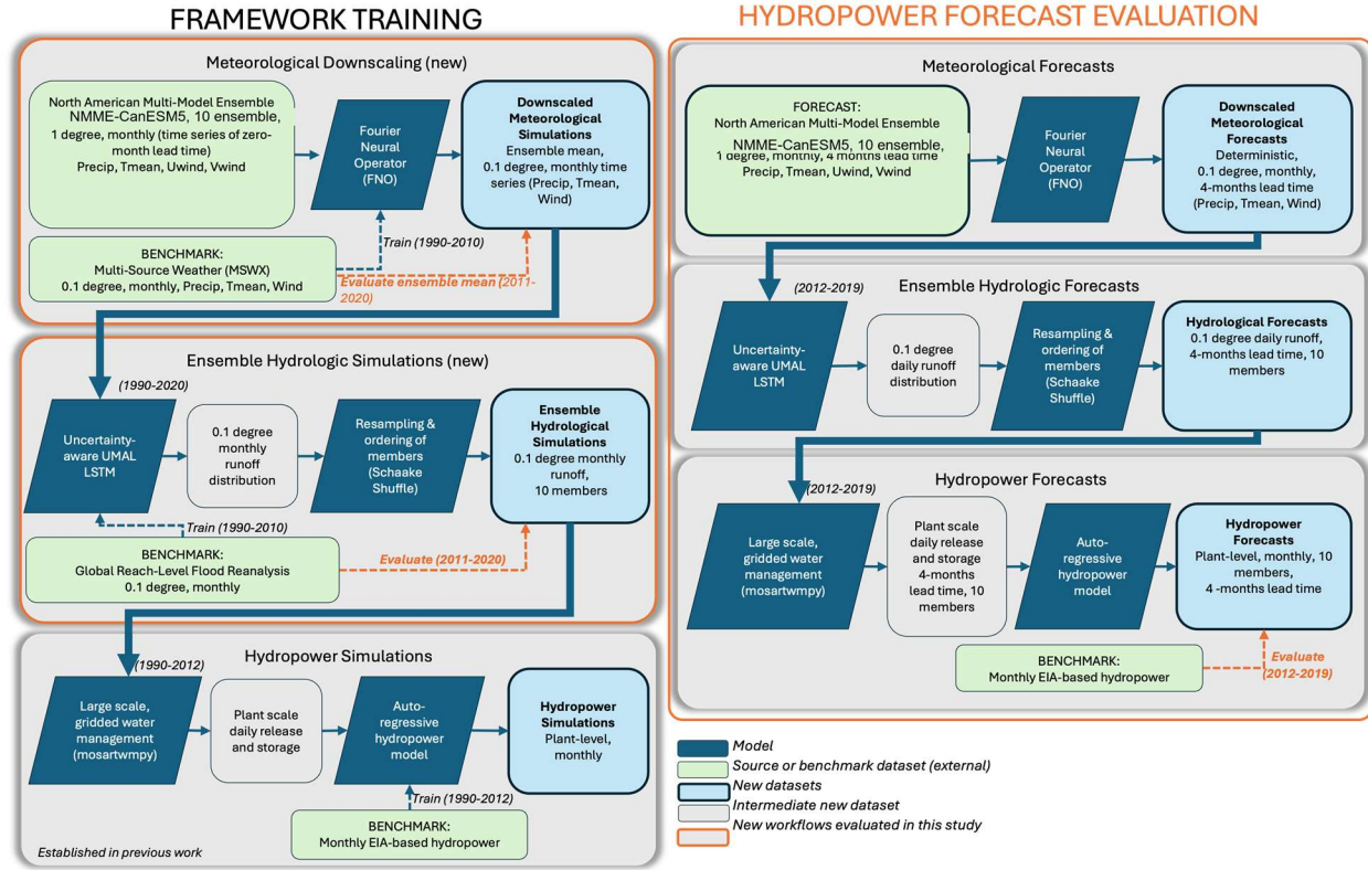
Figure 1: Hydropower Forecasting System Architecture. Left: training of the meteorological downscaling, hydrological, and hydropower components. Right: application in forecast mode.
