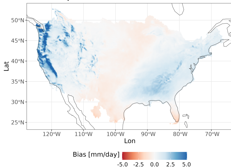
Precipitation [2011-2020] - Bias
