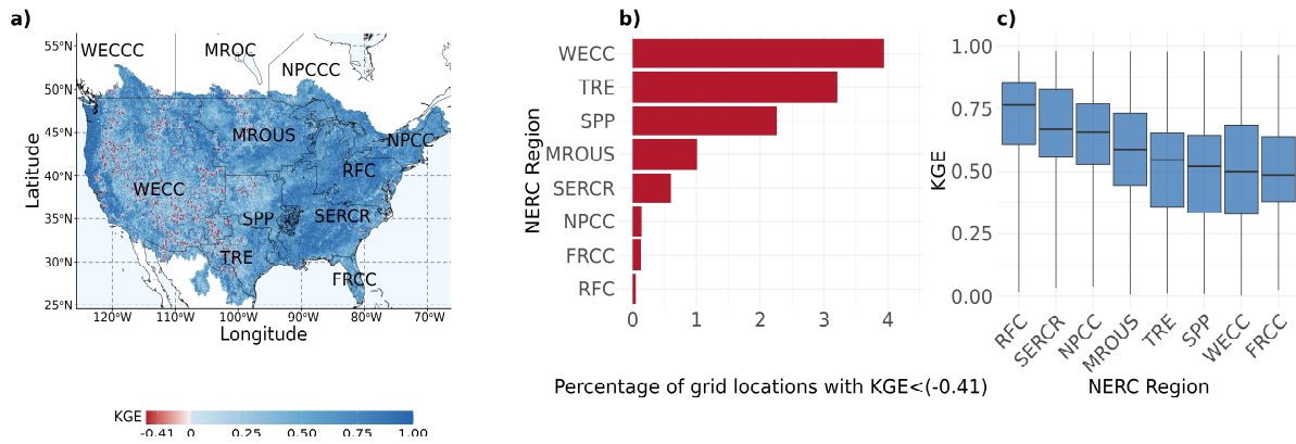
Figure 5. GRFR-based KGE evaluation of the UMAL-LSTM ensemble median across NERC regions. (a) Spatial KGE over the conterminous United States. (b) Fraction of all grid cells with KGE < −0.41 by region. (c) Regional KGE boxplot distributions by NERC region.
