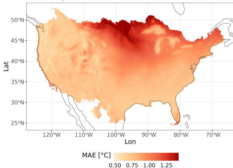
Temperature [2011-2020] - MAE
