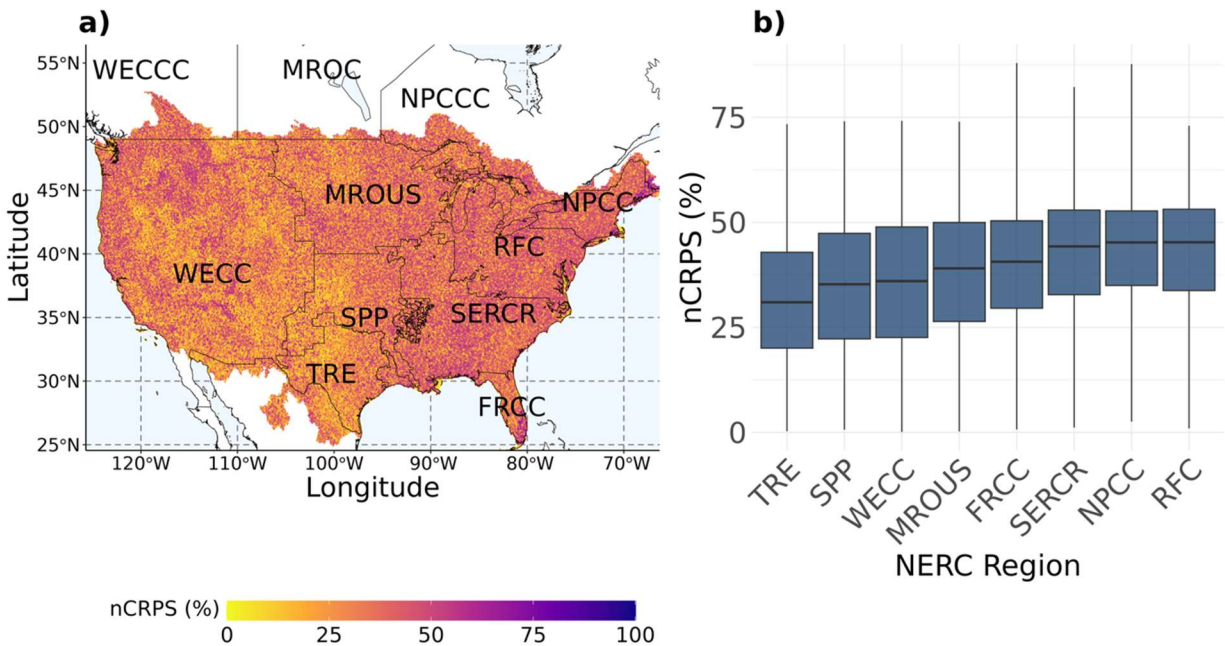
Figure 7. Spatial map and regional distributions of normalized CRPS (nCRPS) for the UMAL-LSTM. (a) Spatial nCRPS over the conterminous United States (lower is better). (b) Regional nCRPS distributions by NERC region.
