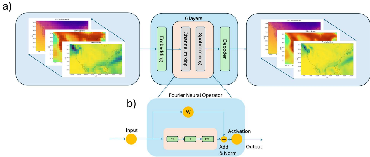
Figure 2: Fourier Neural Operator (FNO) for Meteorological Downscaling. a) End-to-end downscaling framework showing coarse-resolution inputs (left), FNO architecture with embedding, six-layer network of channel and spatial mixing, and decoder (center), and resulting
