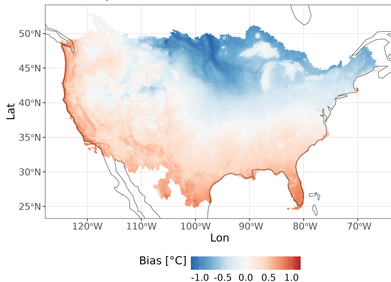
Temperature [2011-2020] - Bias
