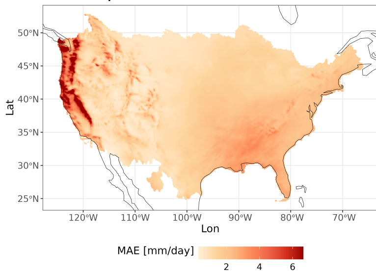
Precipitation [2011-2020] - MAE
