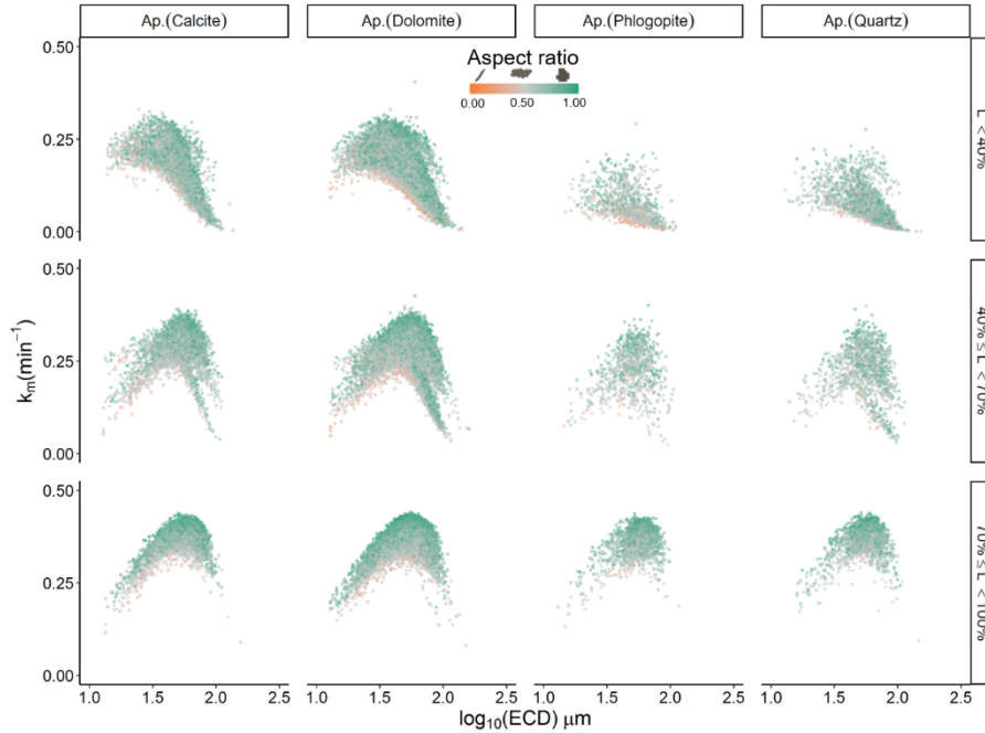
Figure 7: Distribution of k_m among particles containing apatite, according to their size (enclosed circle diameter - ECD), liberation degree (L), and aspect ratio. Particles are further grouped according to their main association, as indicated in parentheses.
