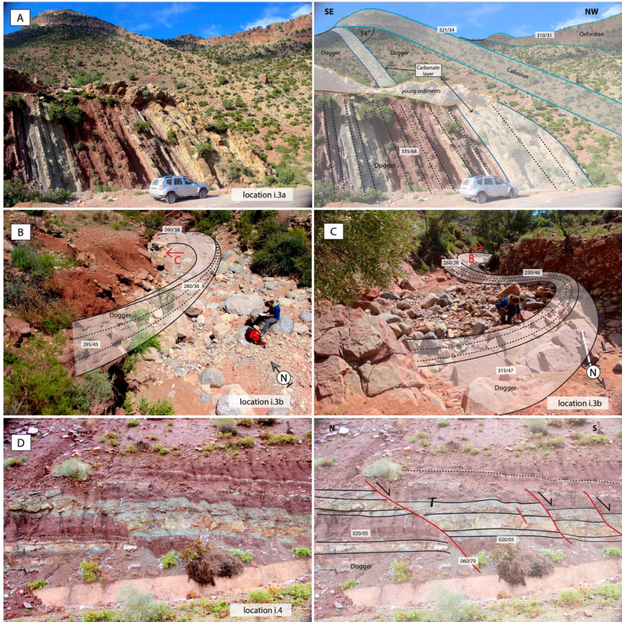
Figure B2 | Dogger showing an angular unconformity, folding, and normal faulting.
