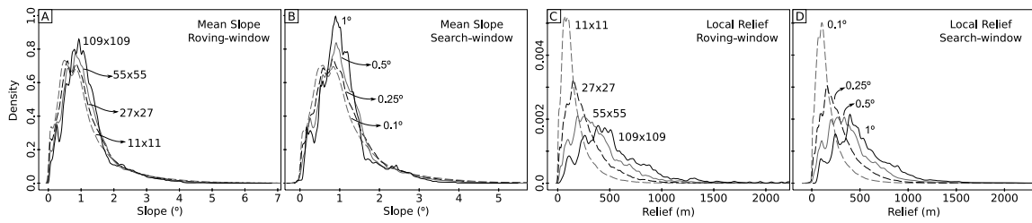
Figure 5. Density plots of morphometric maps. A) Mean slope, roving-window; B) Mean slope, search-window; C) Local relief, roving-window; D) Local relief, search-window.
