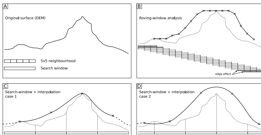
Figure 3. Comparison between roving-window and search-window (maximum value). A) Original surface (elevation); B) Roving-window (5x5); C) Search-window – case 1; D) Search-window – case 2.
