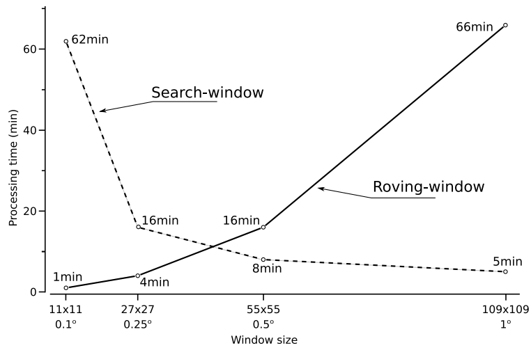
Figure 4. Processing time for mean slope operation, using roving-windows and search-windows, according to window size.
