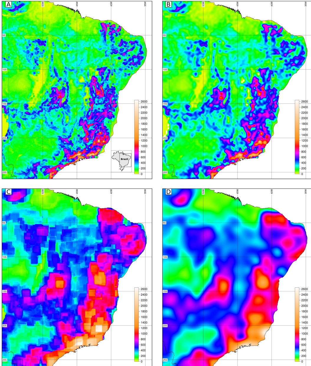
Figure 6. Maps of local relief. A) Roving-window, 27x27 cells; B) Search-window, 0.25°; C) Roving-window, 109x109 cells; D) Search-window, 1°.
