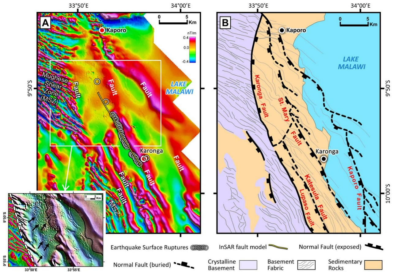
Figure: Filtered aeromagnetic data (Fig A) reveal buried seismogenic faults along the actively-deforming hinge zone of a half-graben rift. Further enhancement of the data shows that basement fabric aligns with the segments of the faults
