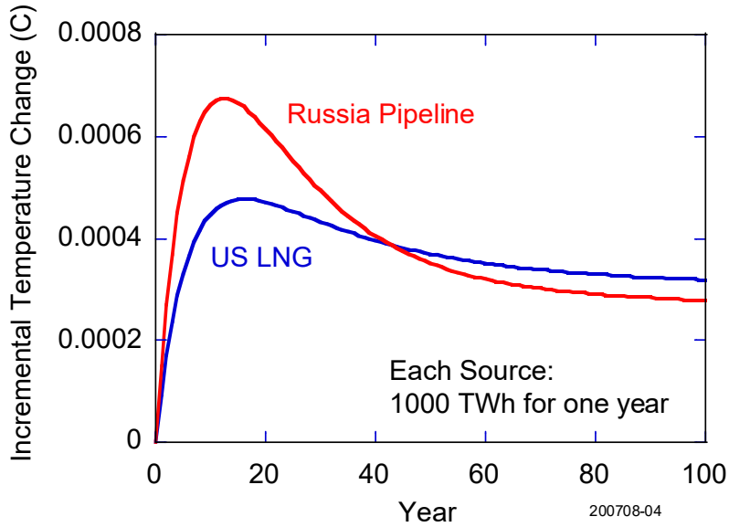
Figure 21c. Actual greenhouse gas impacts of gas-fired electric power plants fueled by gas imported to Europe via pipeline from Russia (red) and via liquefied natural gas imported from the United States (blue) following a single year of emissions. The GHG footprint of electric power generation, transmission, and distribution are included in the calculations.
