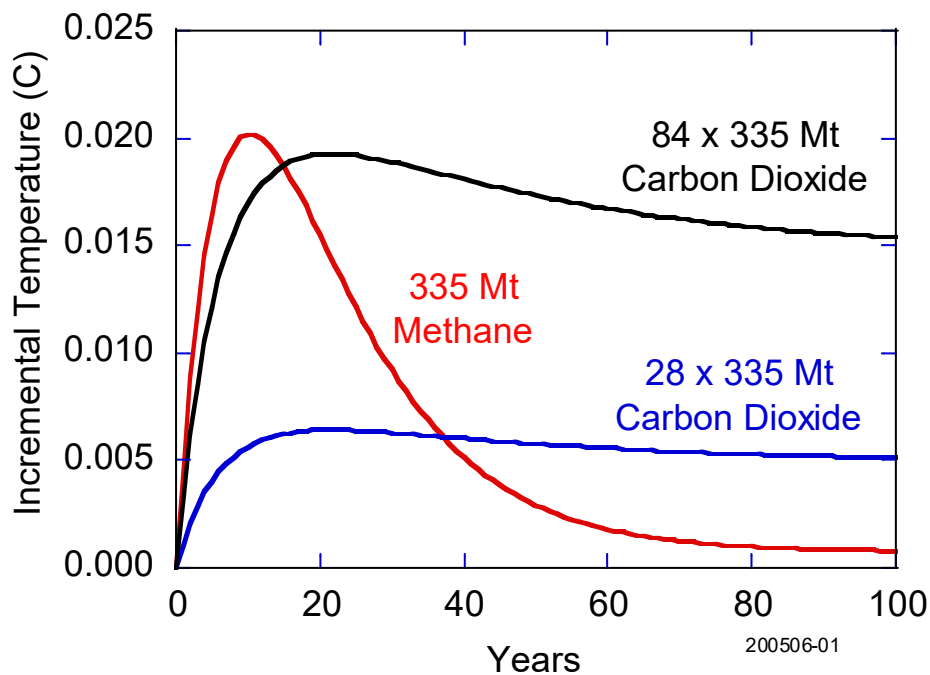
Figure 11. Temperature trajectory of a 335 Mt pulse of methane at t = 0 (red) compared to temperature trajectories for corresponding CO_2\text{-eq} pulses for GWP_{20} = 84 (black) and GWP_{100} = 28 (blue).
