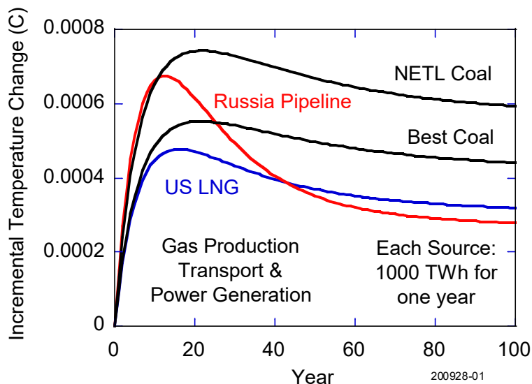
Figure 23. Greenhouse gas impacts of single-year emissions for various options for electric power generation in the European context.
