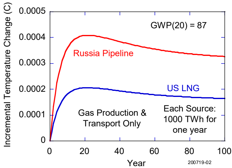
Figure 22b. Global warming potential calculation (GWP 20 = 87) of the greenhouse gas impacts of gas imported to Europe via pipeline from Russia (red) and via liquefied natural gas imported from the United States (blue) following a single year of emissions. The GHG footprint of electric power generation, transmission, and distribution are not included in the calculations.
