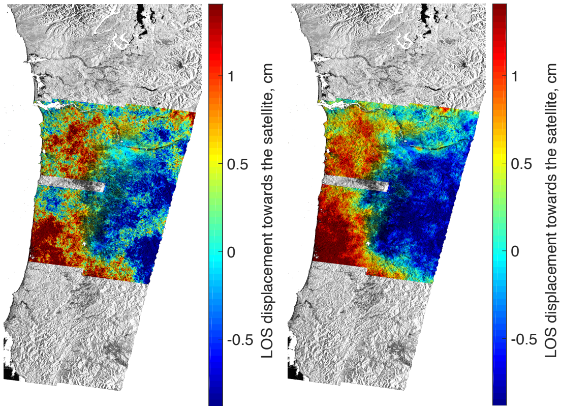
Fig. 5. Results from (left) non-repeating and (right) repeating stacking over the February 2016 slow slip event in the Cascadia region. The result from repeating stacking suffers from less decorrelation noise than the result from non-repeating stacking. Areas with less coverage than 20 acquisitions are masked. Phase measurements are converted to radar line-of-sight (LOS) measurements.
