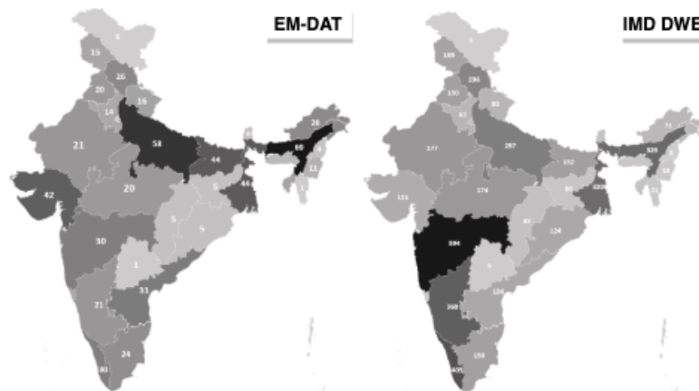
Figure 4 shows the spatial distribution of the number of flooding events in IFI from IMD DWE and EM-DAT.
