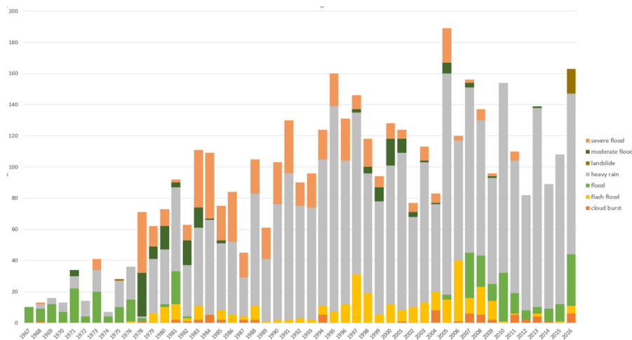
Figure 7. Temporal evolution of causative factors according to IMD DWE
