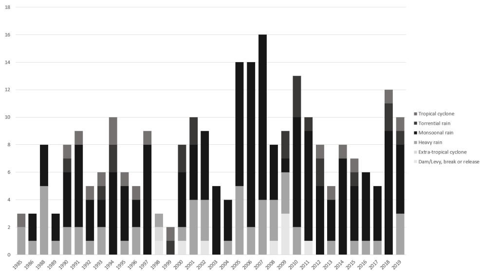
Figure 6. Temporal evolution of causative factors according to DFO
