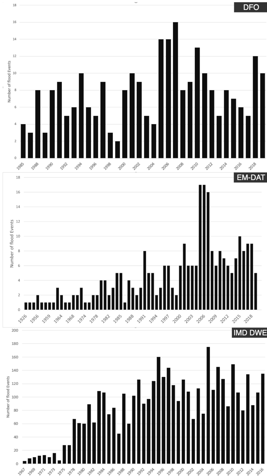
Figure 2: Temporal evolution of the number of floods at national scale
