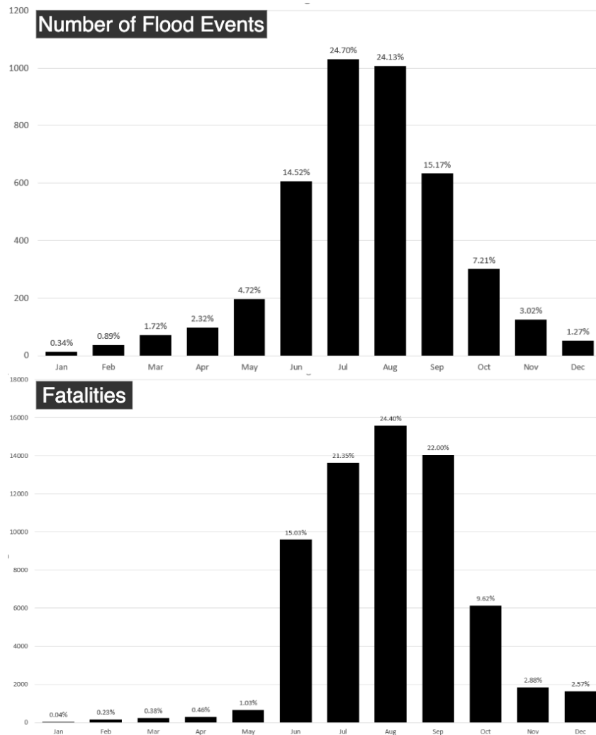
Figure 8: Monthly variation of the number of flooding events and the fatalities according the IMD DWE
