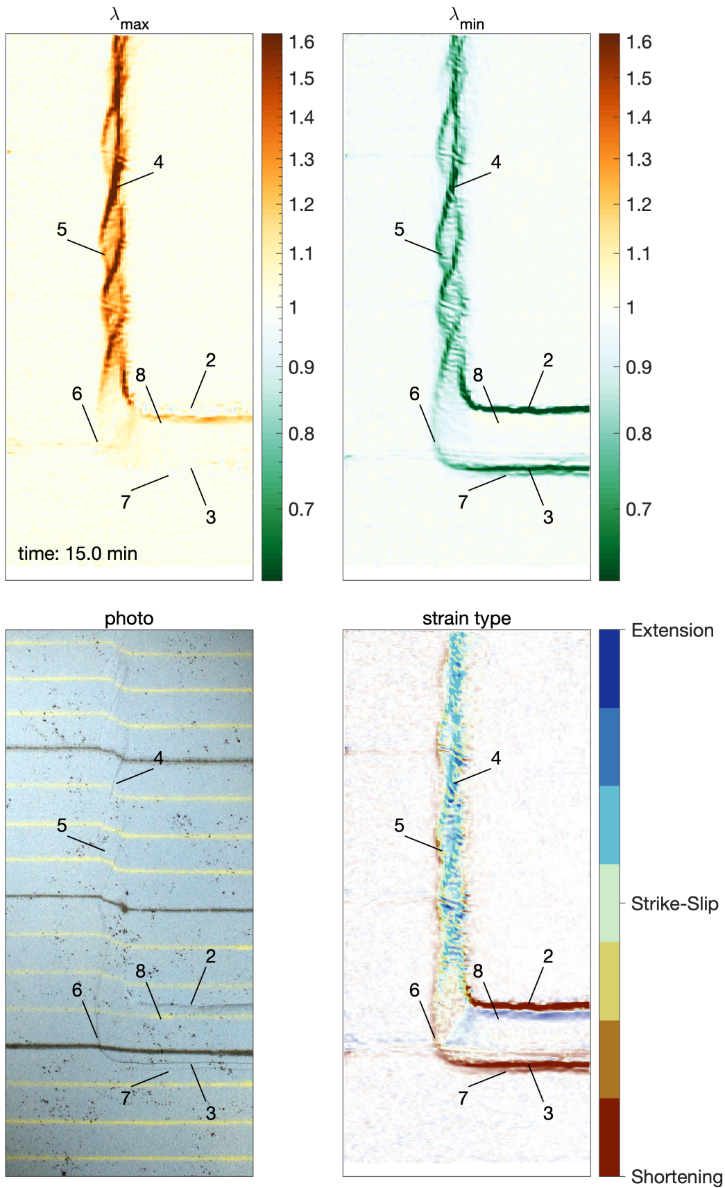
Figure 13: Principal stretches \lambda_{max} , \lambda_{min} ( \lambda = 1 represents no length change) and strain type \Phi at 15 minutes of model evolution: shortening (red), strike-slip (green) and extension (blue), with intermediate, oblique deformation at intermediate colors. Numbers indicate: (2) basal thrust; (3) first back-thrust; (4) Riedel R-shear; (5) Riedel P-shear; (6) fault connecting basal-thrust and strike-slip zone; (7) new back-thrust; (8) zone of extensional surface deformation.
